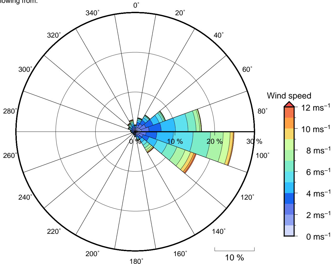
Figure 11 Annual wind rose for Pago Pago. Note that directions are where the wind is coming from .
