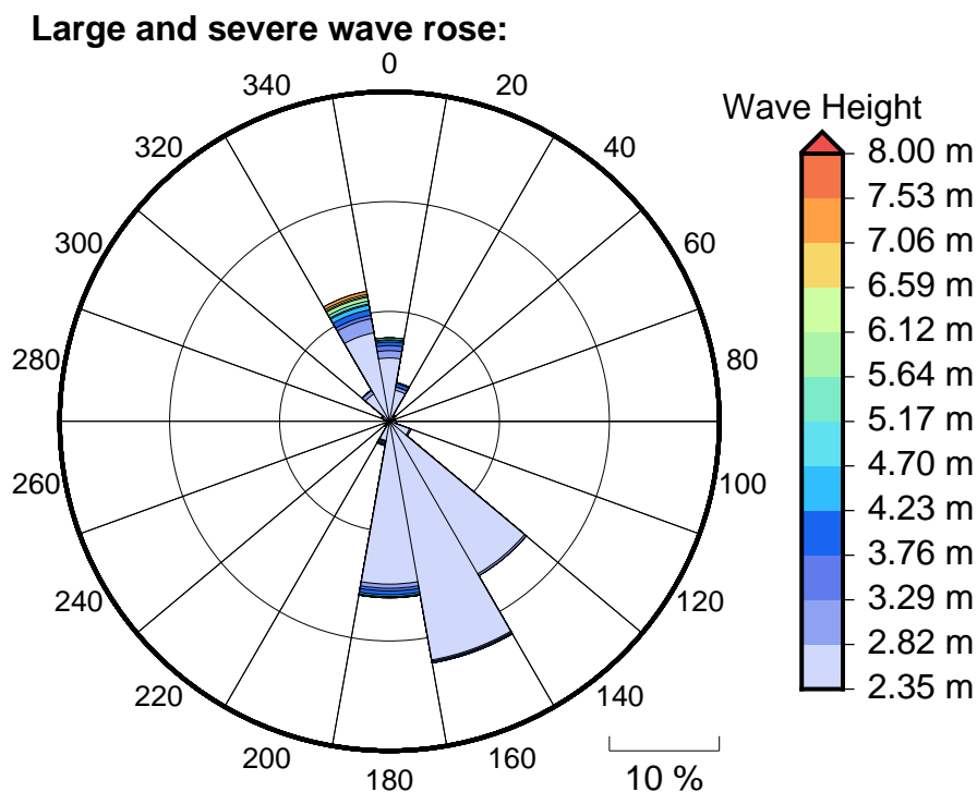
Figure 6 Large, severe and extreme wave roses for Pago Pago
