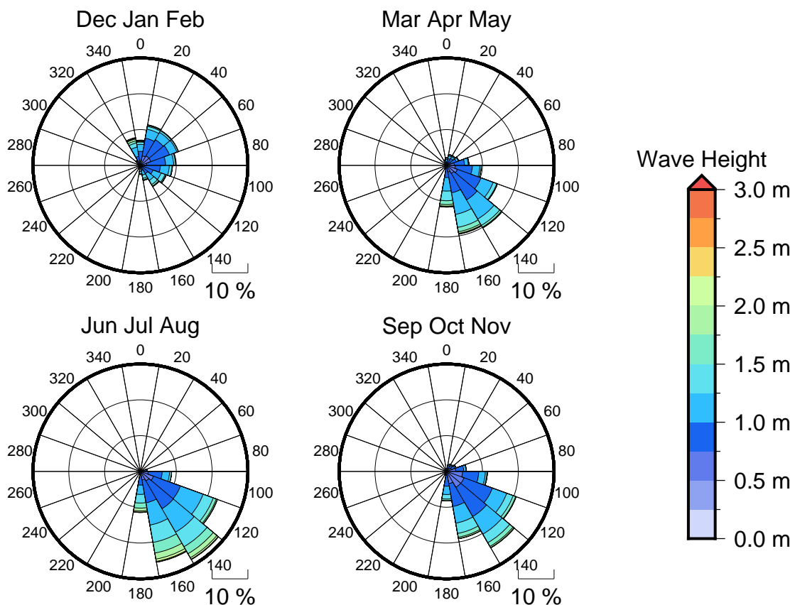
Figure 3 Seasonal wave roses for Pago Pago
