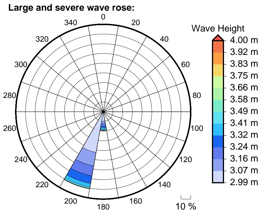
Figure 6 Large, severe and extreme wave roses for Avaavaroa passage
