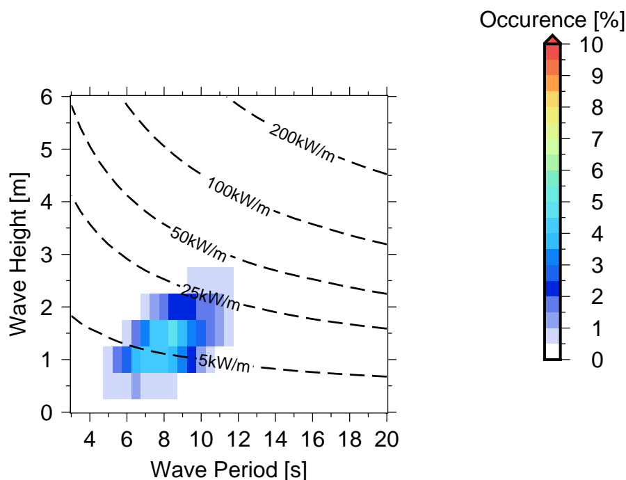
Figure 10 Occurrences of sea states in Avaavaroa passage .
