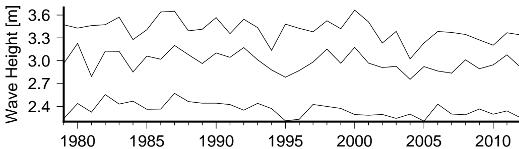
Figure 8 Annual variation in large waves (90th percentile)(lower curve), severe waves (99th percentile) (middle curve) and the largest wave(upper curve) in Avaavaroa passage.
