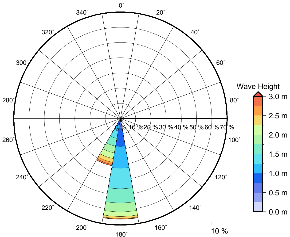
Figure 2 Annual wave rose for Avaavaroa passage. Note that direction are where the wave are coming from.
