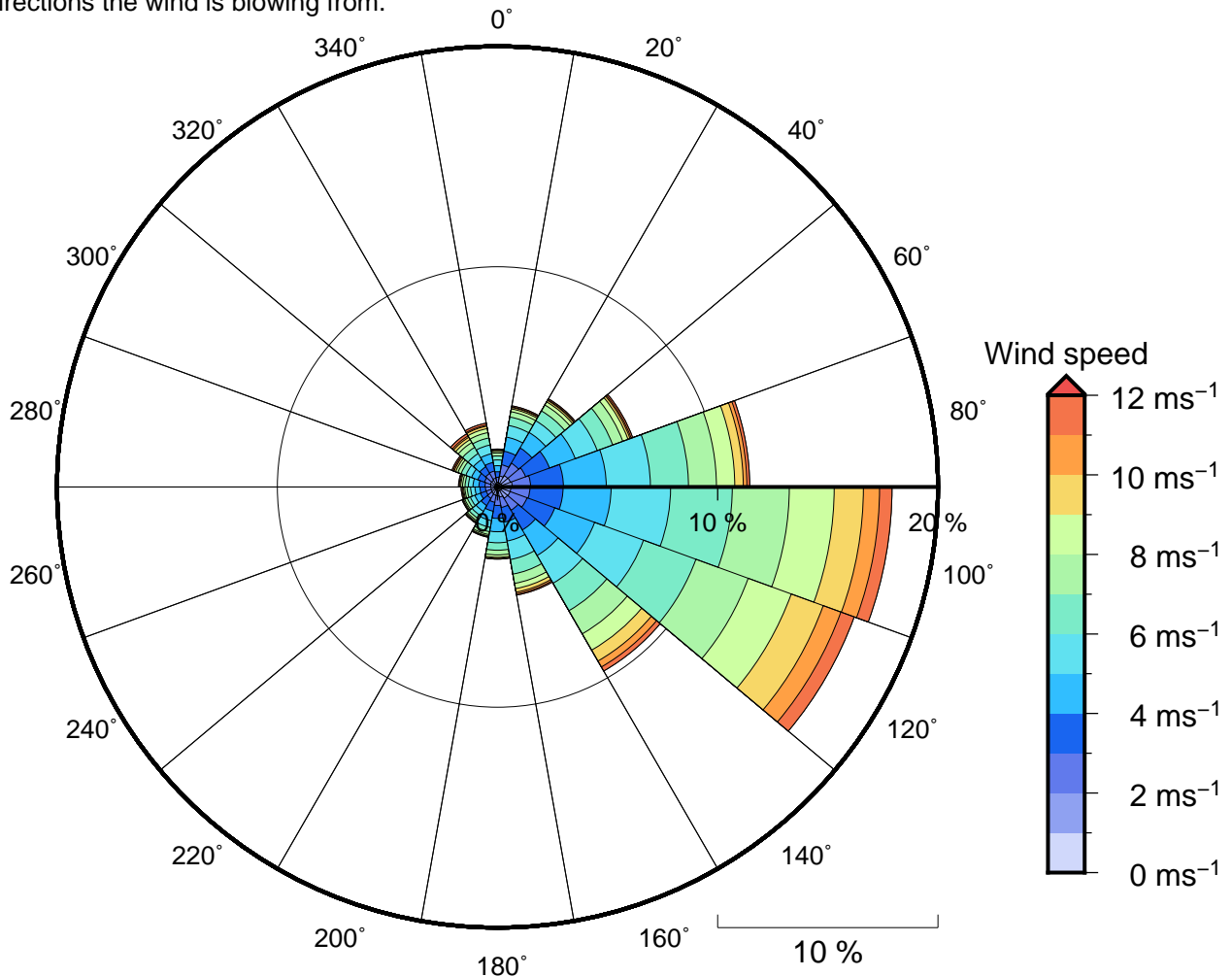
Figure 11 Annual wind rose for Avaavaroa passage. Note that directions are where the wind is coming from.
