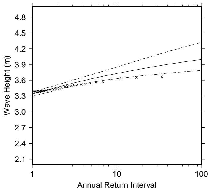
Figure 9 Extreme wave distribution for Avaavaroa passage. The crosses represents the wave events that occurred since 1979. The plain line is the statistical distribution that best fit the past wave events. The dotted line show the upper and lower high confidence of the fit, there is a 95% chance that the fitted distribution lie between the two dashed lines.
