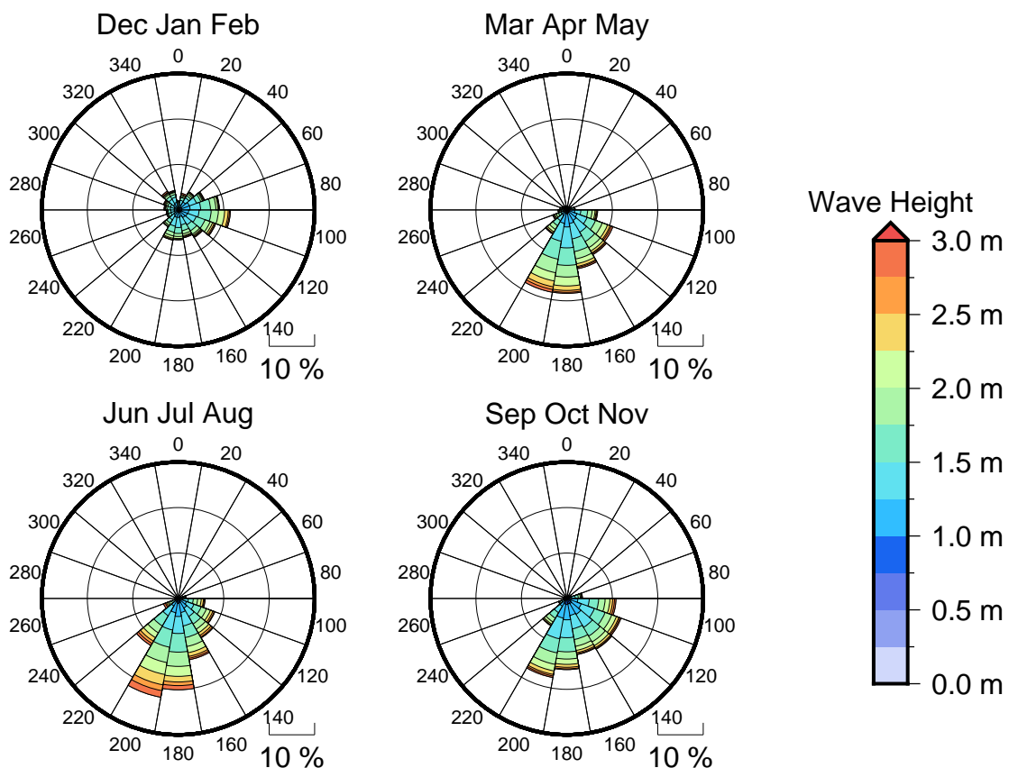
Figure 3 Seasonal wave roses for Avatiu
