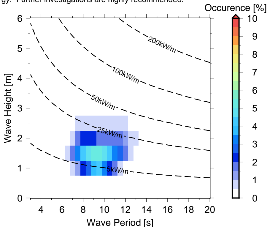
Figure 10 Occurrences of sea states in Avatiu .
