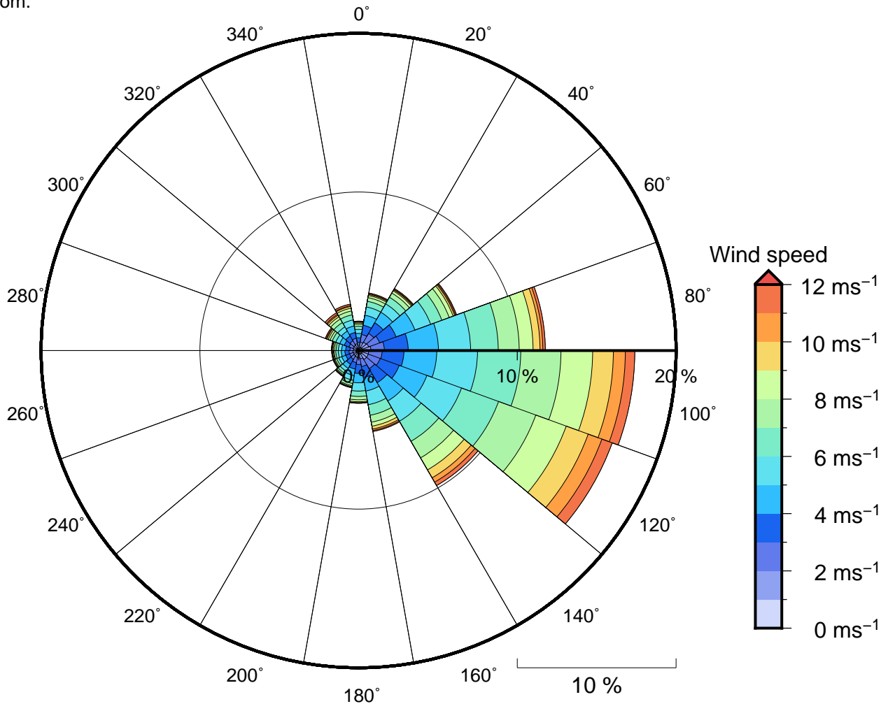
Figure 11 Annual wind rose for Avatiu. Note that directions are where the wind is coming from.
