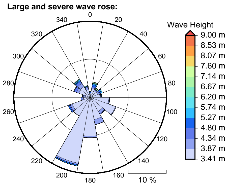
Figure 6 Large, severe and extreme wave roses for Avatiu
