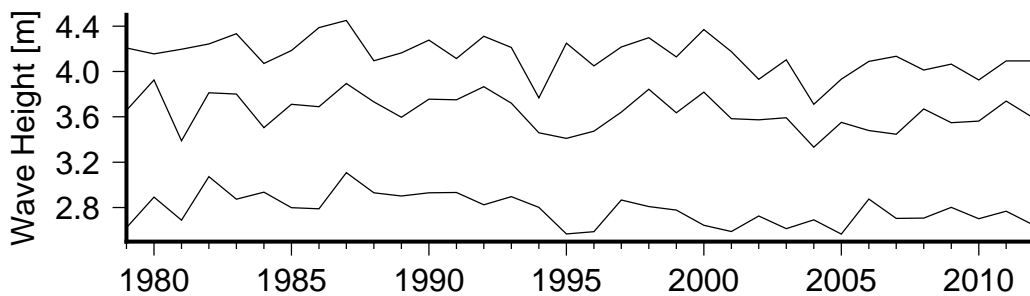
Figure 8 Annual variation in large waves (90th percentile)(lower curve), severe waves (99th percentile) (middle curve) and the largest wave(upper curve) in Avatiu passage.
