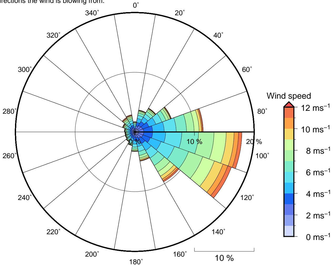
Figure 11 Annual wind rose for Avatiu passage. Note that directions are where the wind is coming from.
