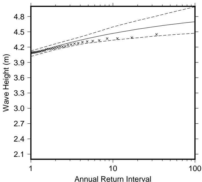
Figure 9 Extreme wave distribution for Avatiu passage. The crosses represents the wave events that occurred since 1979. The plain line is the statistical distribution that best fit the past wave events. The dotted line show the upper and lower high confidence of the fit, there is a 95% chance that the fitted distribution lie between the two dashed lines.
