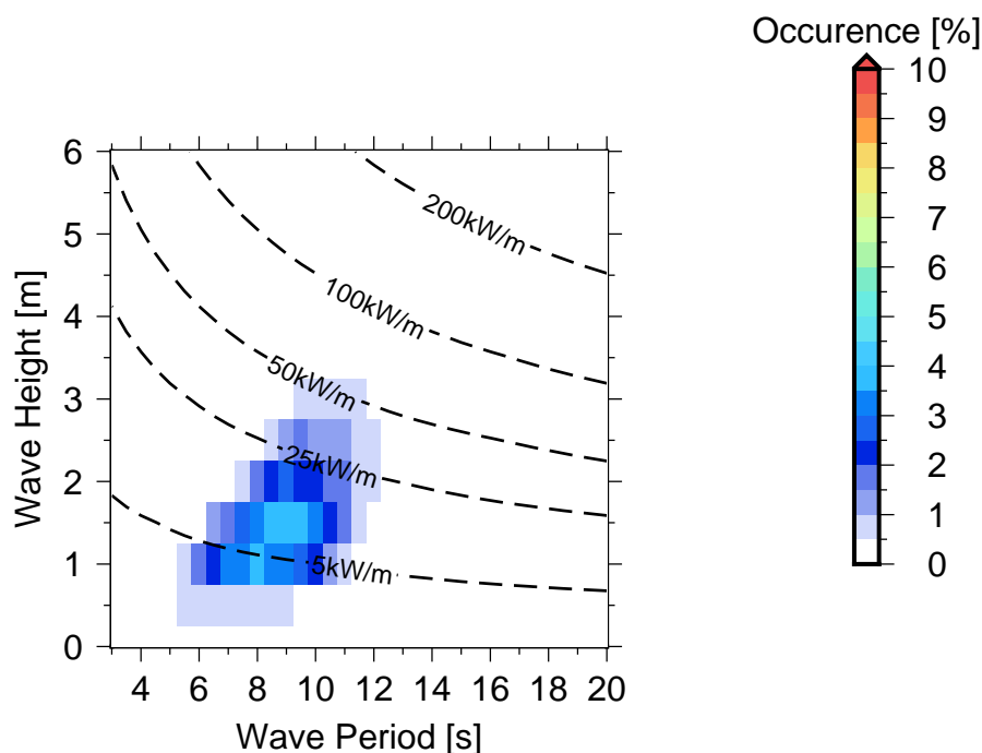
Figure 10 Occurrences of sea states in Avatiu passage .
