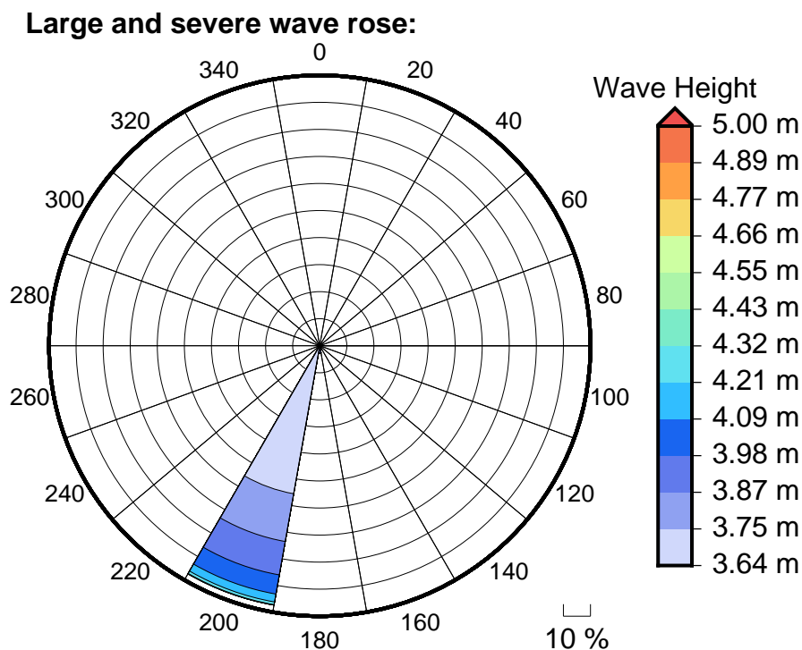
Figure 6 Large, severe and extreme wave roses for Avatiu passage
