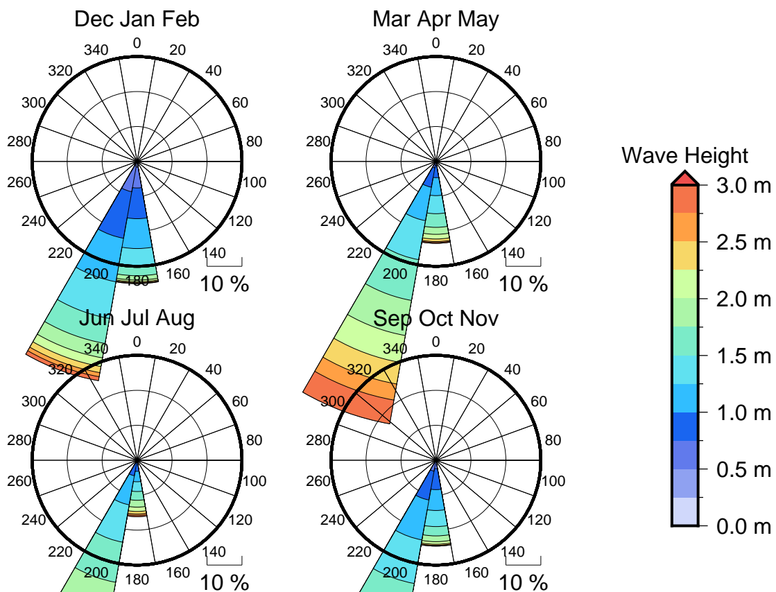
Figure 3 Seasonal wave roses for Avatiu passage
