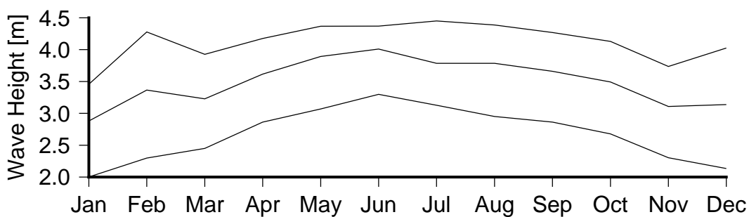
Figure 7 Monthly variation in large waves (90th percentile)(lower curve), severe waves (99th percentile) (middle curve) and the largest wave(upper curve) in Avatiu passage.
