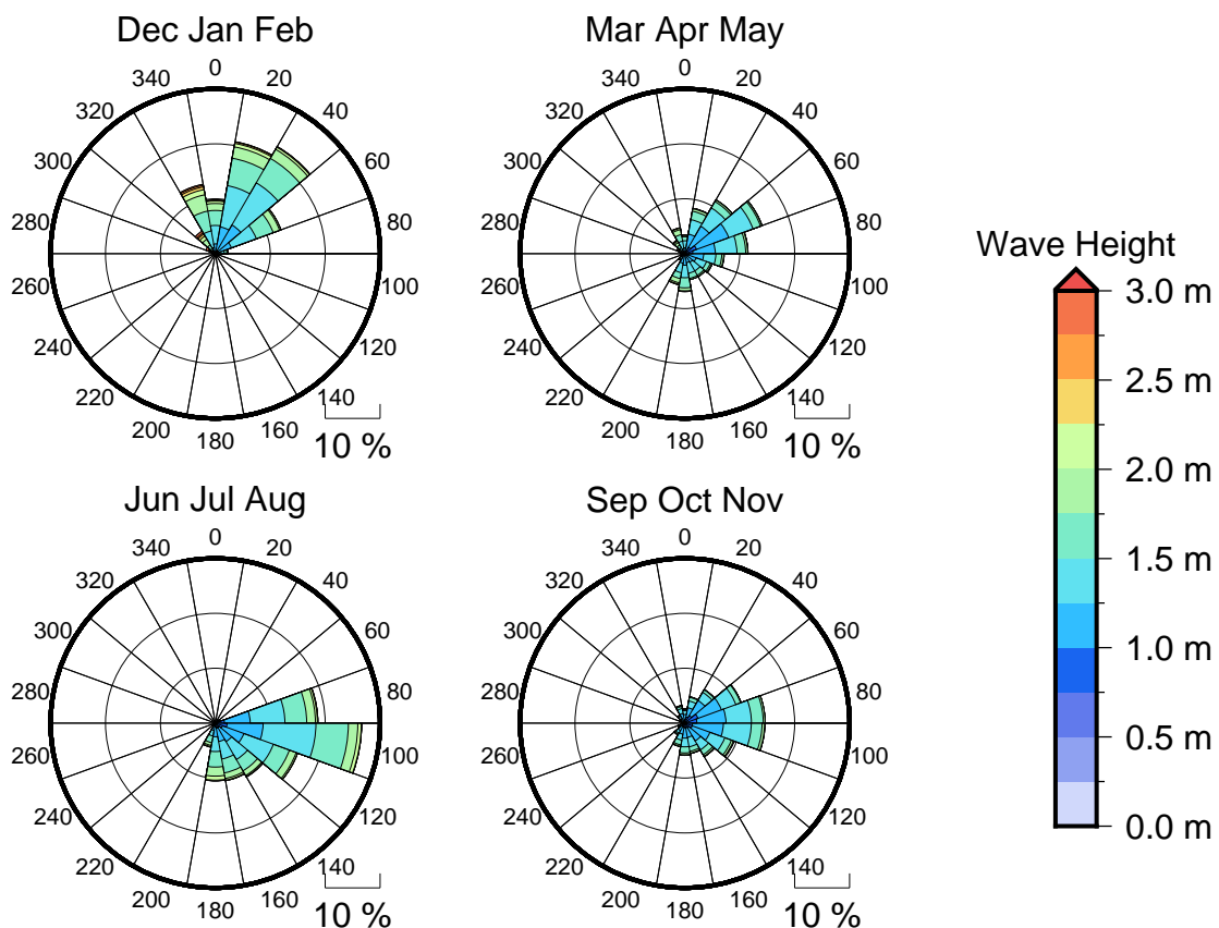
Figure 3 Seasonal wave roses for Penrhyn
