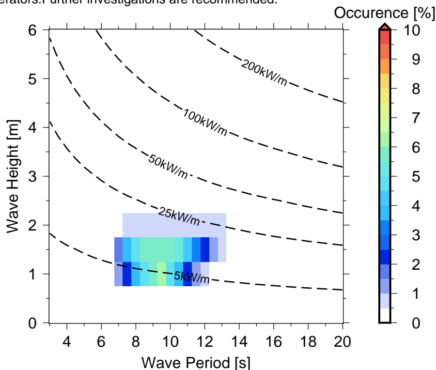
Figure 10 Occurrences of sea states in Penrhyn .
