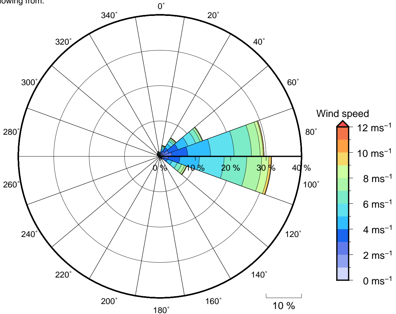
Figure 11 Annual wind rose for Penrhyn. Note that directions are where the wind is coming from.
