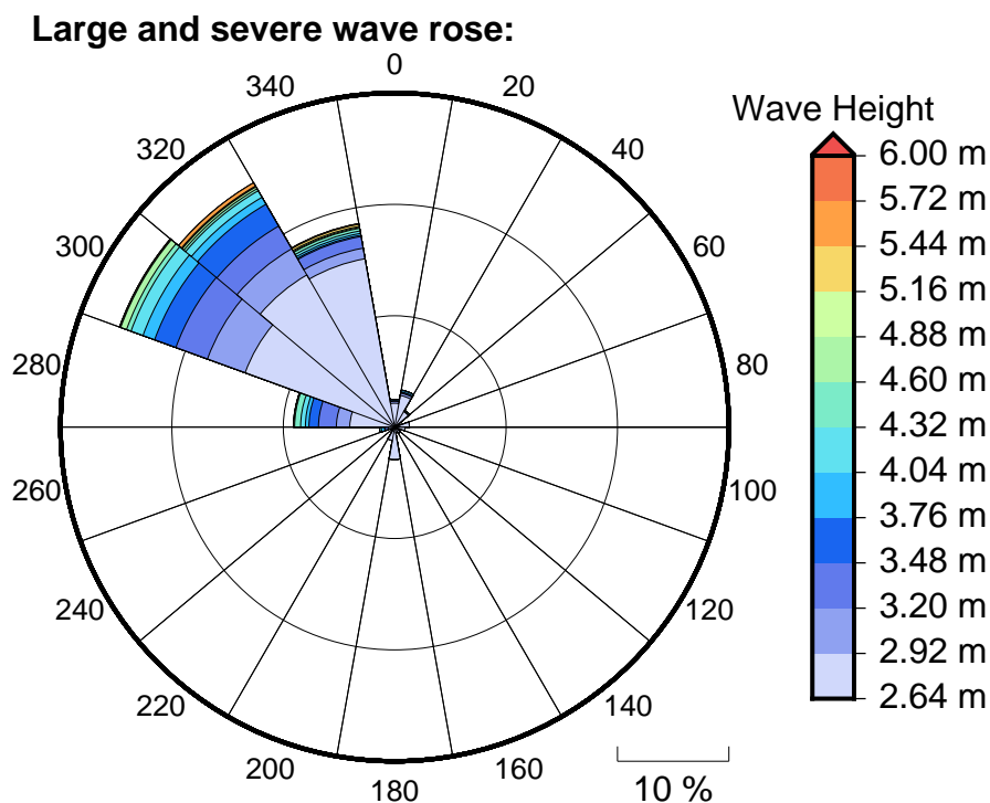
Figure 6 Large, severe and extreme wave roses for Penrhyn
