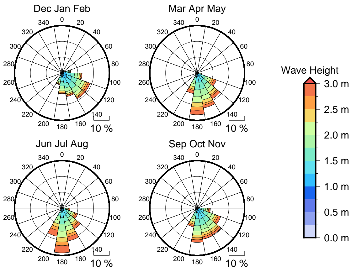
Figure 3 Seasonal wave roses for Wave Bouy location 2
