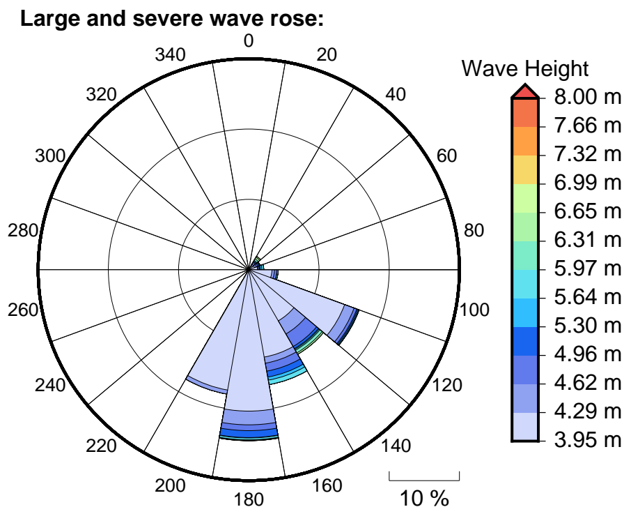
Figure 6 Large, severe and extreme wave roses for Wave Bouy location 2
