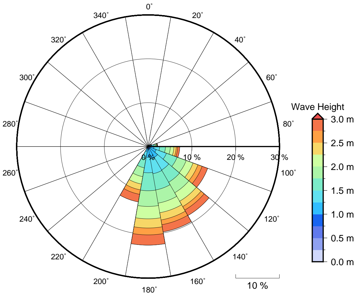
Figure 2 Annual wave rose for Wave Bouy location 2. Note that direction are where the wave are coming from.
