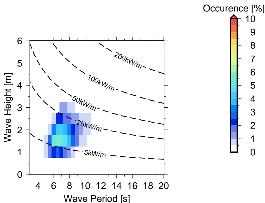
Figure 10 Occurences of sea states in Wave Bouy location 2 .
