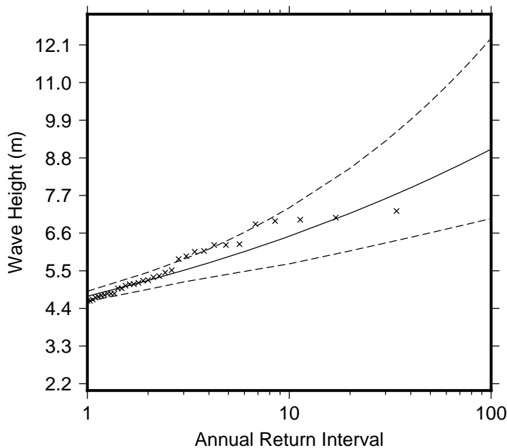
Figure 9 Extreme wave distribution for Wave Bouy location 2. The crosses represents the wave events that occurred since 1979. The plain line is the statistical distribution that best fit the past wave events. The dotted line show the upper and lower high confidence of the fit, there is a 95% chance that the fitted distribution lie between the two dashed lines.
