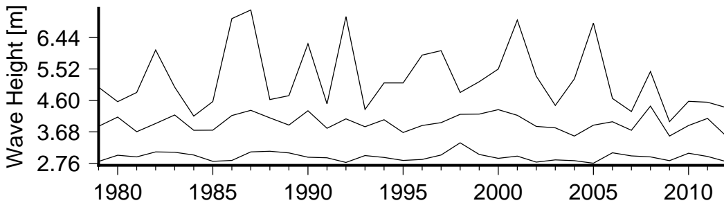
Figure 8 Annual variation in large waves (90th percentile)(lower curve), severe waves (99th percentile) (middle curve) and the largest wave(upper curve) in Wave Bouy location 2.
