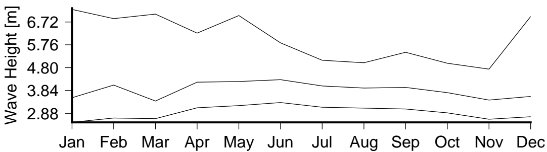
Figure 7 Monthly variation in large waves (90th percentile)(lower curve), severe waves (99th percentile) (middle curve) and the largest wave(upper curve) in Wave Bouy location 2.
