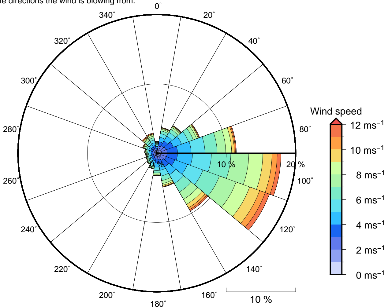
Figure 11 Annual wind rose for Wave Bouy location 2. Note that directions are where the wind is coming from.
