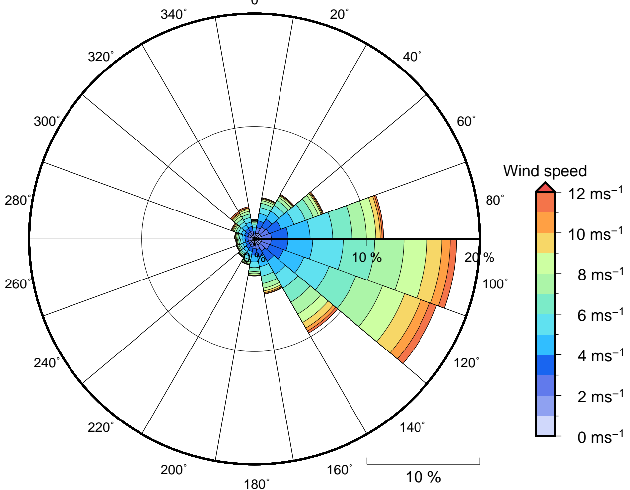
Figure 11 Annual wind rose for Rarotongan wave energy hotspot. Note that directions are where the wind is coming from .
