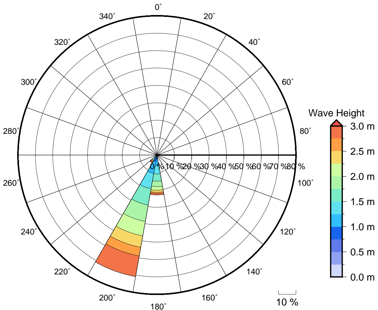
Figure 2 Annual wave rose for Rarotongan wave energy hotspot. Note that direction are where the wave are coming from .
