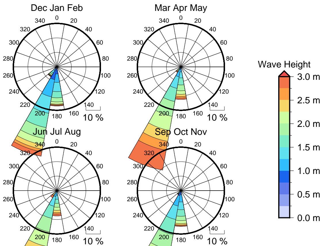
Figure 3 Seasonal wave roses for Rarotongan wave energy hotspot
