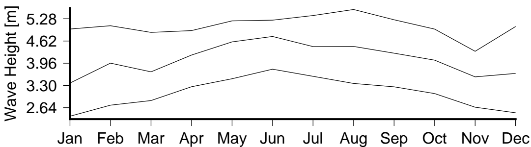
Figure 7 Monthly variation in large waves (90th percentile)(lower curve), severe waves (99th percentile) (middle curve) and the largest wave(upper curve) in Rarotongan wave energy hotspot.
