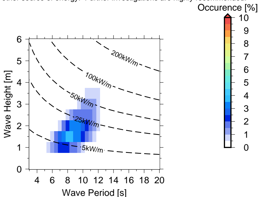
Figure 10 Occurrences of sea states in Rarotongan wave energy hotspot .
