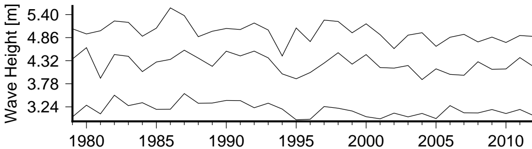
Figure 8 Annual variation in large waves (90th percentile)(lower curve), severe waves (99th percentile) (middle curve) and the largest wave(upper curve) in Rarotongan wave energy hotspot.
