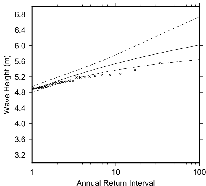
Figure 9 Extreme wave distribution for Rarotongan wave energy hotspot. The crosses represents the wave events that occurred since 1979. The plain line is the statistical distribution that best fit the past wave events. The dotted line show the upper and lower high confidence of the fit, there is a 95% chance that the fitted distribution lie between the two dashed lines.
