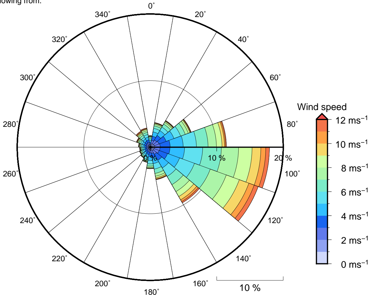
Figure 11 Annual wind rose for Tupapa. Note that directions are where the wind is coming from.
