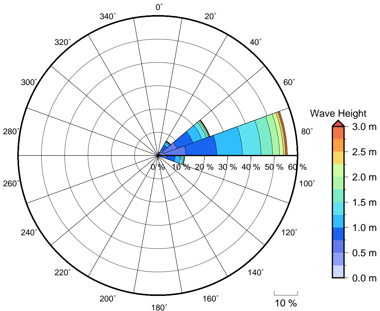
Figure 2 Annual wave rose for Tupapa. Note that direction are where the wave are coming from.
