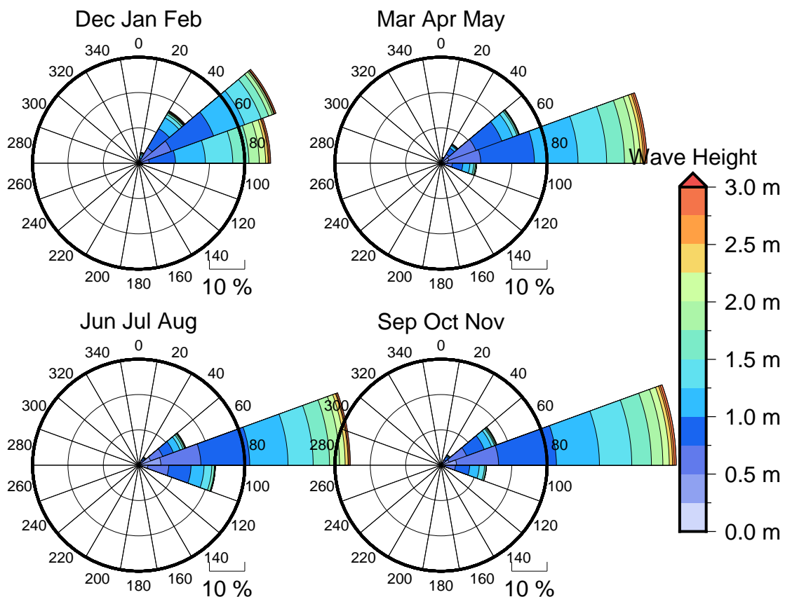
Figure 3 Seasonal wave roses for Tupapa
