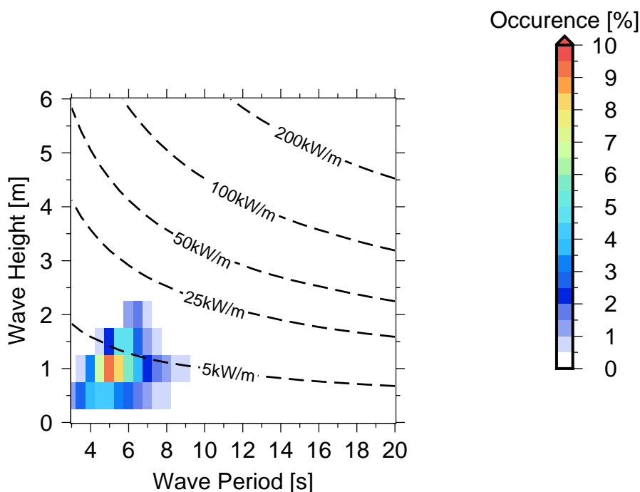
Figure 10 Occurrences of sea states in Tupapa .
