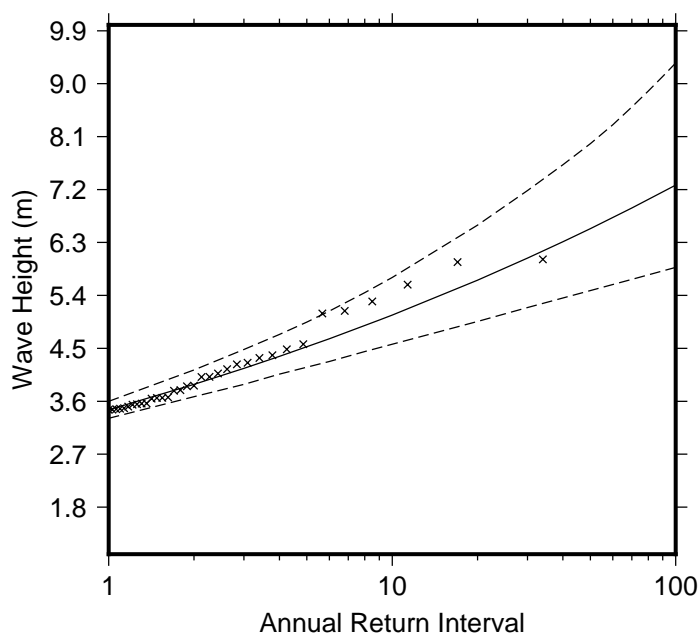
Figure 9 Extreme wave distribution for Tupapa. The crosses represents the wave events that occurred since 1979. The plain line is the statistical distribution that best fit the past wave events. The dotted line show the upper and lower high confidence of the fit, there is a 95% chance that the fitted distribution lie between the two dashed lines.
