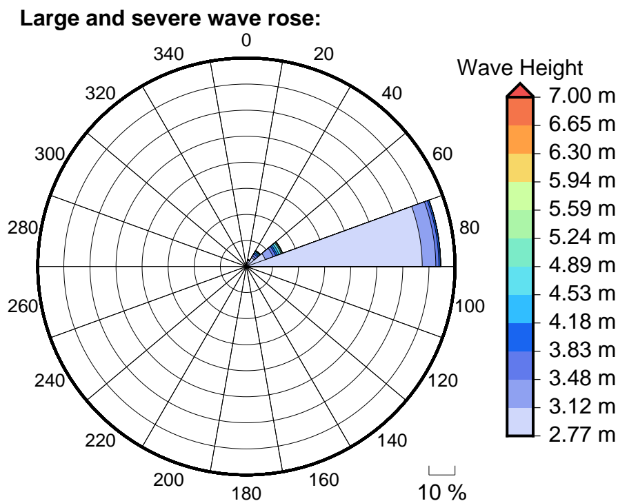
Figure 6 Large, severe and extreme wave roses for Tupapa
