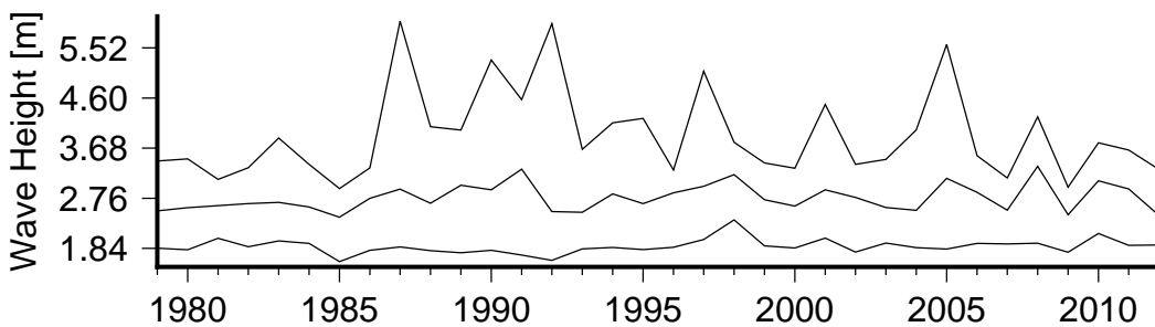
Figure 8 Annual variation in large waves (90th percentile)(lower curve), severe waves (99th percentile) (middle curve) and the largest wave(upper curve) in Tupapa.
