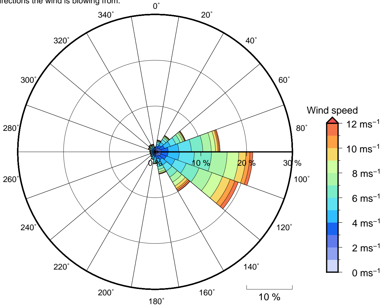
Figure 11 Annual wind rose for Fiji Wave Buoy. Note that directions are where the wind is coming from.
