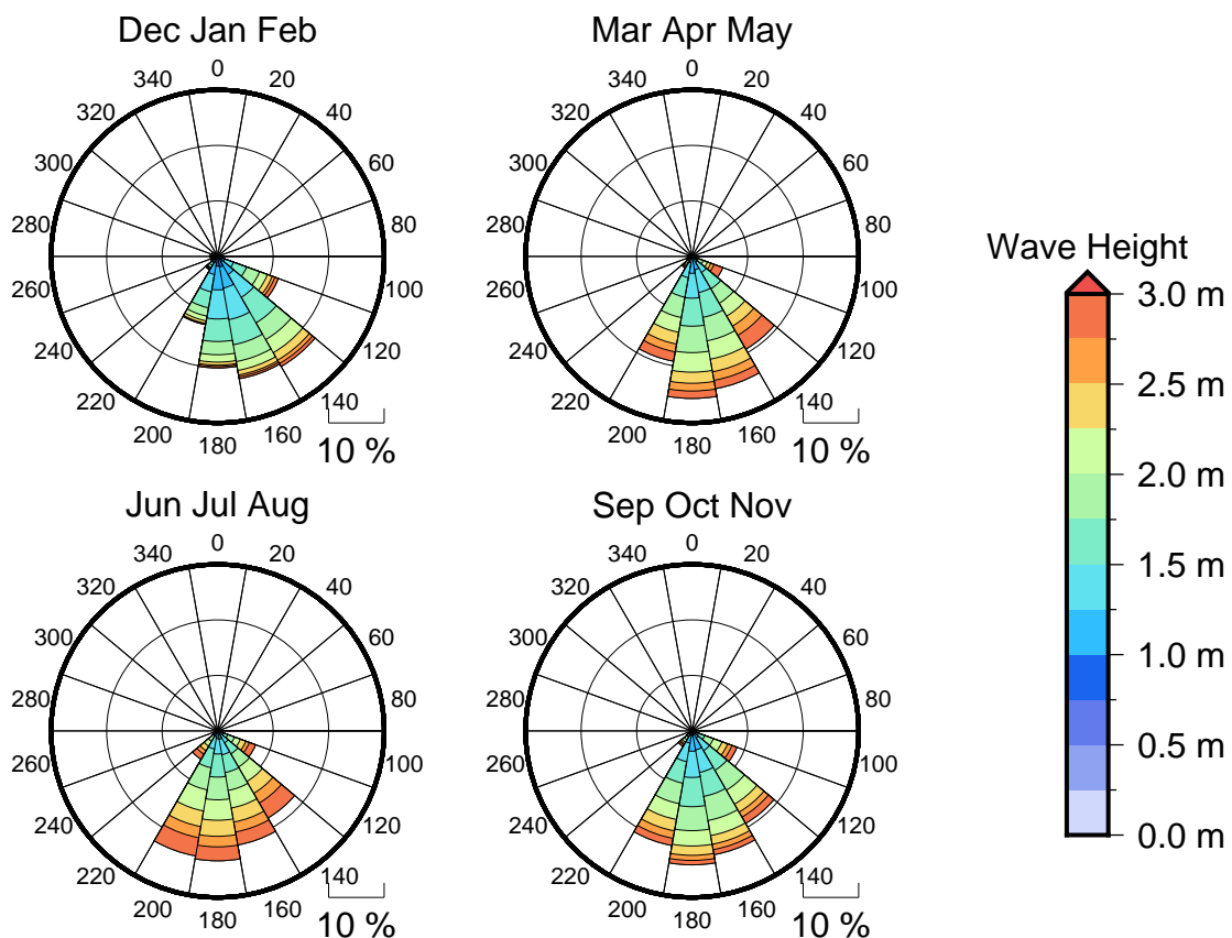
Figure 3 Seasonal wave roses for Fiji Wave Buoy
