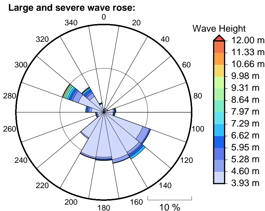
Figure 6 Large, severe and extreme wave roses for Fiji Wave Buoy
