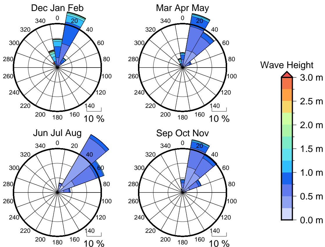
Figure 3 Seasonal wave roses for Labasa Channel
