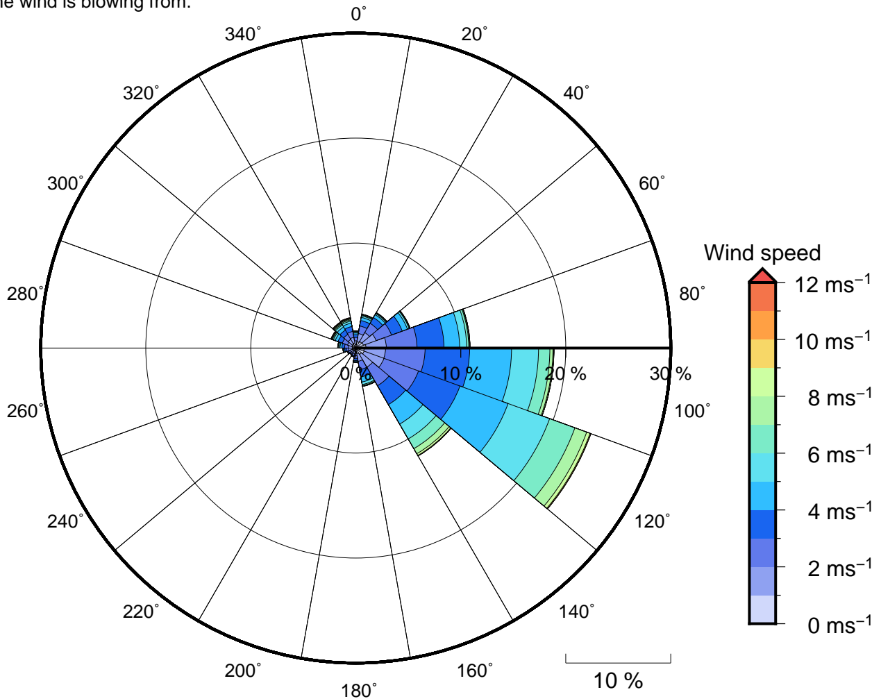
Figure 11 Annual wind rose for Labasa Channel. Note that directions are where the wind is coming from.
