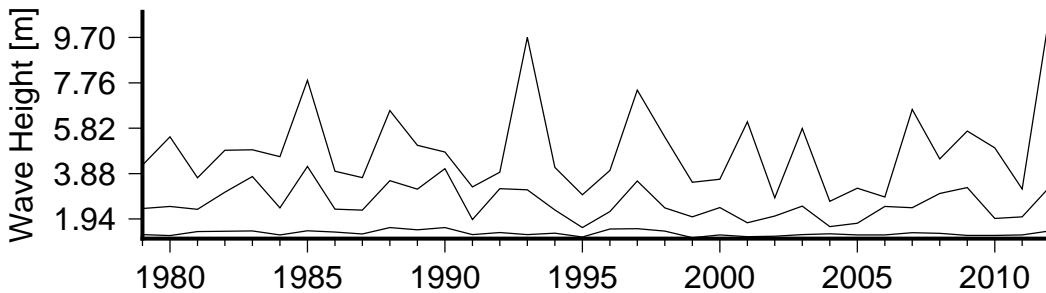
Figure 8 Annual variation in large waves (90th percentile)(lower curve), severe waves (99th percentile) (middle curve) and the largest wave(upper curve) in Labasa Channel.
