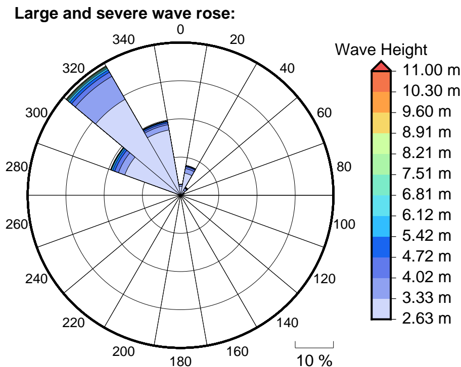
Figure 6 Large, severe and extreme wave roses for Labasa Channel
