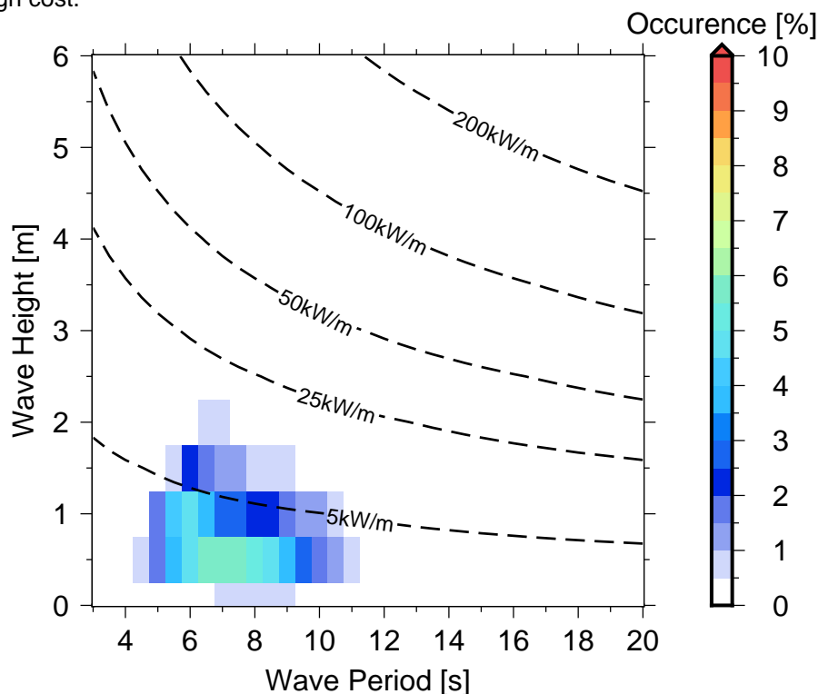
Figure 10 Occurrences of sea states in Levuka .
