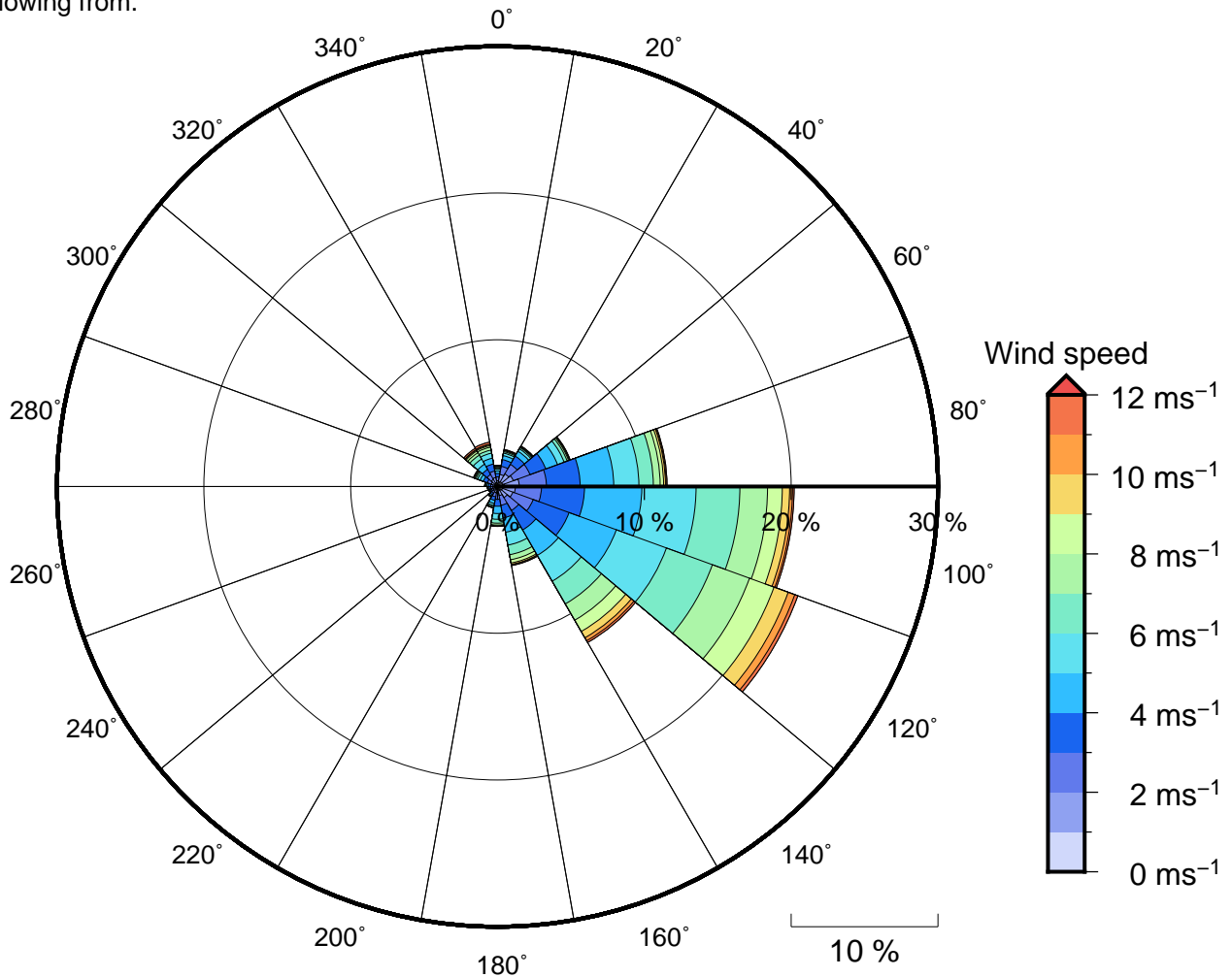
Figure 11 Annual wind rose for Levuka. Note that directions are where the wind is coming from.
