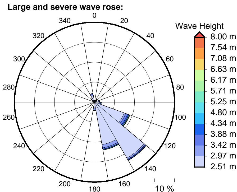
Figure 6 Large, severe and extreme wave roses for Levuka
