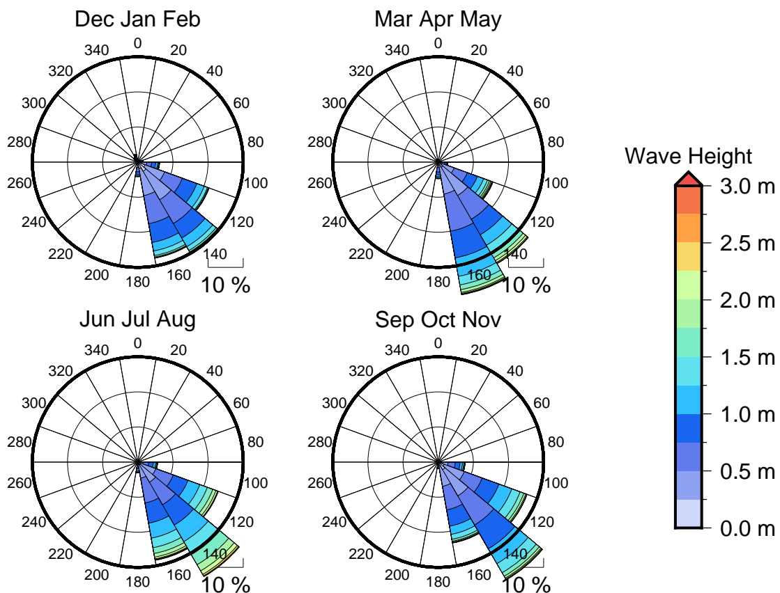
Figure 3 Seasonal wave roses for Levuka
