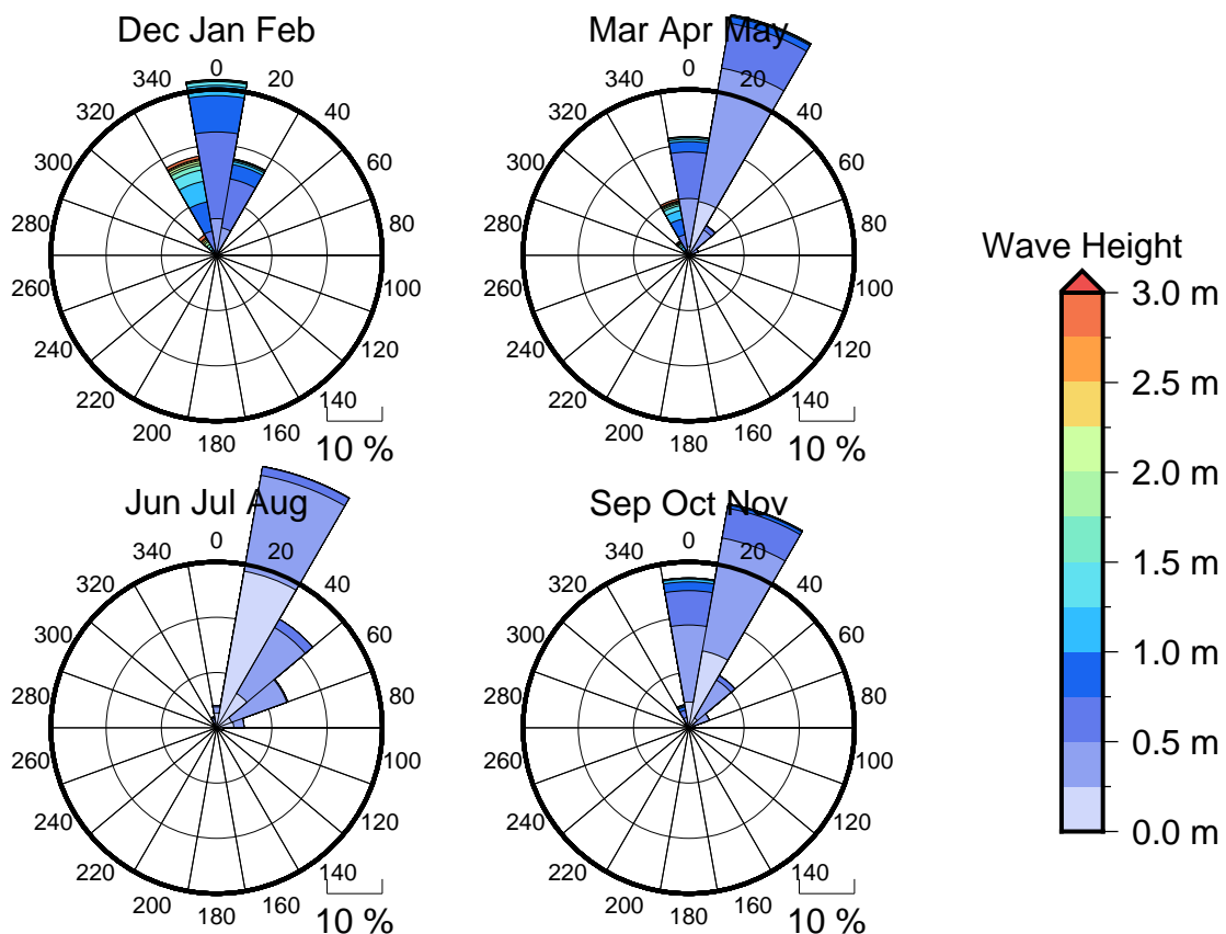
Figure 3 Seasonal wave roses for Malau
