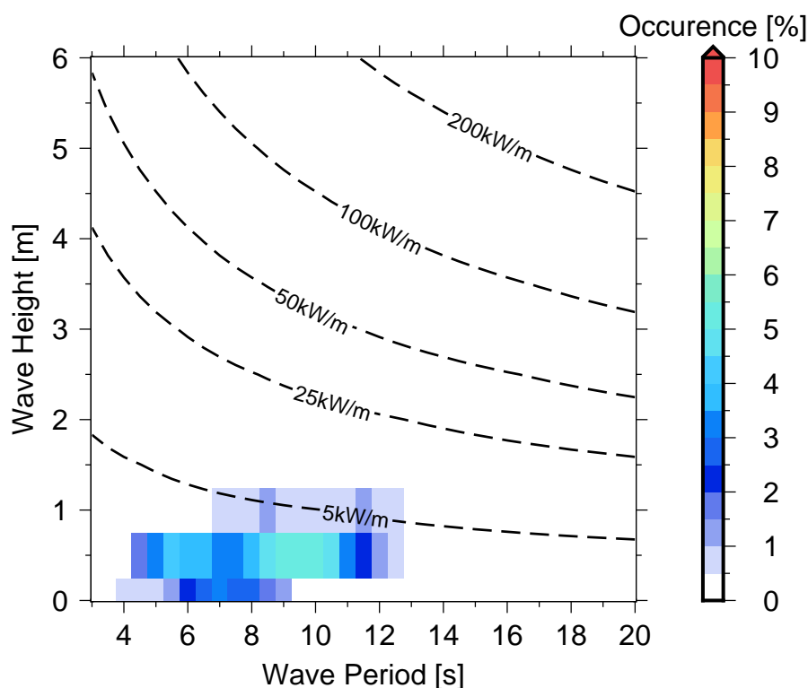
Figure 10 Occurrences of sea states in Malau .
