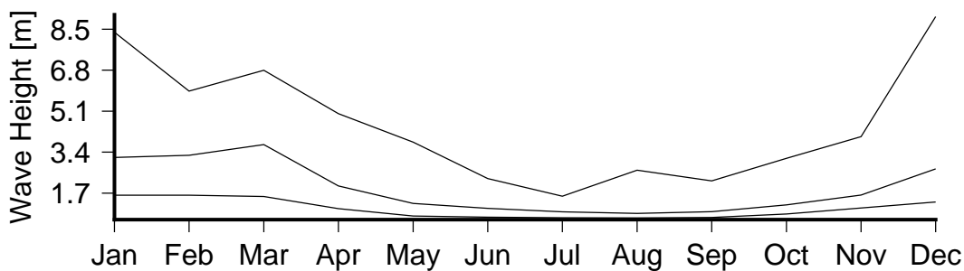
Figure 7 Monthly variation in large waves (90th percentile)(lower curve), severe waves (99th percentile) (middle curve) and the largest wave(upper curve) in Malau.
