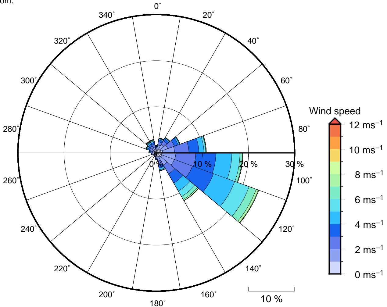
Figure 11 Annual wind rose for Malau. Note that directions are where the wind is coming from .
