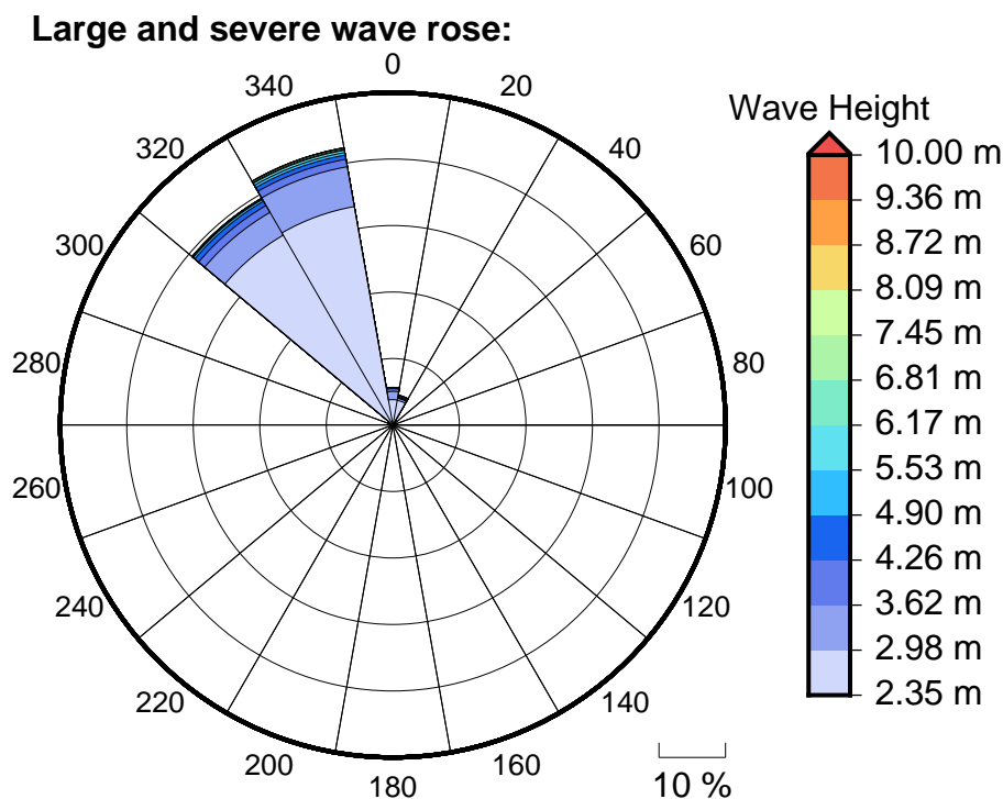
Figure 6 Large, severe and extreme wave roses for Malau
