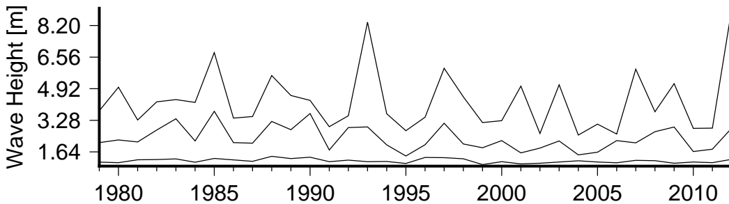
Figure 8 Annual variation in large waves (90th percentile)(lower curve), severe waves (99th percentile) (middle curve) and the largest wave(upper curve) in Malau.
