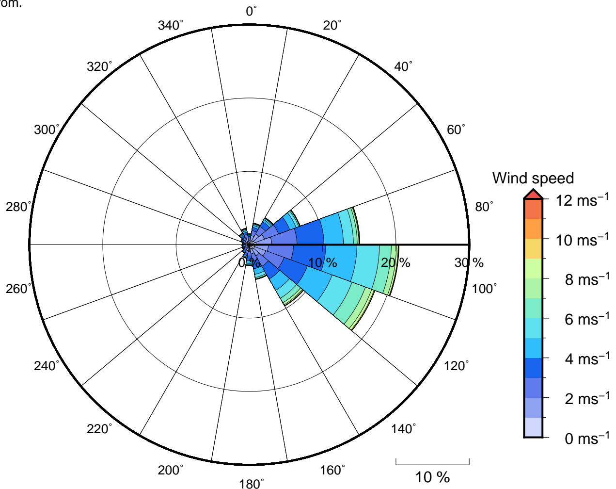
Figure 11 Annual wind rose for Suva. Note that directions are where the wind is coming from.
