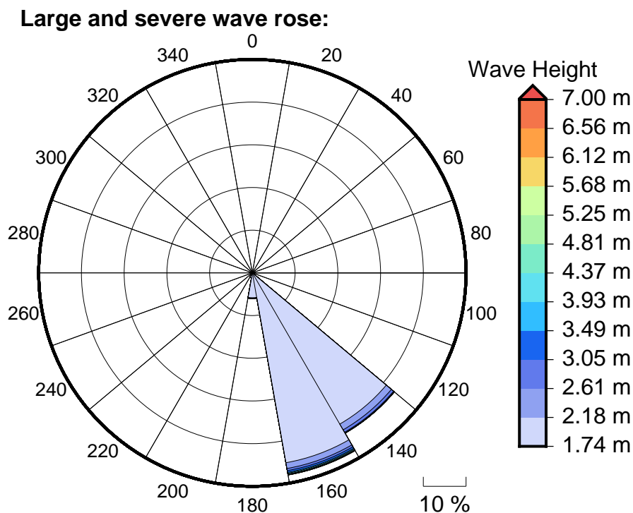
Figure 6 Large, severe and extreme wave roses for Suva
