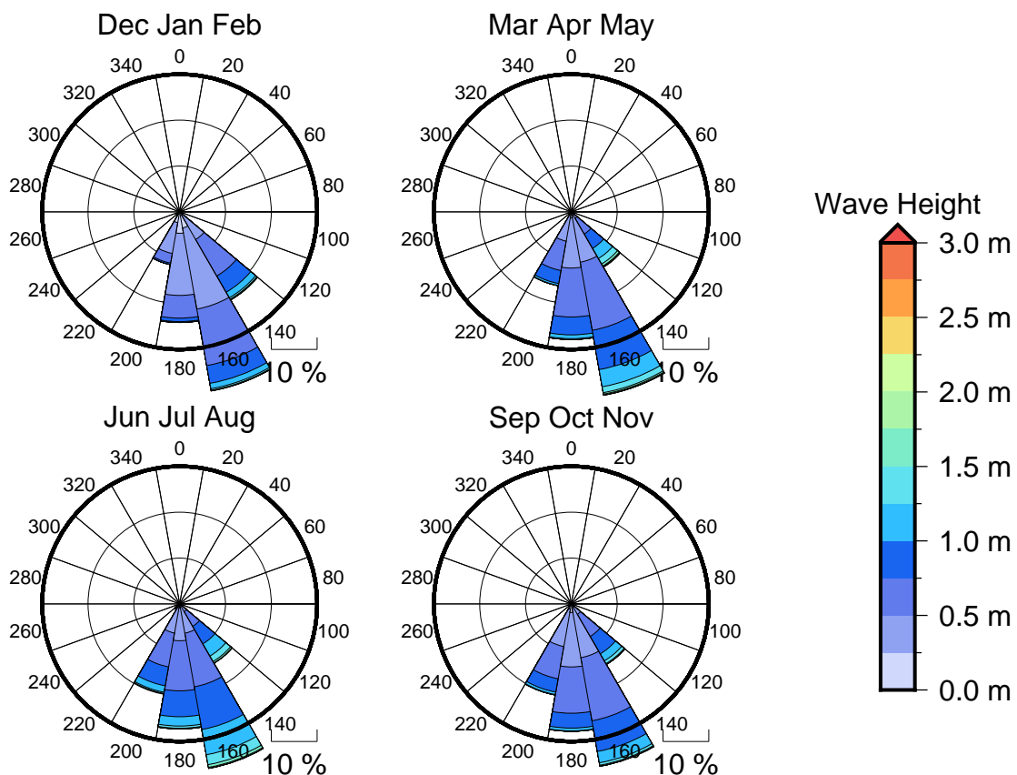
Figure 3 Seasonal wave roses for Suva
