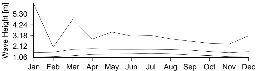
Figure 7 Monthly variation in large waves (90th percentile)(lower curve), severe waves (99th percentile) (middle curve) and the largest wave(upper curve) in Suva.
