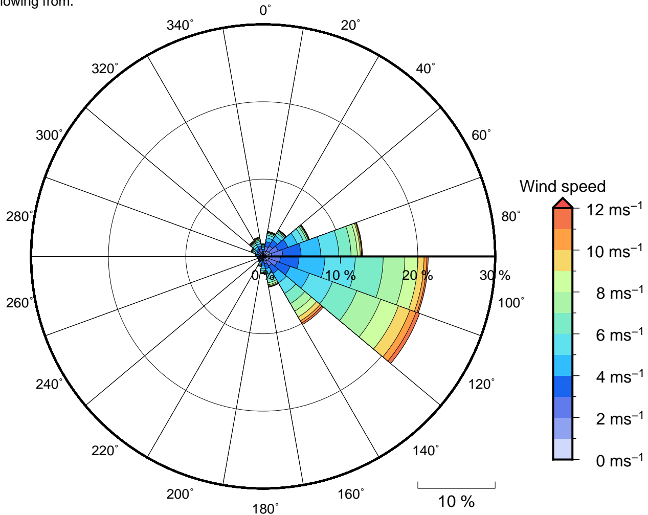
Figure 11 Annual wind rose for Taveuni. Note that directions are where the wind is coming from.
