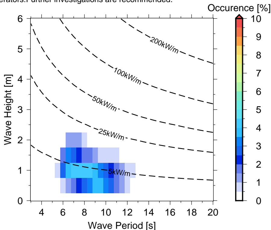
Figure 10 Occurrences of sea states in Taveuni .
