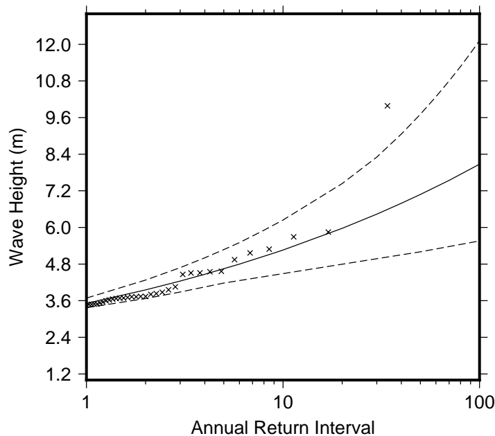
Figure 9 Extreme wave distribution for Taveuni. The crosses represents the wave events that occurred since 1979. The plain line is the statistical distribution that best fit the past wave events. The dotted line show the upper and lower high confidence of the fit, there is a 95% chance that the fitted distribution lie between the two dashed lines.
