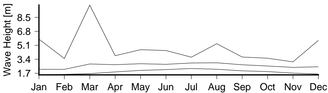
Figure 7 Monthly variation in large waves (90th percentile)(lower curve), severe waves (99th percentile) (middle curve) and the largest wave(upper curve) in Taveuni.
