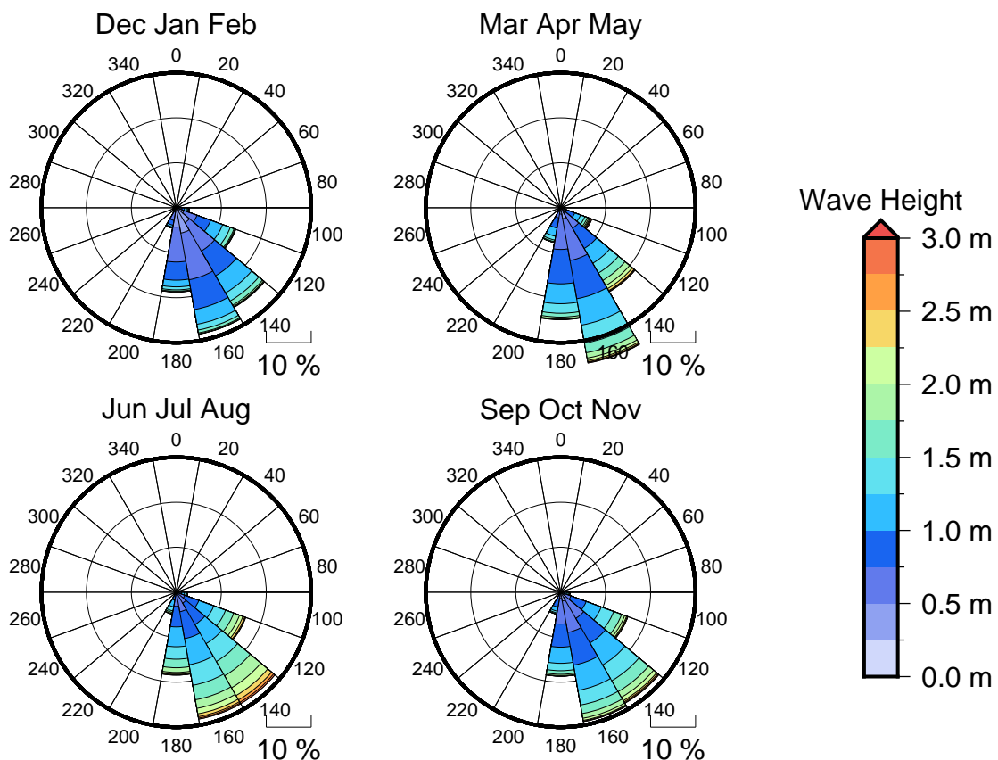
Figure 3 Seasonal wave roses for Taveuni
