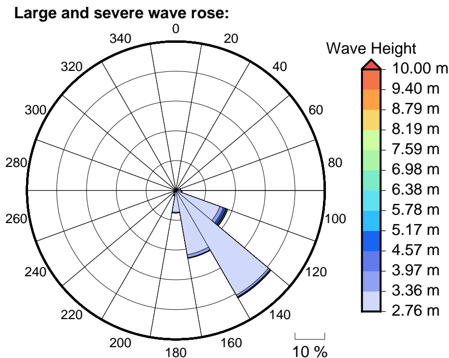
Figure 6 Large, severe and extreme wave roses for Taveuni
