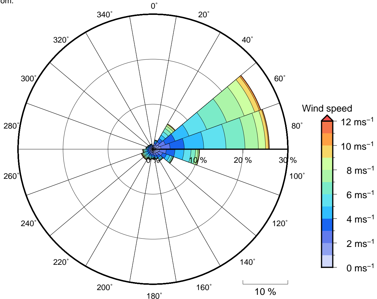
Figure 11 Annual wind rose for Chuuk. Note that directions are where the wind is coming from.
