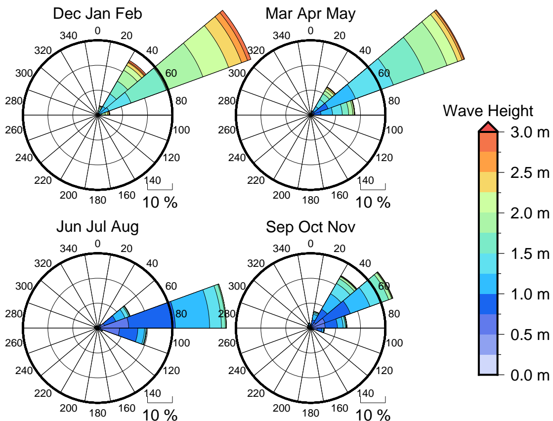
Figure 3 Seasonal wave roses for Chuuk
