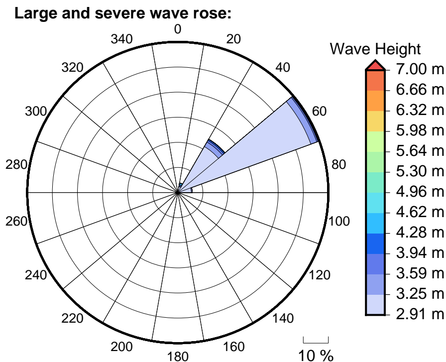
Figure 6 Large, severe and extreme wave roses for Chuuk
