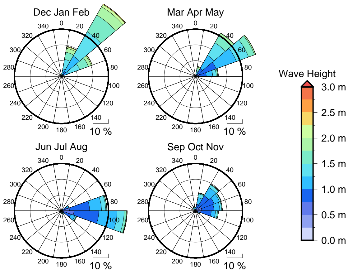
Figure 3 Seasonal wave roses for Kapingamarangi
