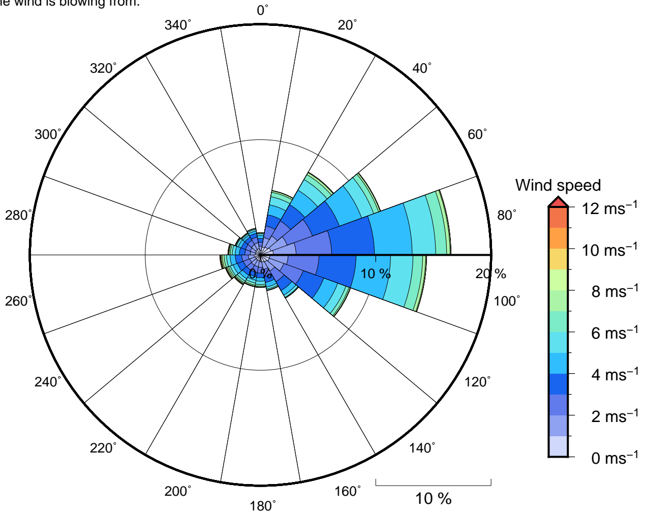
Figure 11 Annual wind rose for Kapingamarangi. Note that directions are where the wind is coming from.
