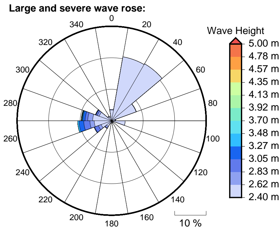
Figure 6 Large, severe and extreme wave roses for Kapingamarangi
