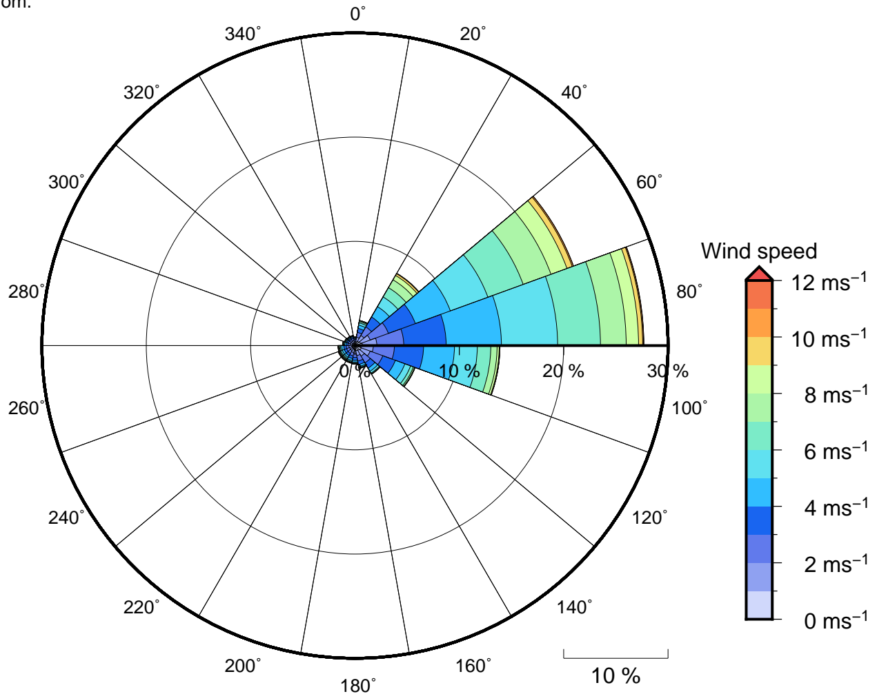
Figure 11 Annual wind rose for Kosrae. Note that directions are where the wind is coming from.
