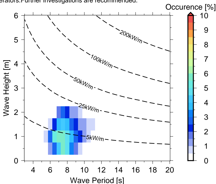
Figure 10 Occurrences of sea states in Kosrae .
