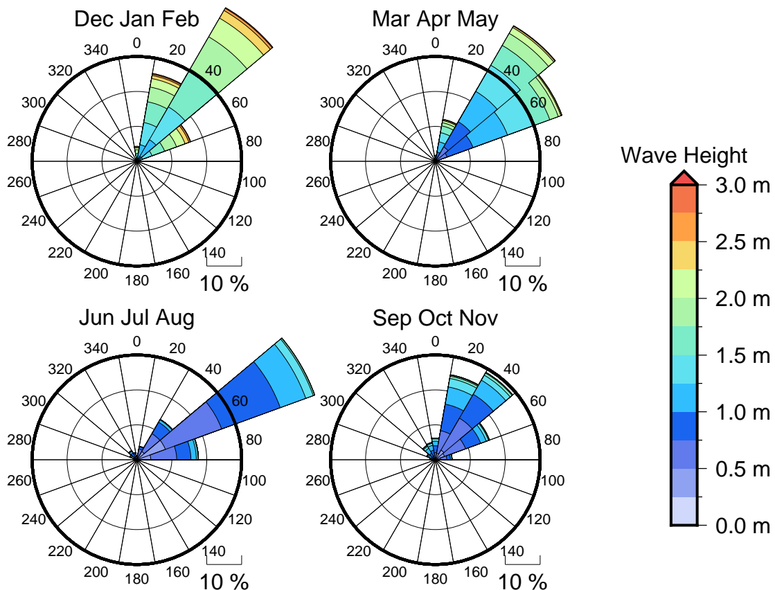
Figure 3 Seasonal wave roses for Kosrae
