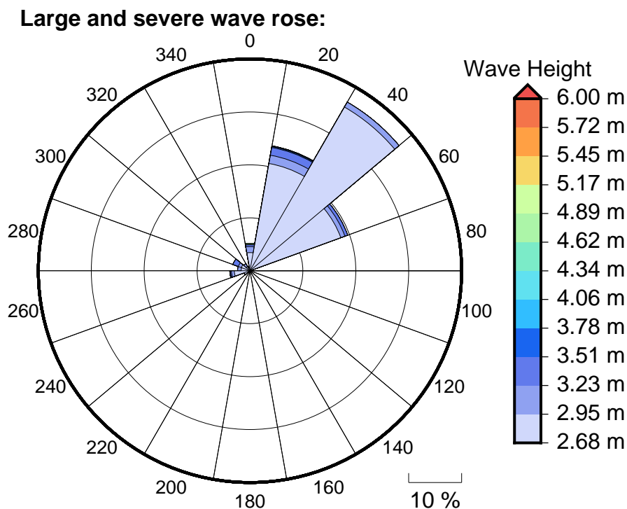
Figure 6 Large, severe and extreme wave roses for Kosrae
