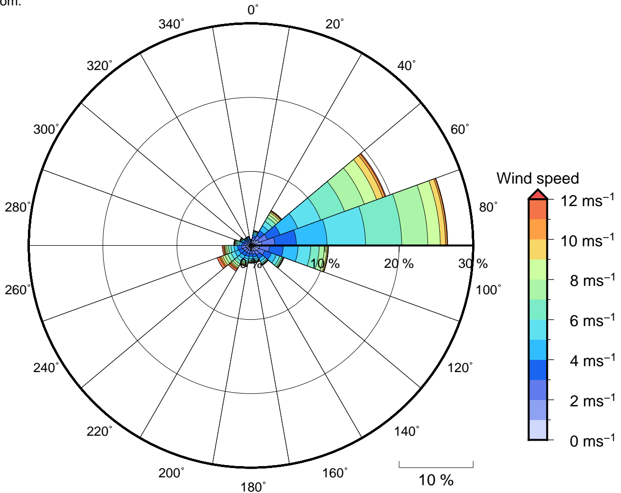
Figure 11 Annual wind rose for Yap. Note that directions are where the wind is coming from.
