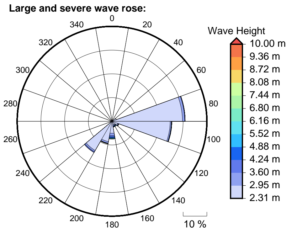
Figure 6 Large, severe and extreme wave roses for Yap
