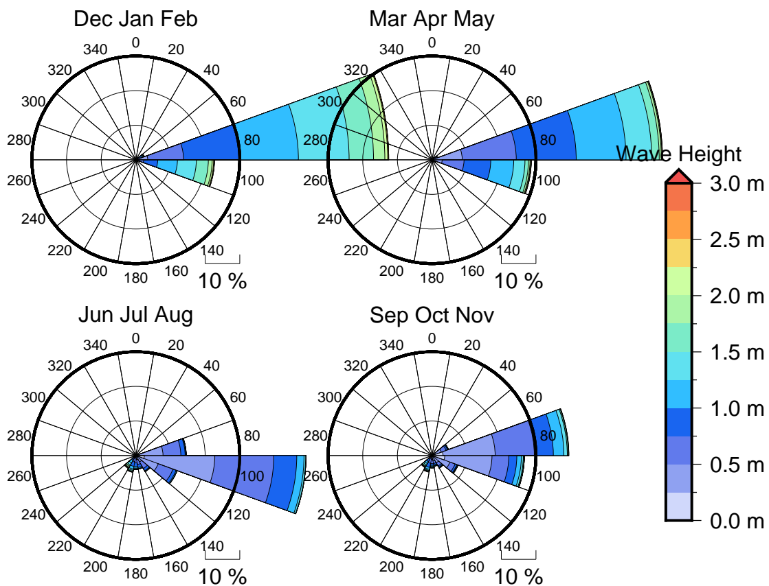
Figure 3 Seasonal wave roses for Yap
