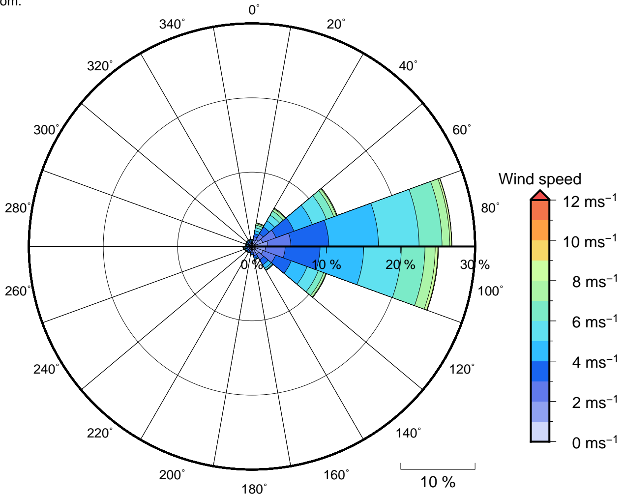
Figure 11 Annual wind rose for Betio. Note that directions are where the wind is coming from.
