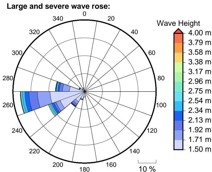
Figure 6 Large, severe and extreme wave roses for Betio
