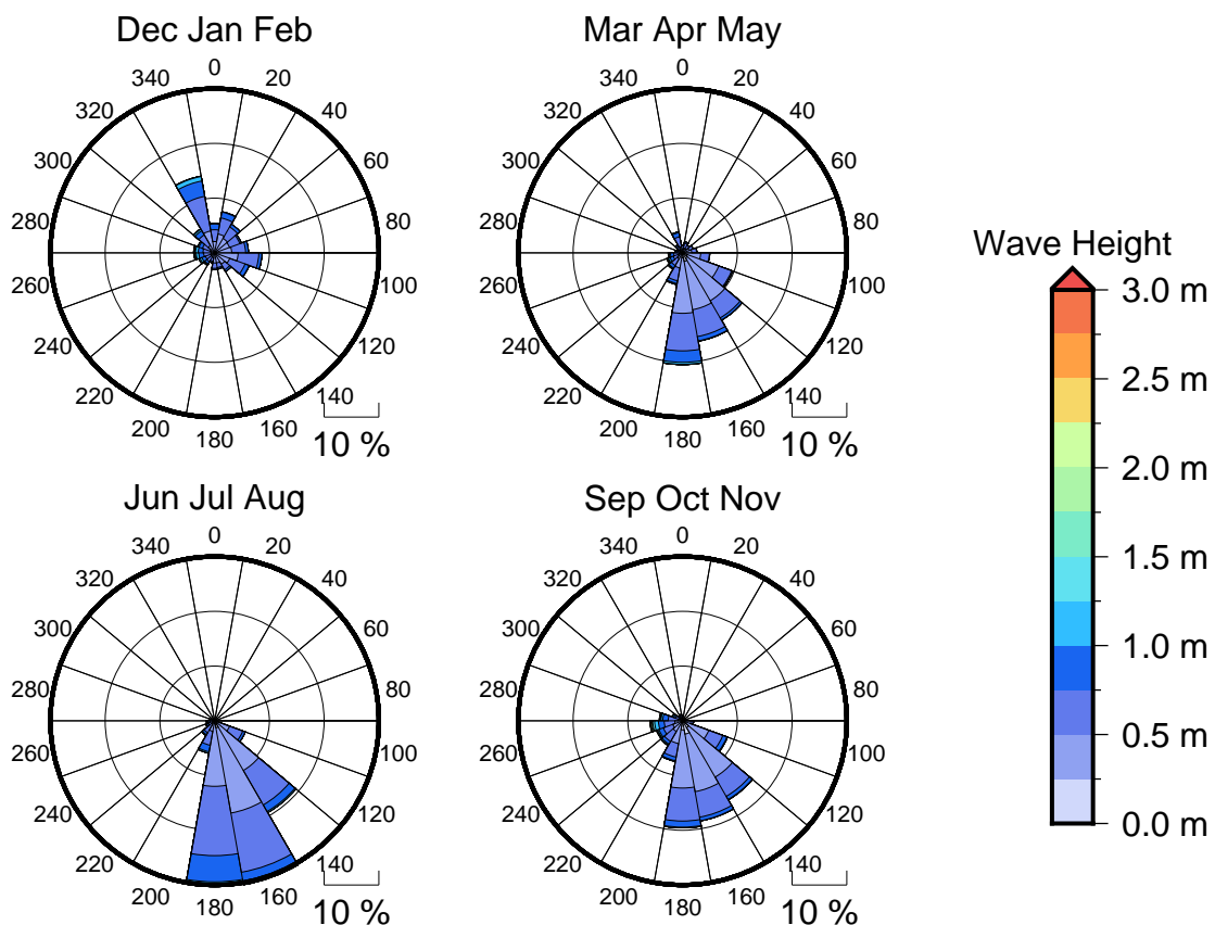
Figure 3 Seasonal wave roses for Betio
