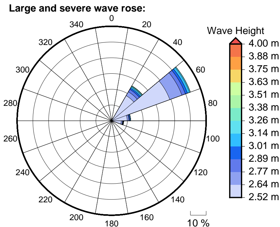
Figure 6 Large, severe and extreme wave roses for Bonriki
