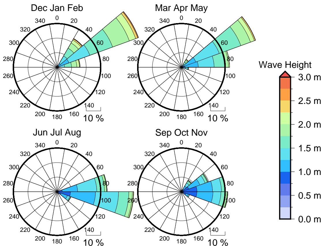
Figure 3 Seasonal wave roses for Bonriki
