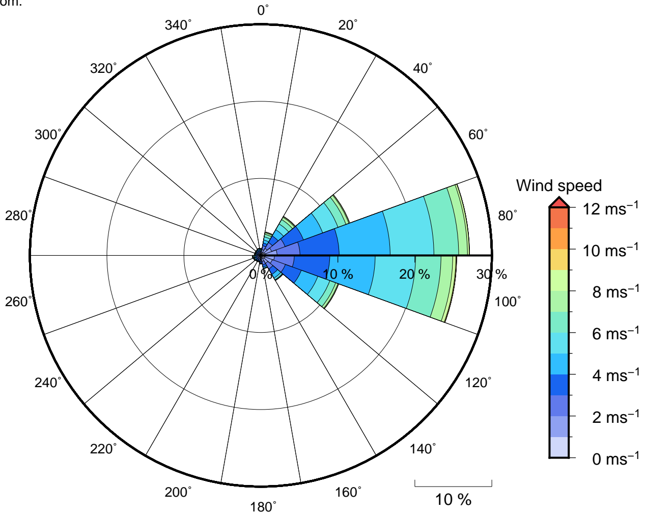
Figure 11 Annual wind rose for Bonriki. Note that directions are where the wind is coming from.
