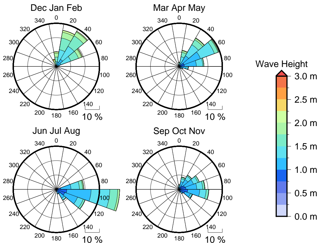
Figure 3 Seasonal wave roses for Canton Is.
