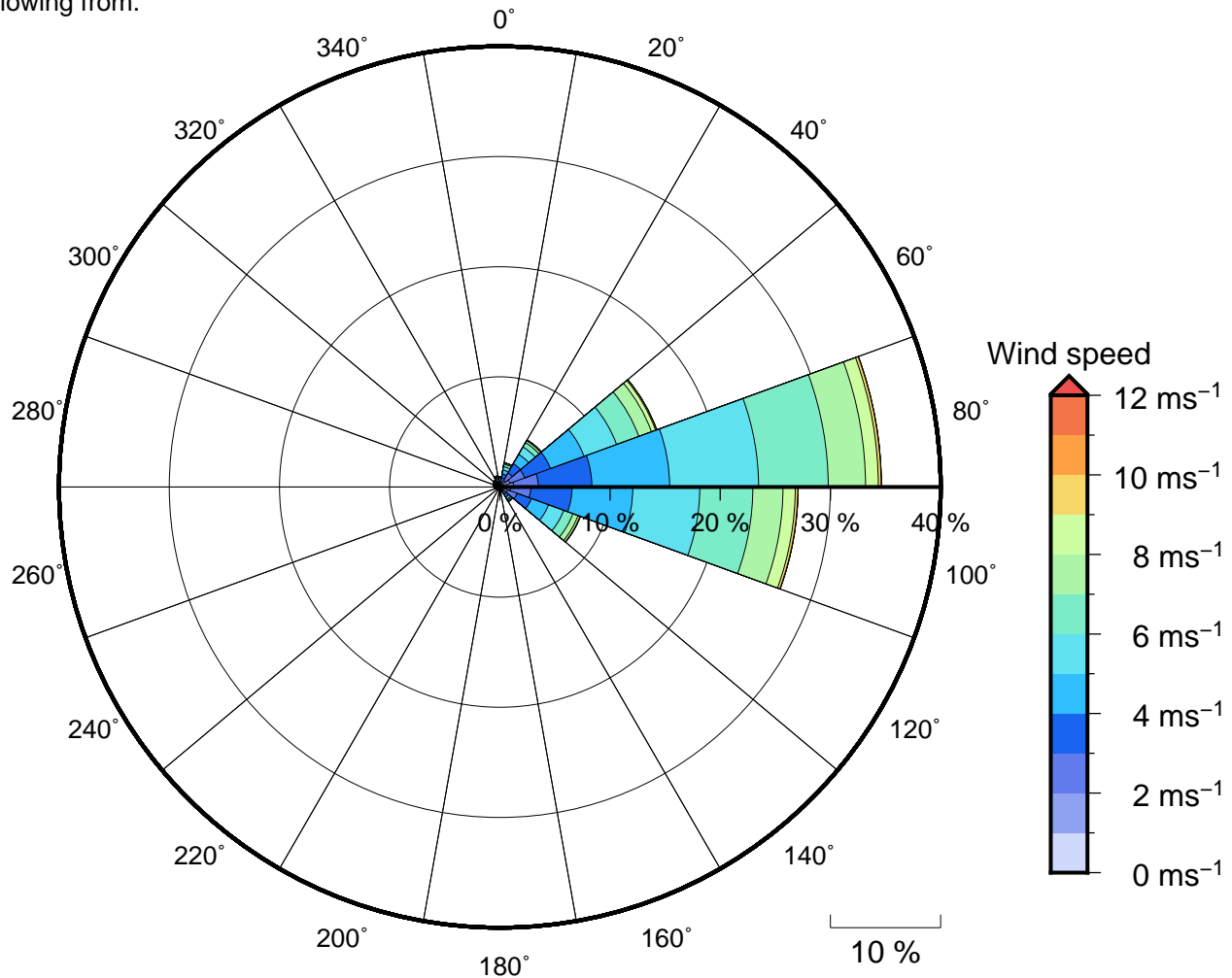
Figure 11 Annual wind rose for Canton Is.. Note that directions are where the wind is coming from .
