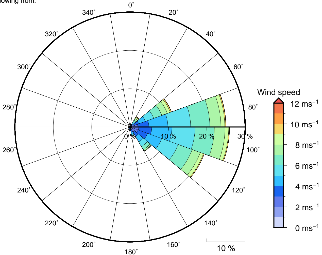
Figure 11 Annual wind rose for Fanning Is.. Note that directions are where the wind is coming from .
