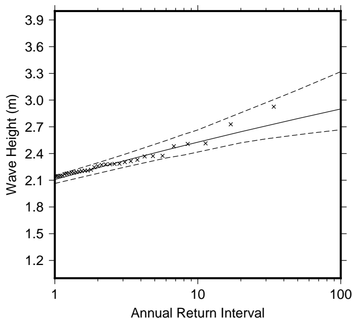
Figure 9 Extreme wave distribution for Fanning Is.. The crosses represents the wave events that occurred since 1979. The plain line is the statistical distribution that best fit the past wave events. The dotted line show the upper and lower high confidence of the fit, there is a 95% chance that the fitted distribution lie between the two dashed lines.
