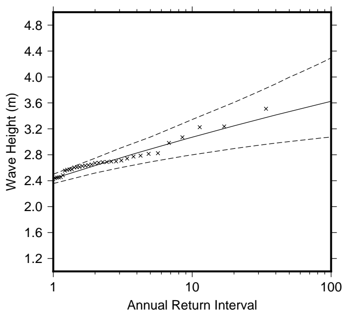
Figure 9 Extreme wave distribution for Kiritimati. The crosses represents the wave events that occurred since 1979. The plain line is the statistical distribution that best fit the past wave events. The dotted line show the upper and lower high confidence of the fit, there is a 95% chance that the fitted distribution lie between the two dashed lines.
