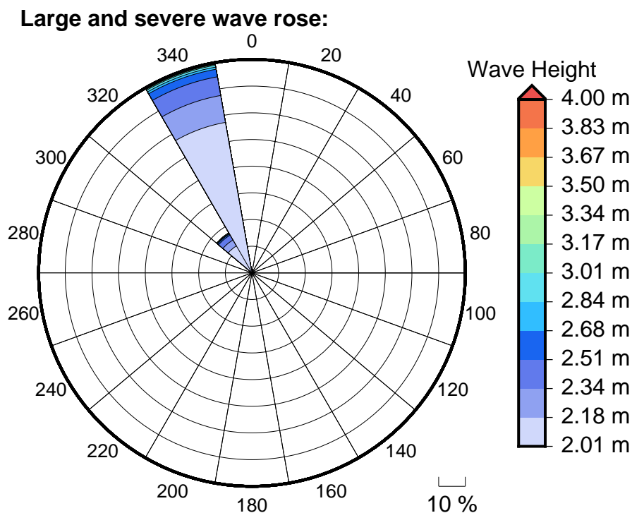
Figure 6 Large, severe and extreme wave roses for Kiritimati
