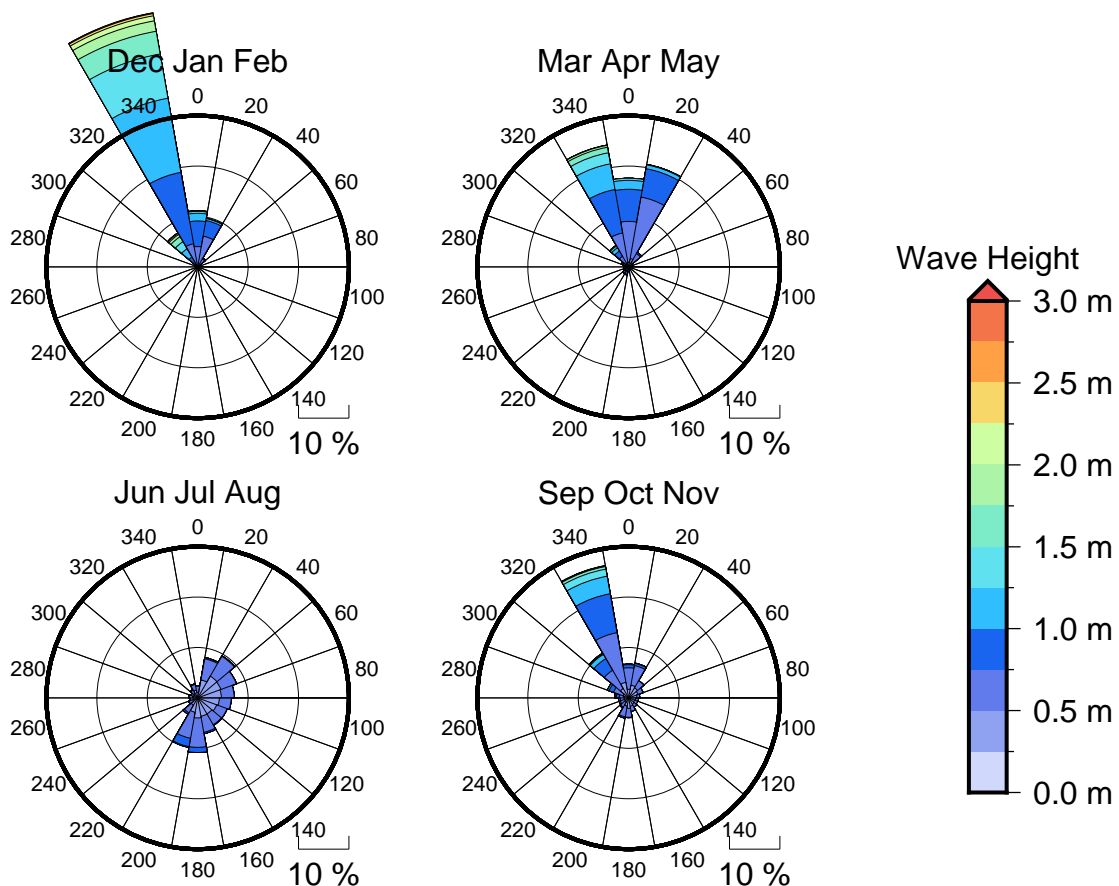
Figure 3 Seasonal wave roses for Kiritimati
