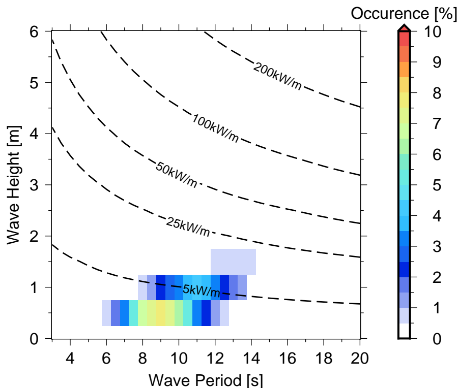
Figure 10 Occurrences of sea states in Kiritimati .
