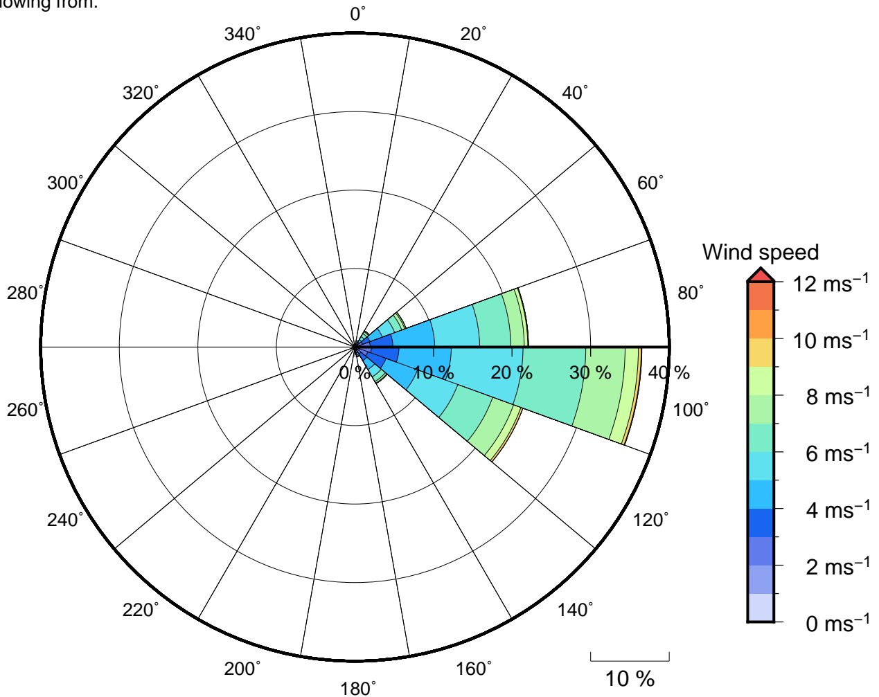
Figure 11 Annual wind rose for Kiritimati. Note that directions are where the wind is coming from .
