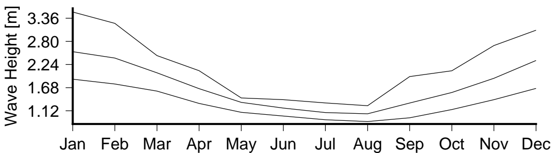
Figure 7 Monthly variation in large waves (90th percentile)(lower curve), severe waves (99th percentile) (middle curve) and the largest wave(upper curve) in Kiritimati.
