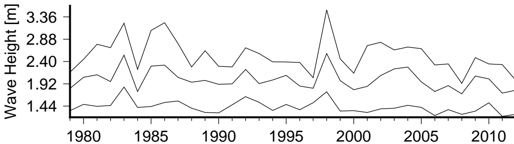
Figure 8 Annual variation in large waves (90th percentile)(lower curve), severe waves (99th percentile) (middle curve) and the largest wave(upper curve) in Kiritimati.
