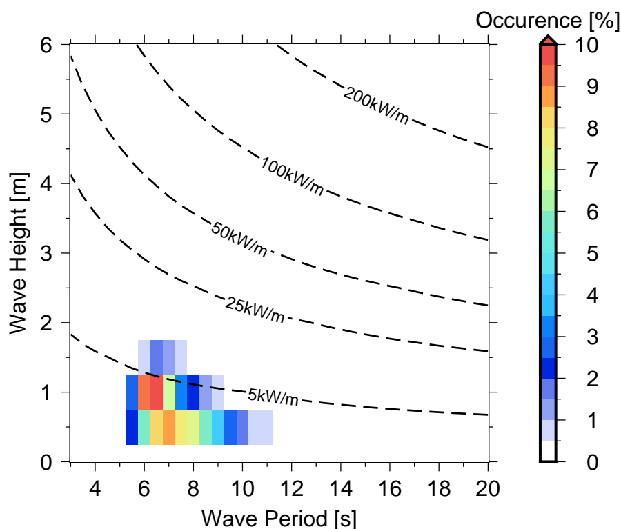
Figure 10 Occurrences of sea states in Kwajalein .
