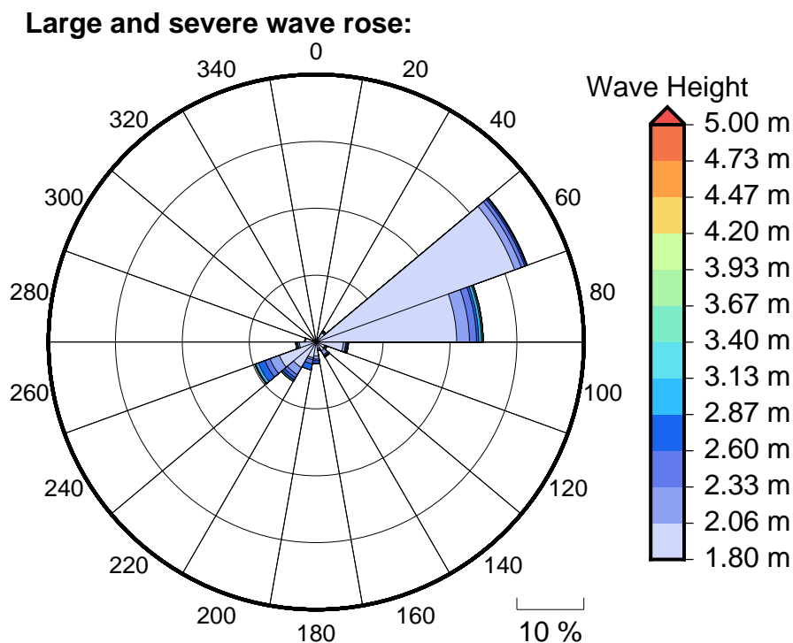
Figure 6 Large, severe and extreme wave roses for Kwajalein
