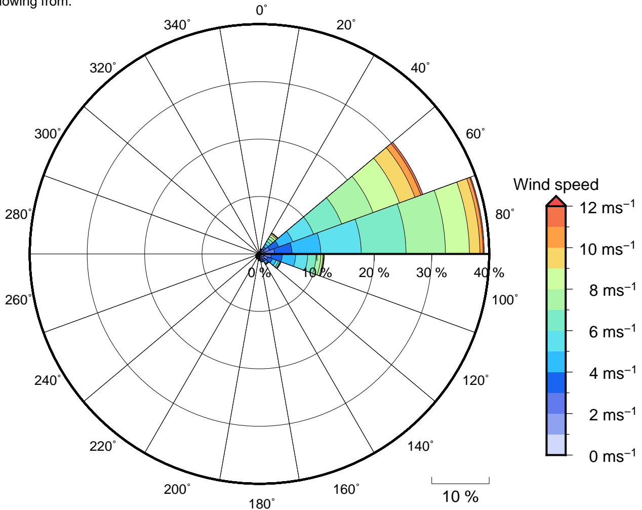
Figure 11 Annual wind rose for Kwajalein. Note that directions are where the wind is coming from.
