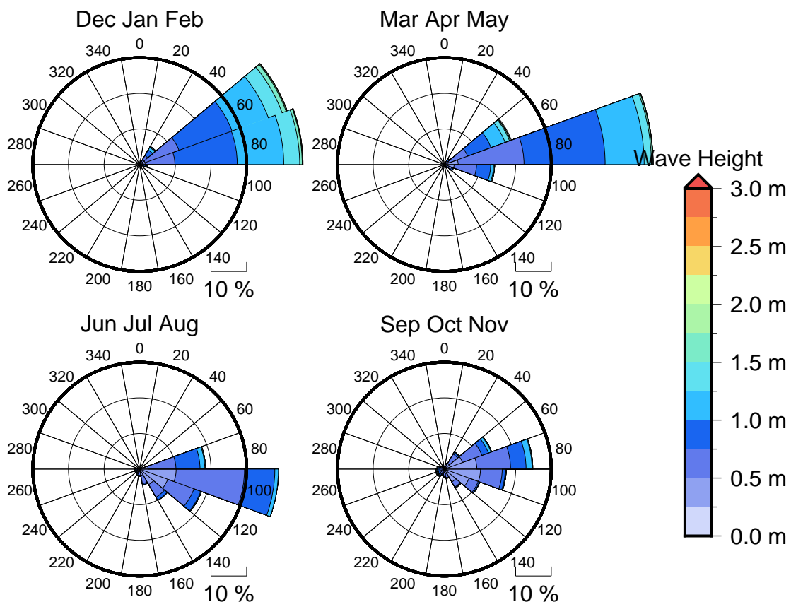
Figure 3 Seasonal wave roses for Kwajalein
