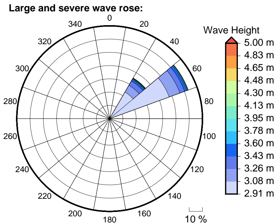
Figure 6 Large, severe and extreme wave roses for Majuro
