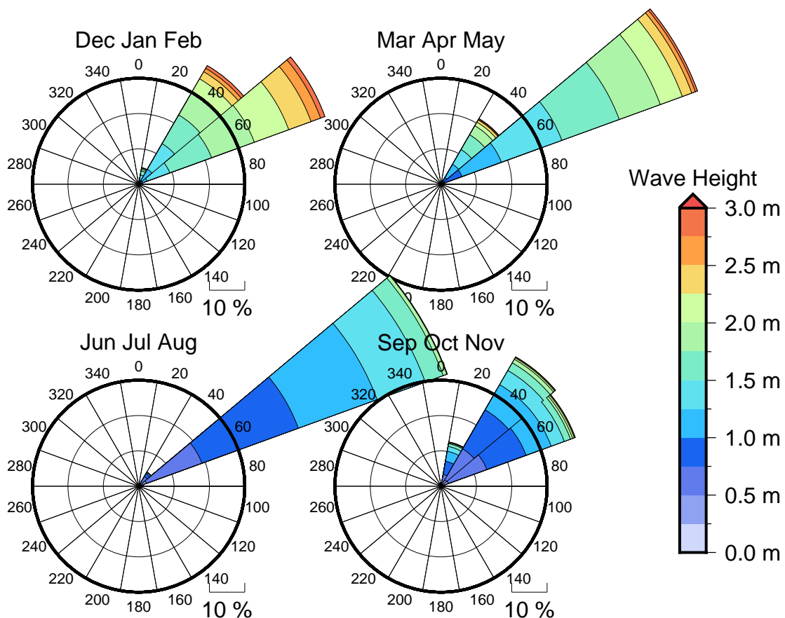
Figure 3 Seasonal wave roses for Majuro
