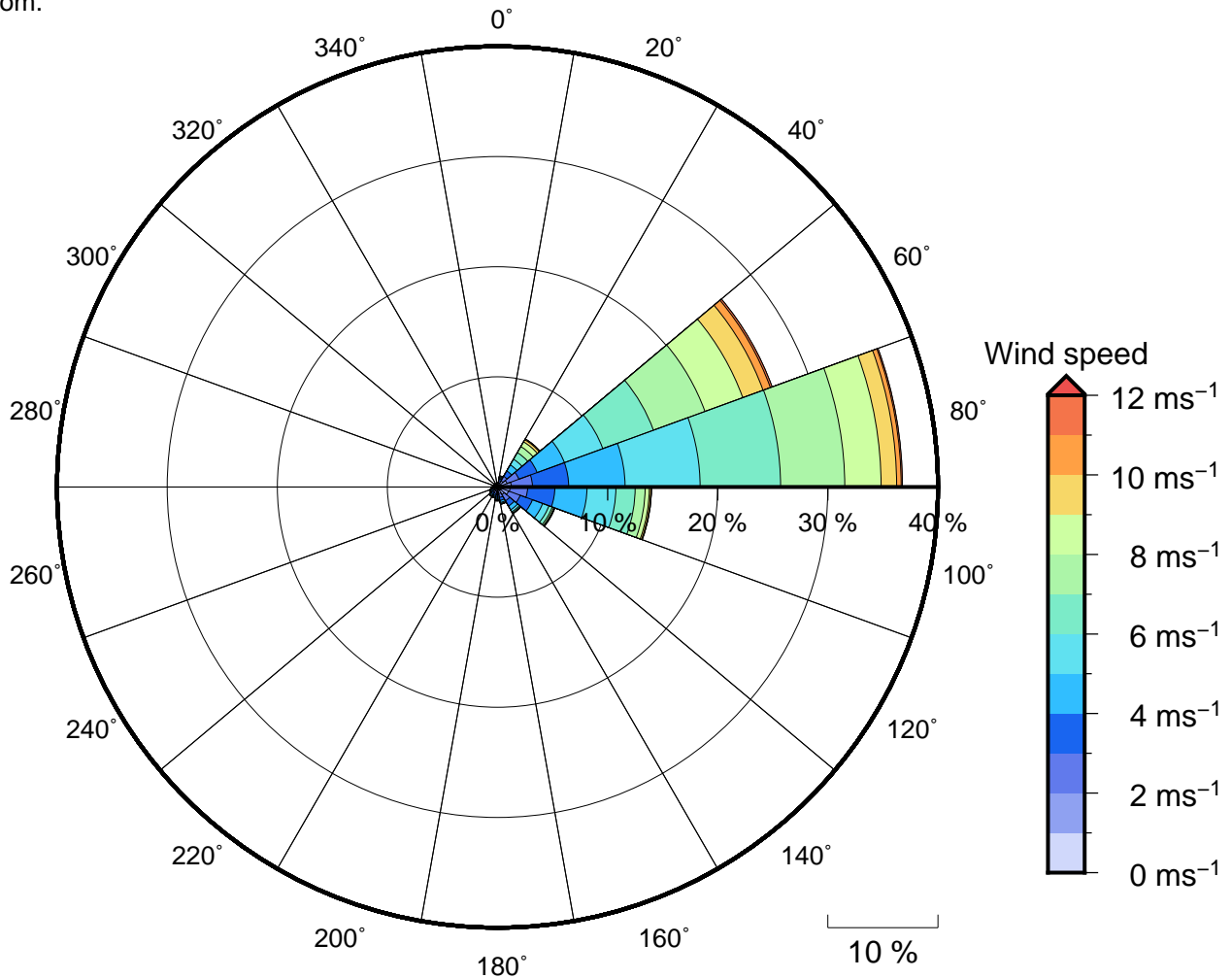
Figure 11 Annual wind rose for Majuro. Note that directions are where the wind is coming from.
