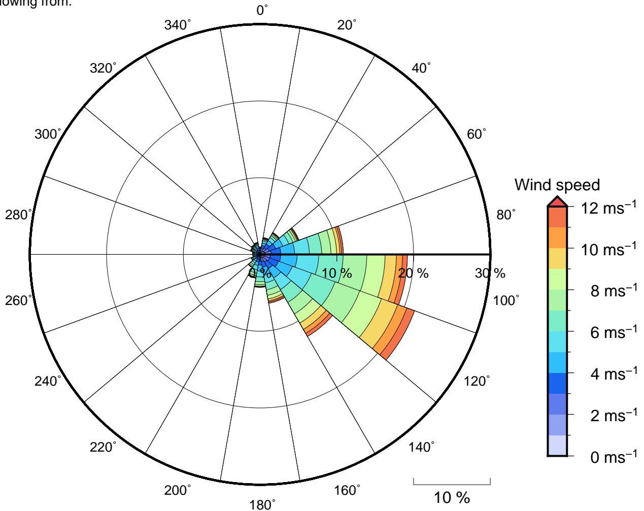
Figure 11 Annual wind rose for Mare Is.. Note that directions are where the wind is coming from.
