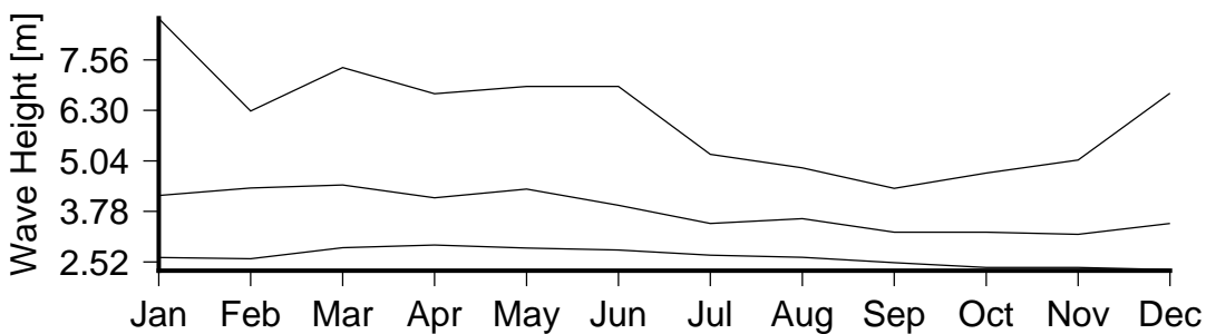
Figure 7 Monthly variation in large waves (90th percentile)(lower curve), severe waves (99th percentile) (middle curve) and the largest wave(upper curve) in Mare Is..
