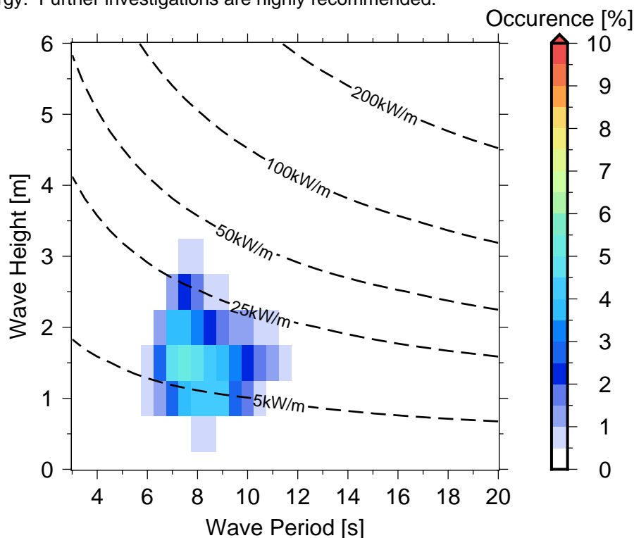
Figure 10 Occurrences of sea states in Mare Is. .
