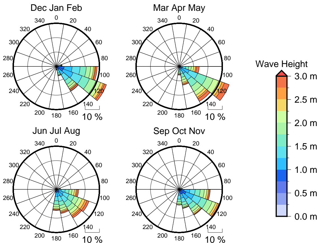
Figure 3 Seasonal wave roses for Mare Is.
