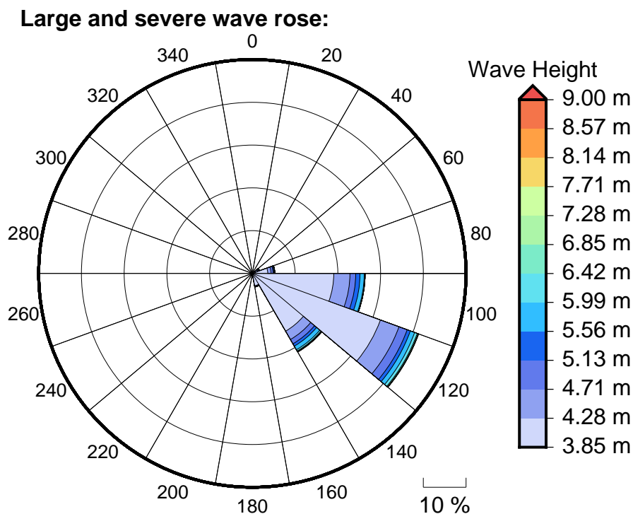
Figure 6 Large, severe and extreme wave roses for Mare Is.
