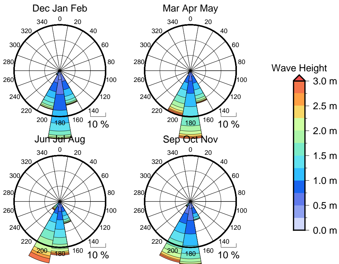
Figure 3 Seasonal wave roses for Nepoui
