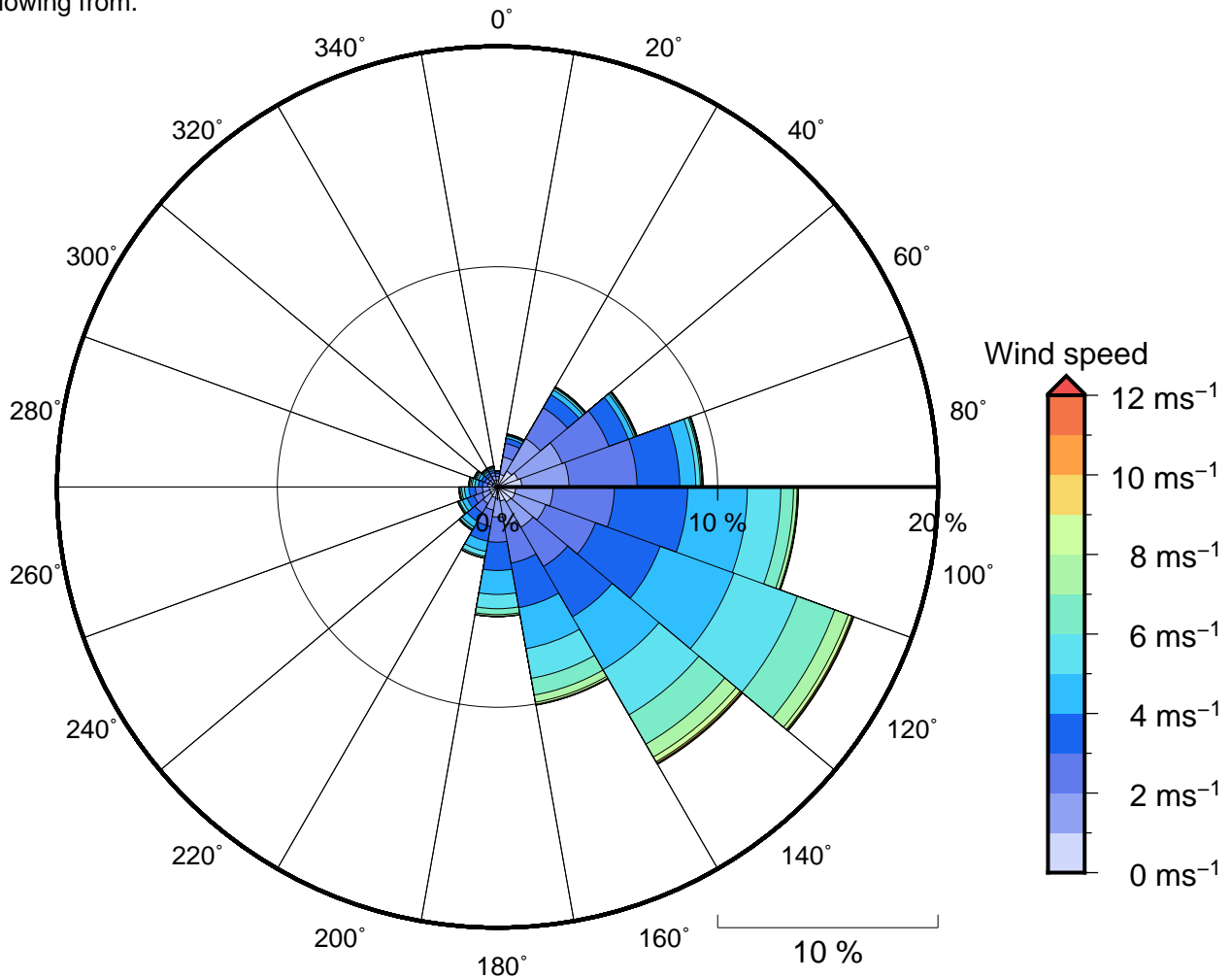
Figure 11 Annual wind rose for Nepoui. Note that directions are where the wind is coming from.
