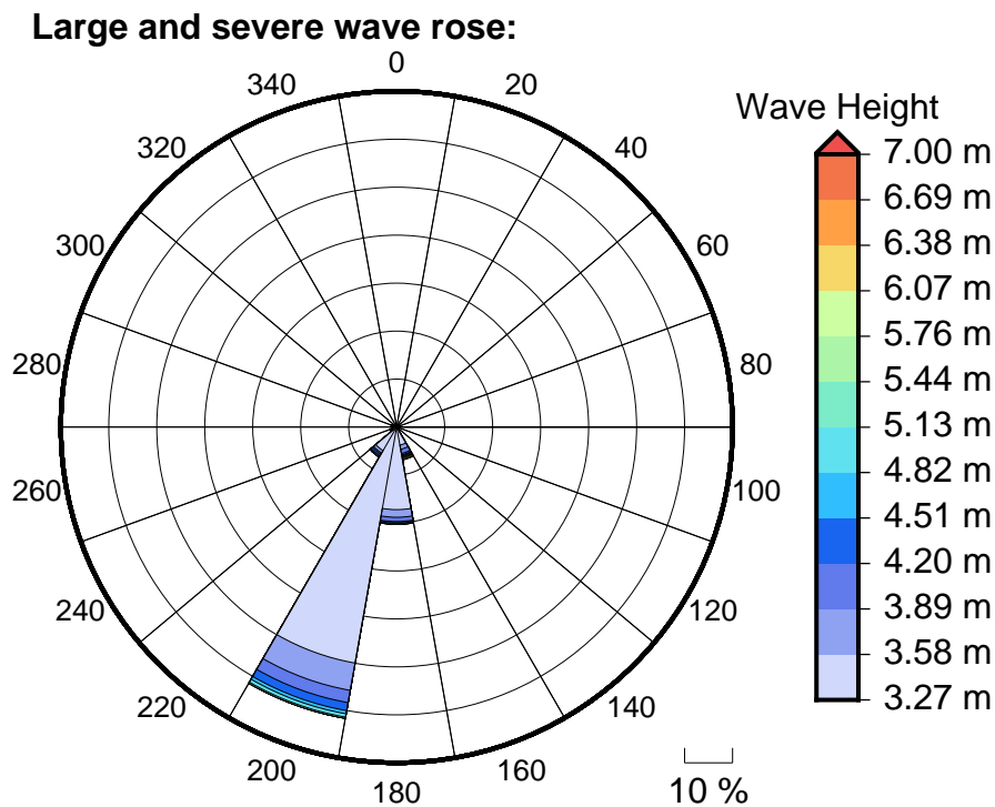
Figure 6 Large, severe and extreme wave roses for Nepoui
