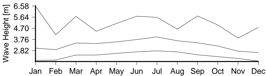
Figure 7 Monthly variation in large waves (90th percentile)(lower curve), severe waves (99th percentile) (middle curve) and the largest wave(upper curve) in Noumea.
