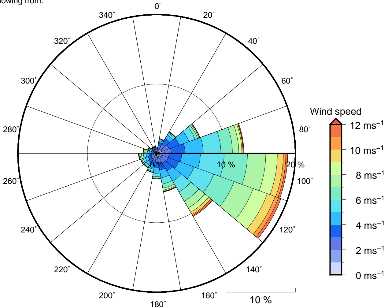
Figure 11 Annual wind rose for Noumea. Note that directions are where the wind is coming from .
