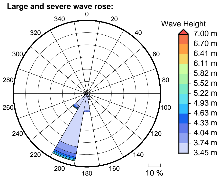
Figure 6 Large, severe and extreme wave roses for Noumea
