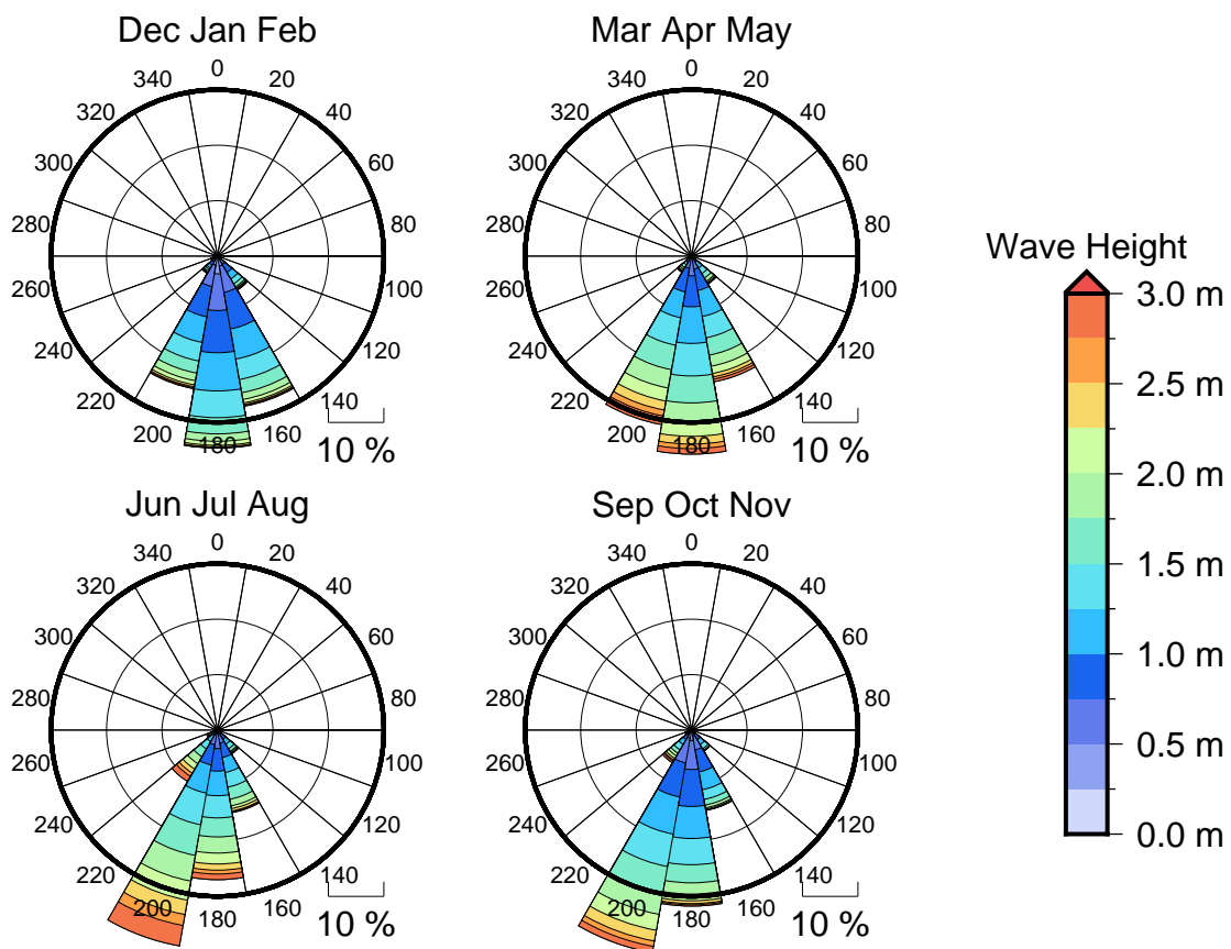
Figure 3 Seasonal wave roses for Noumea
