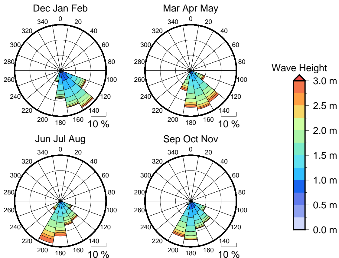
Figure 3 Seasonal wave roses for Pine Is.
