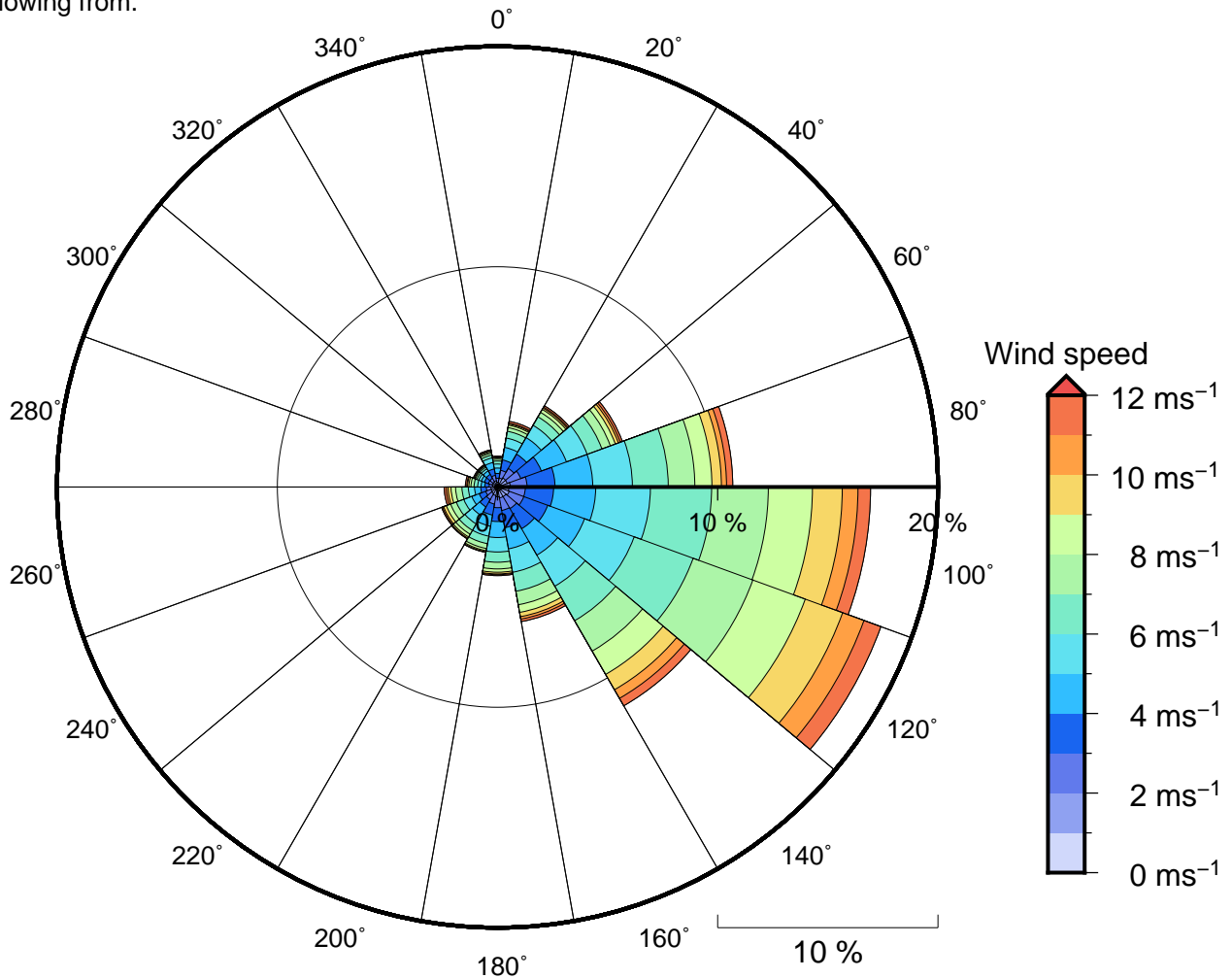
Figure 11 Annual wind rose for Pine Is.. Note that directions are where the wind is coming from .
