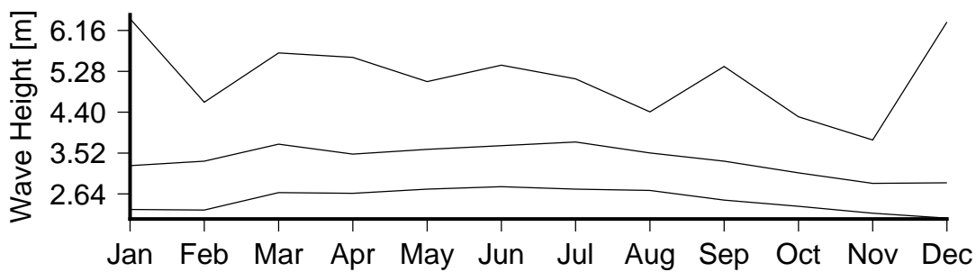
Figure 7 Monthly variation in large waves (90th percentile)(lower curve), severe waves (99th percentile) (middle curve) and the largest wave(upper curve) in Pine Is..
