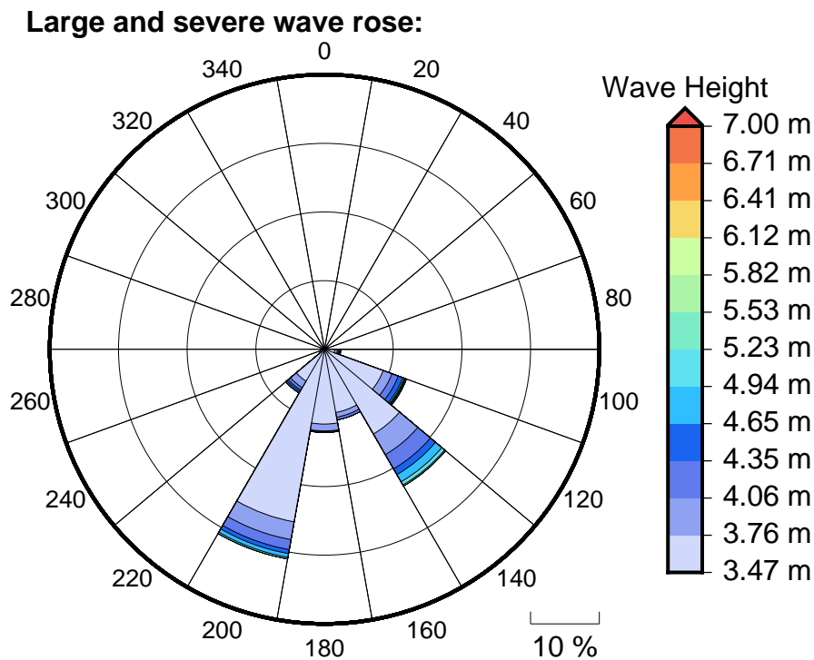
Figure 6 Large, severe and extreme wave roses for Pine Is.
