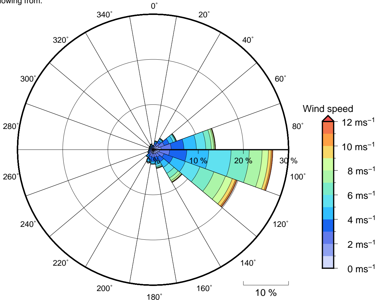
Figure 11 Annual wind rose for Poindimie. Note that directions are where the wind is coming from.
