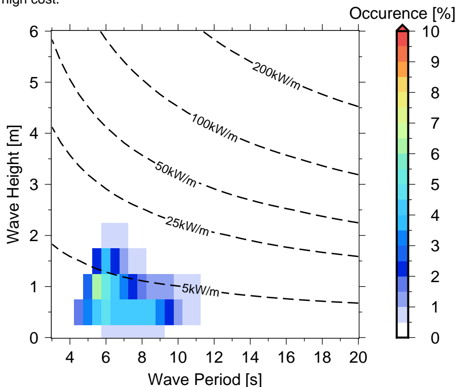
Figure 10 Occurrences of sea states in Poindimie .
