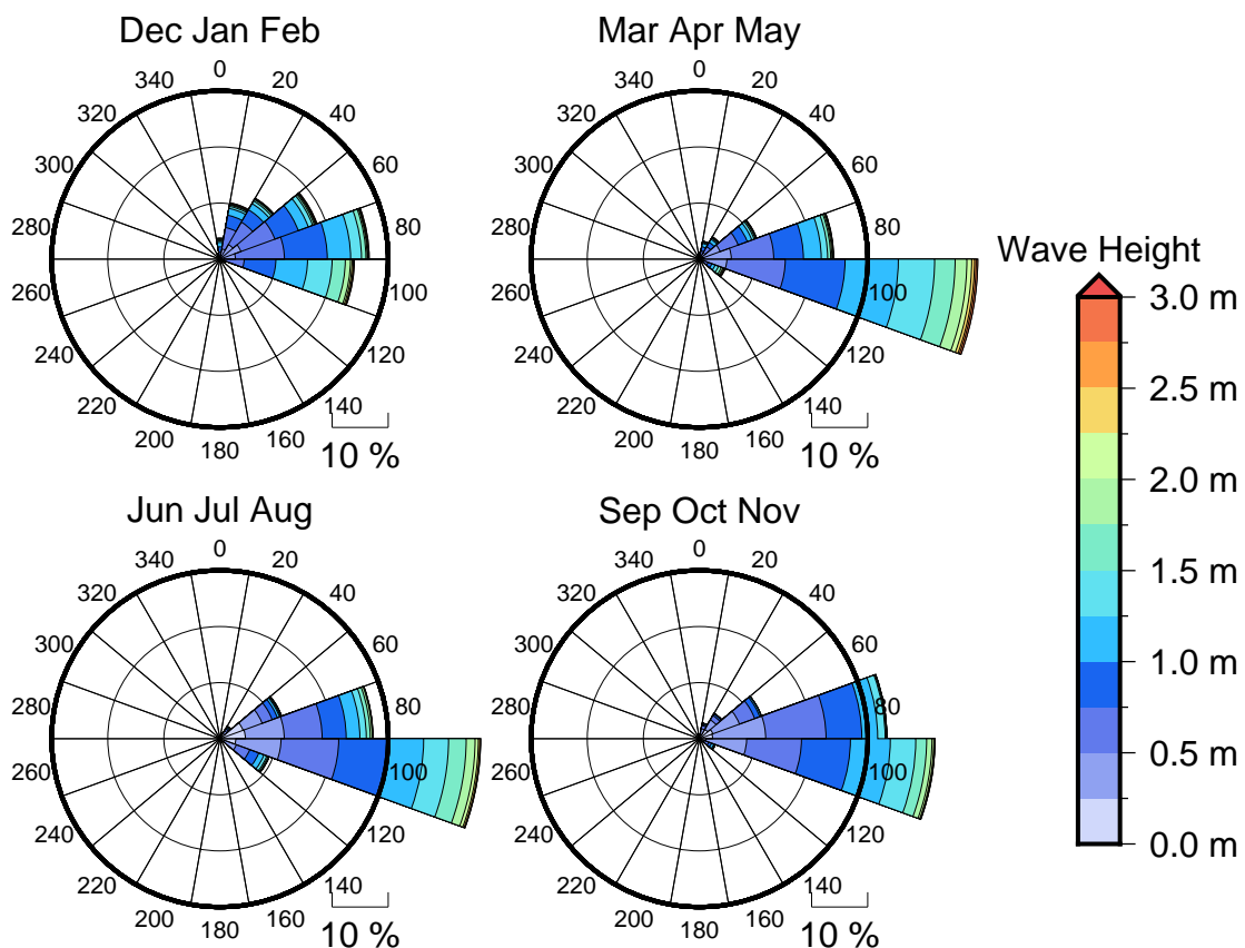
Figure 3 Seasonal wave roses for Poindimie
