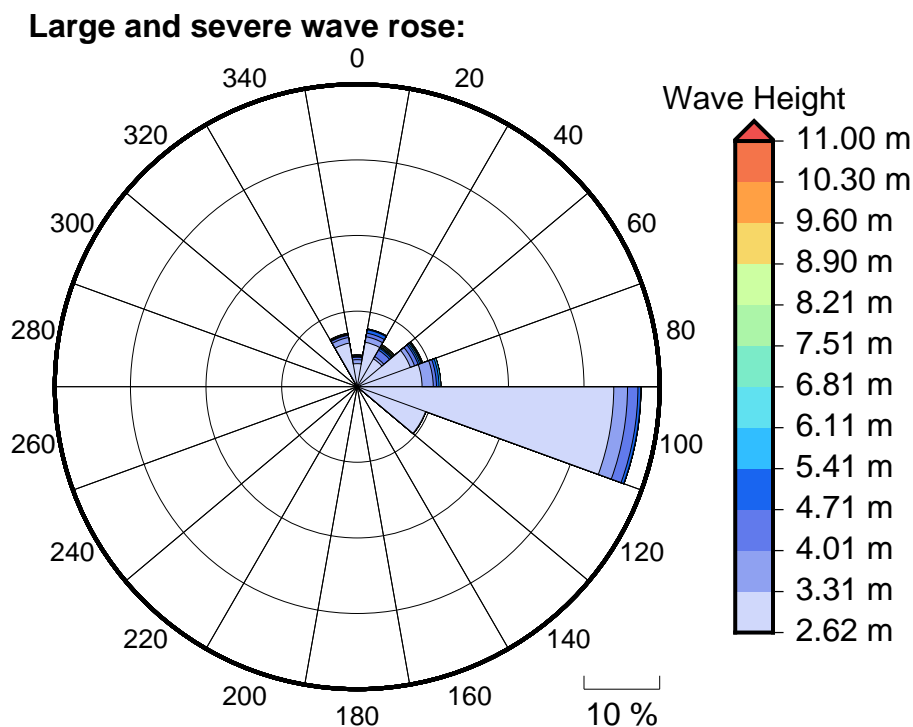
Figure 6 Large, severe and extreme wave roses for Poindimie
