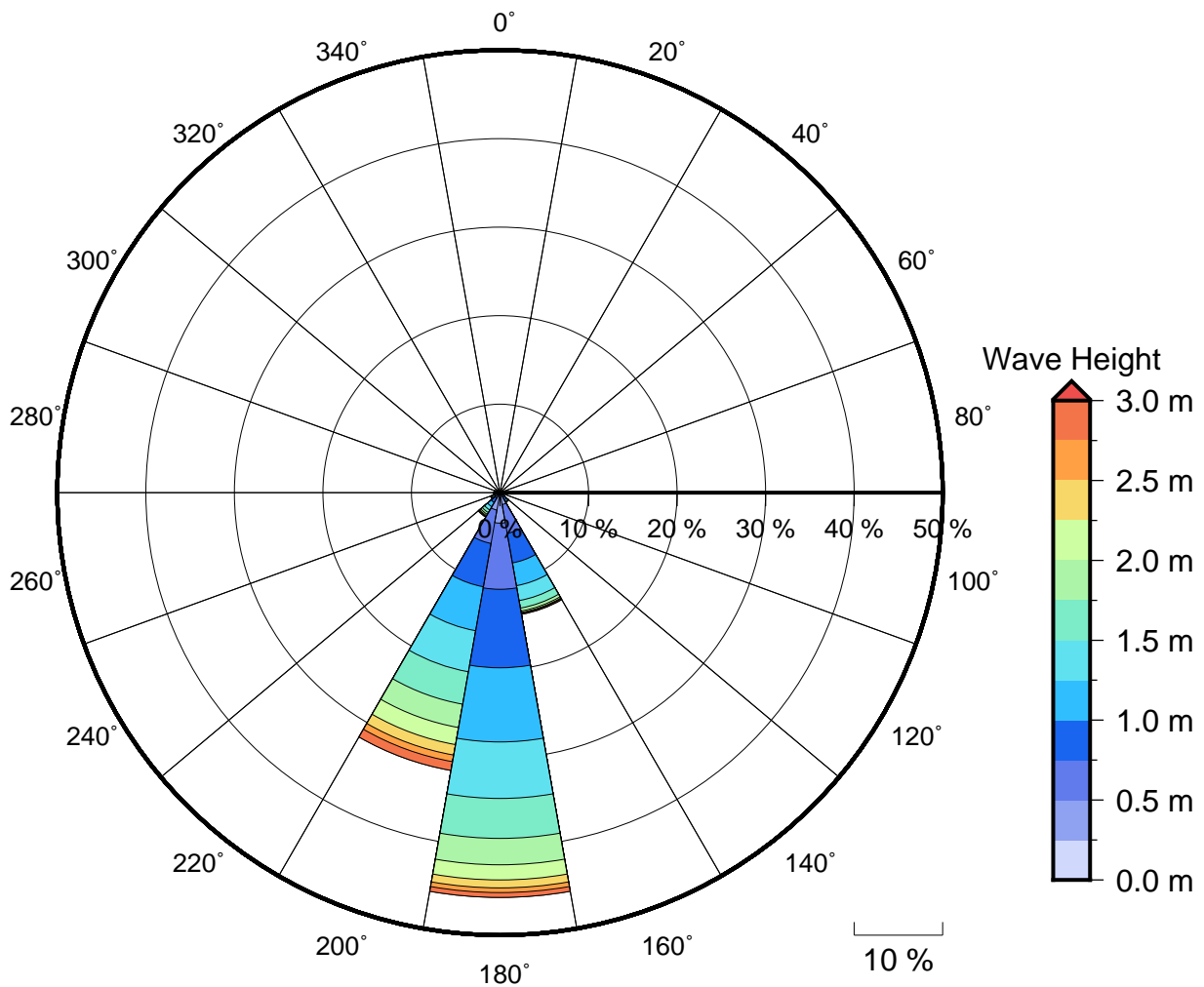
Figure 2 Annual wave rose for Poum. Note that direction are where the wave are coming from.
