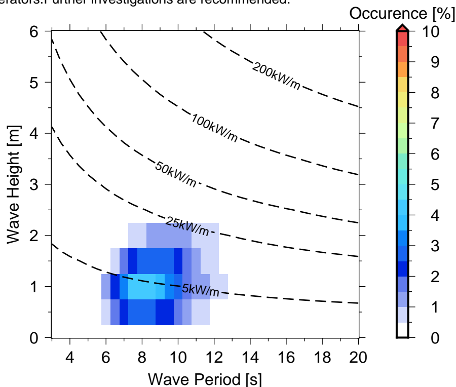
Figure 10 Occurrences of sea states in Poom .
