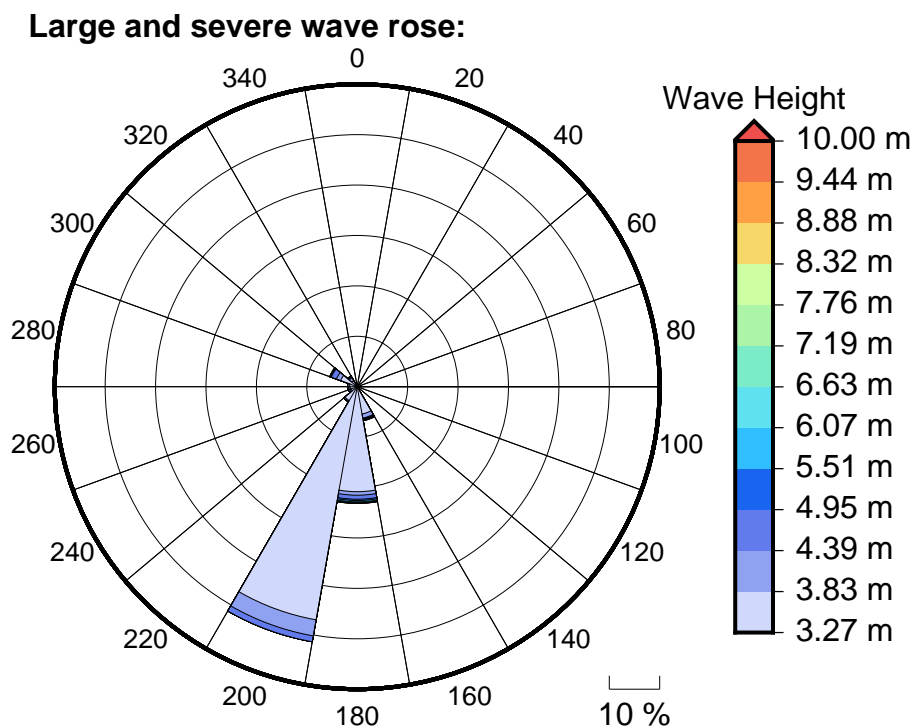
Figure 6 Large, severe and extreme wave roses for Poom
