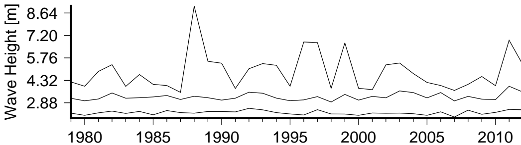
Figure 8 Annual variation in large waves (90th percentile)(lower curve), severe waves (99th percentile) (middle curve) and the largest wave(upper curve) in Poom.
