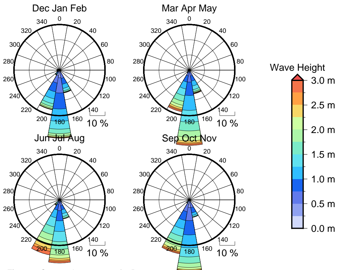
Figure 3 Seasonal wave roses for Poum
