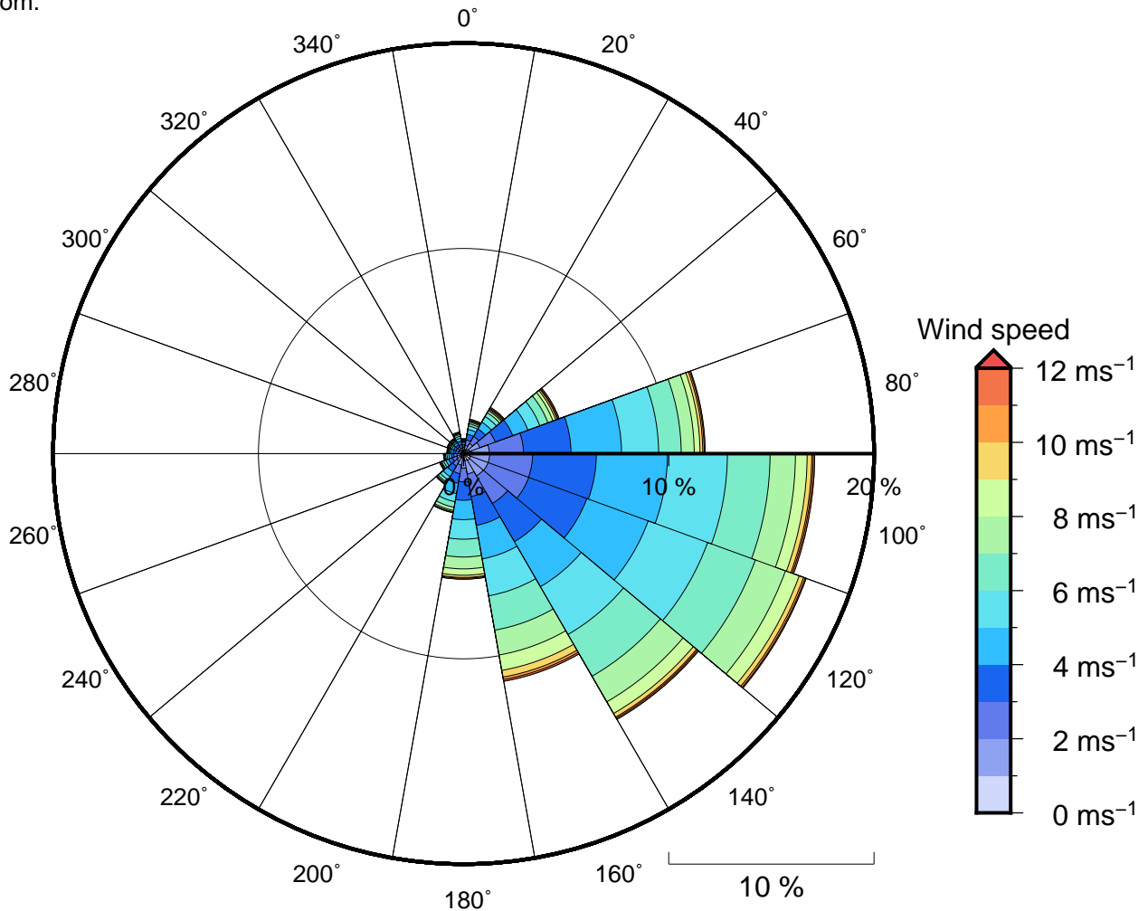
Figure 11 Annual wind rose for Poom. Note that directions are where the wind is coming from .
