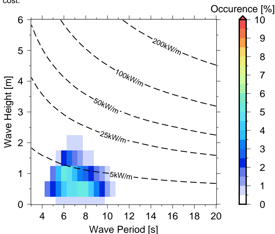
Figure 10 Occurrences of sea states in Thio .
