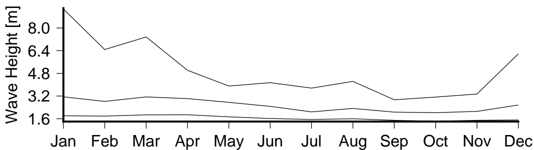
Figure 7 Monthly variation in large waves (90th percentile)(lower curve), severe waves (99th percentile) (middle curve) and the largest wave(upper curve) in Thio.
