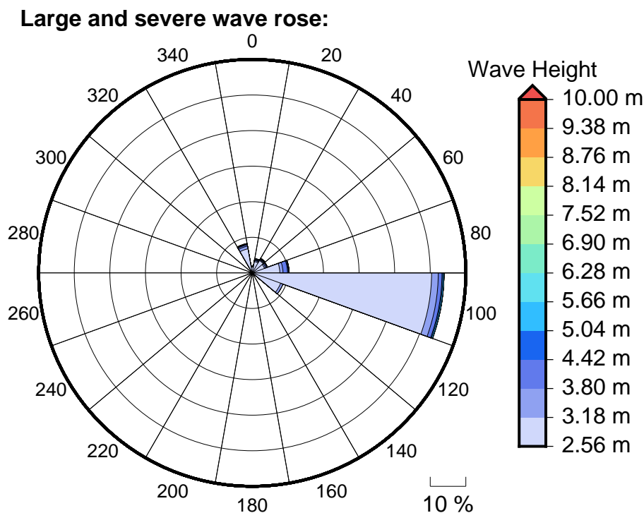
Figure 6 Large, severe and extreme wave roses for Thio
