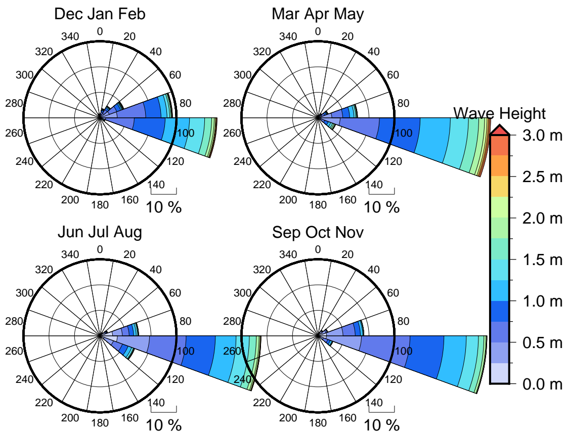
Figure 3 Seasonal wave roses for Thio
