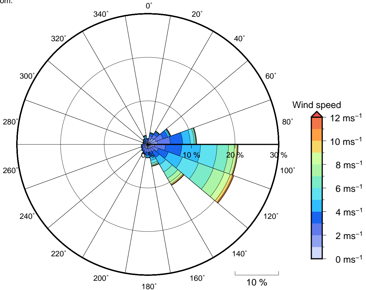
Figure 11 Annual wind rose for Thio. Note that directions are where the wind is coming from.
