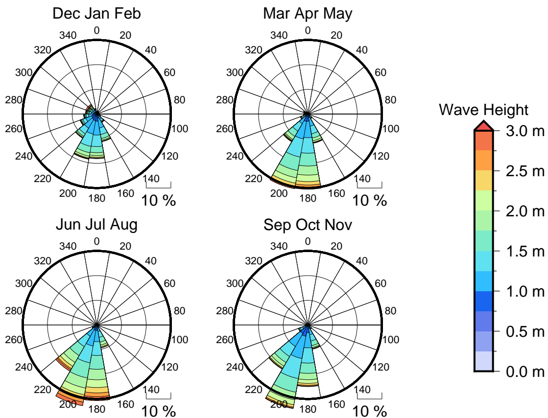
Figure 3 Seasonal wave roses for Niue
