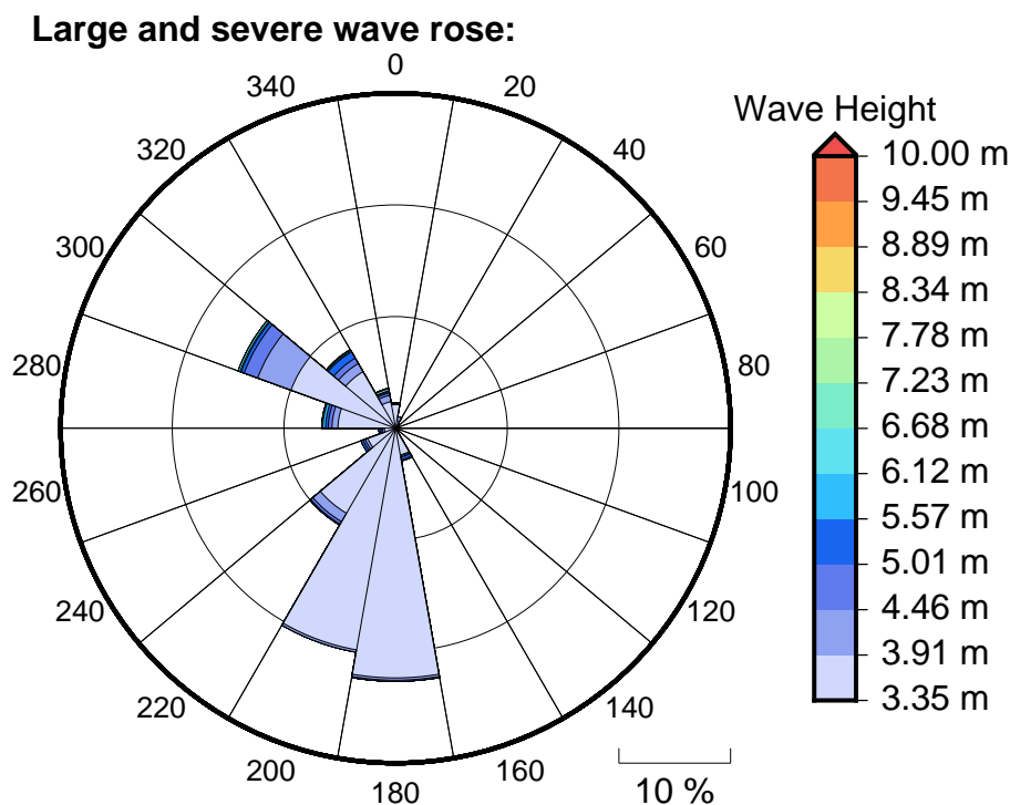
Figure 6 Large, severe and extreme wave roses for Niue
