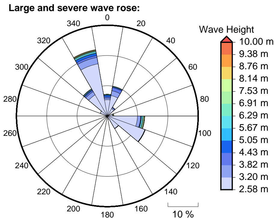
Figure 6 Large, severe and extreme wave roses for Bora Bora
