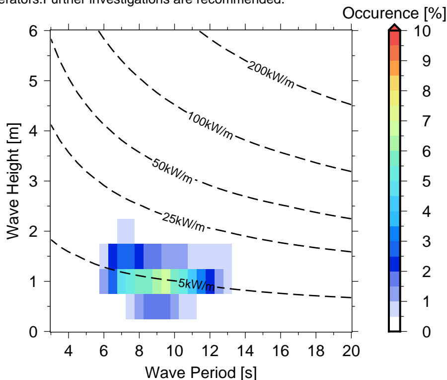
Figure 10 Occurrences of sea states in Bora Bora .
