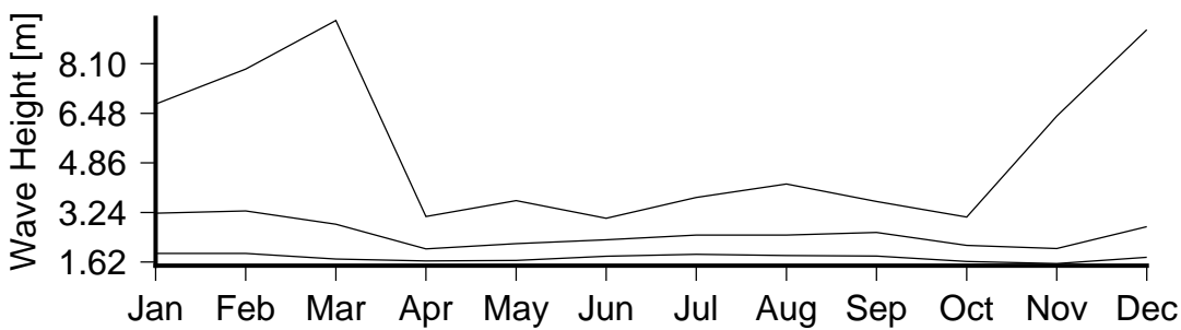
Figure 7 Monthly variation in large waves (90th percentile)(lower curve), severe waves (99th percentile) (middle curve) and the largest wave(upper curve) in Bora Bora.
