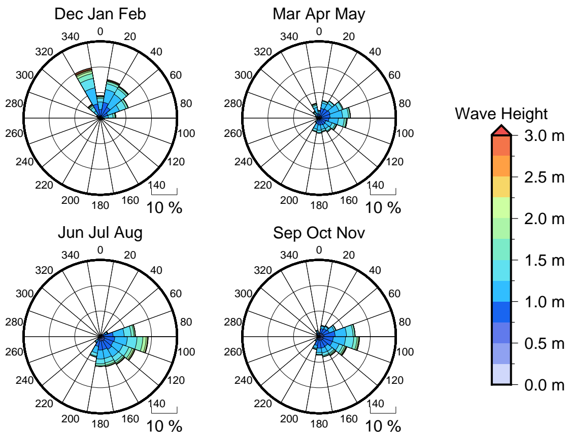
Figure 3 Seasonal wave roses for Bora Bora
