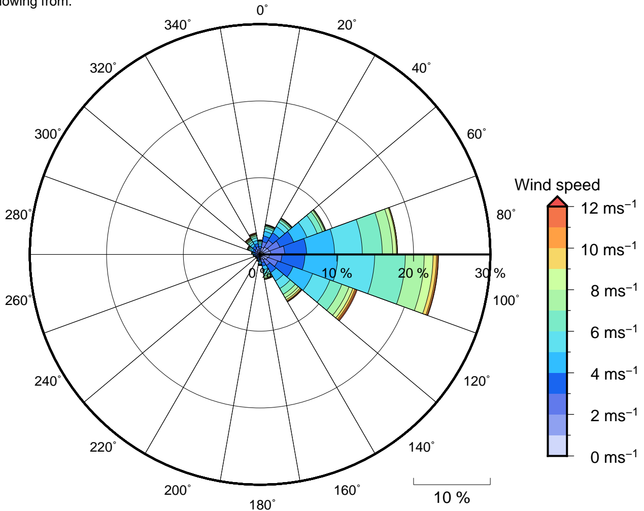
Figure 11 Annual wind rose for Bora Bora. Note that directions are where the wind is coming from .
