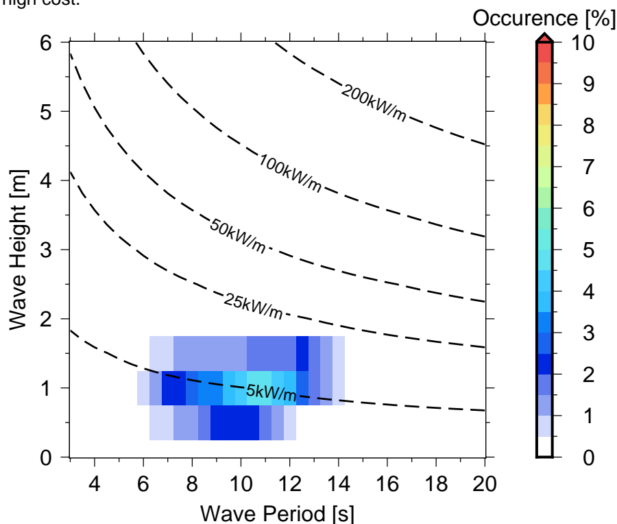
Figure 10 Occurrences of sea states in Fakarava .
