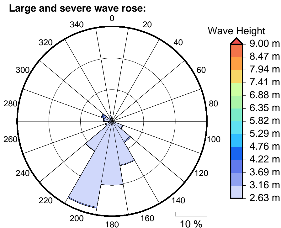
Figure 6 Large, severe and extreme wave roses for Fakarava
