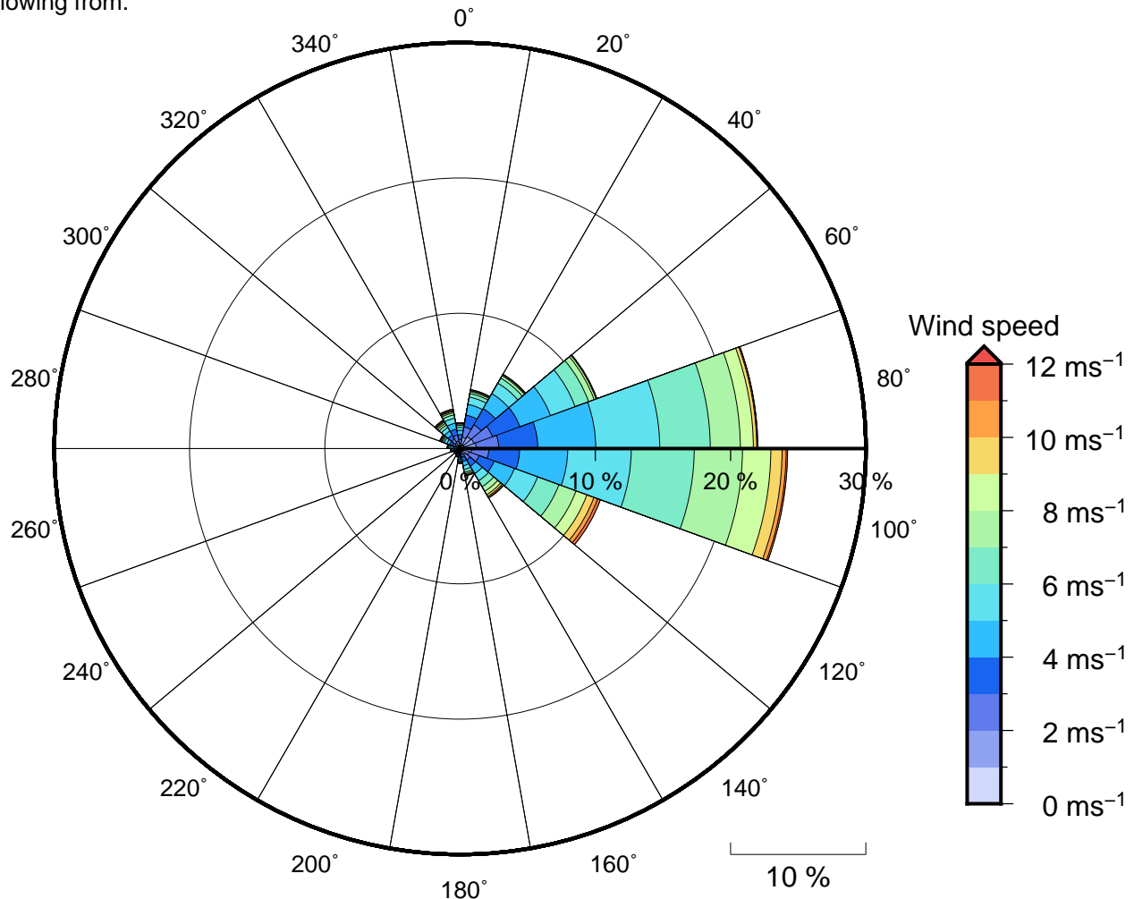
Figure 11 Annual wind rose for Fakarava. Note that directions are where the wind is coming from.
