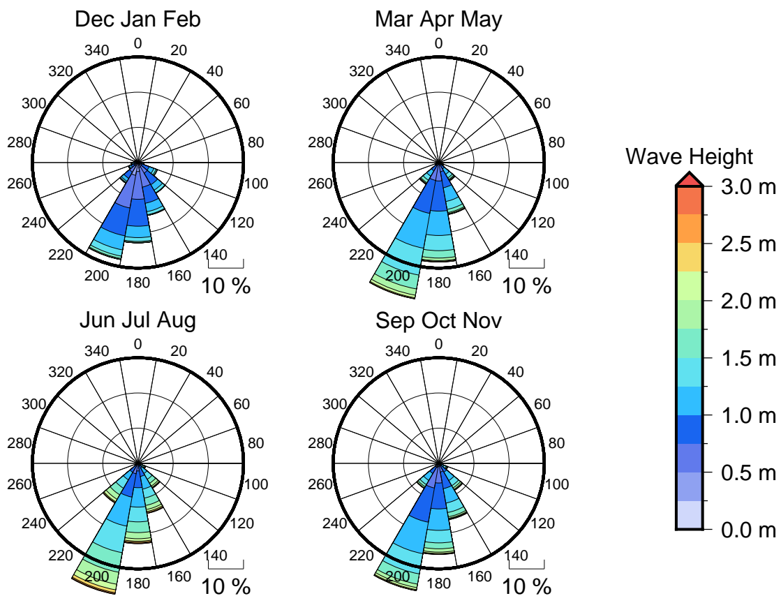
Figure 3 Seasonal wave roses for Fakarava
