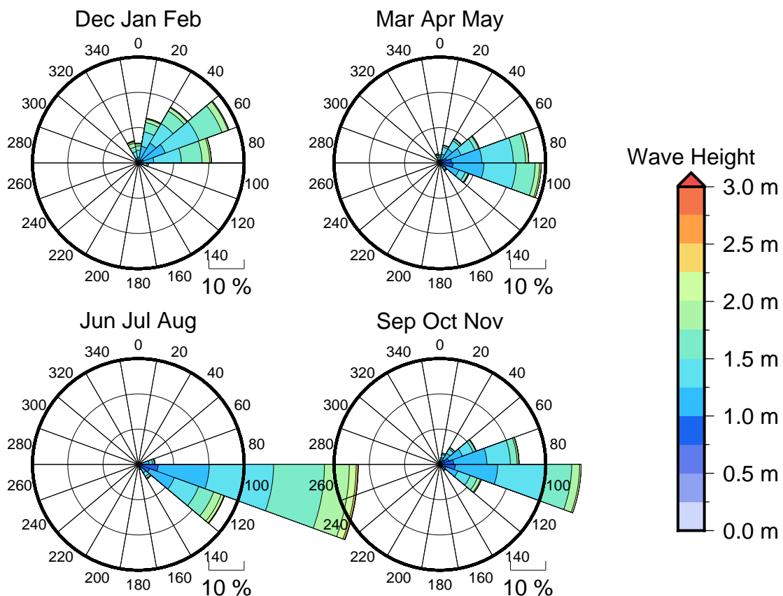
Figure 3 Seasonal wave roses for Nuku Hiva
