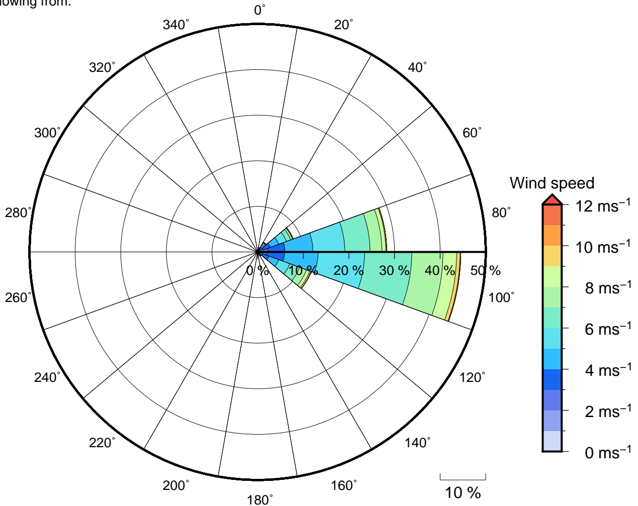
Figure 11 Annual wind rose for Nuku Hiva. Note that directions are where the wind is coming from.
