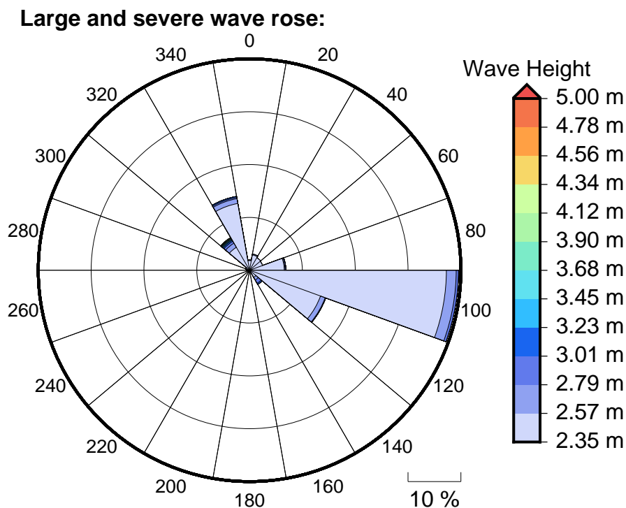
Figure 6 Large, severe and extreme wave roses for Nuku Hiva
