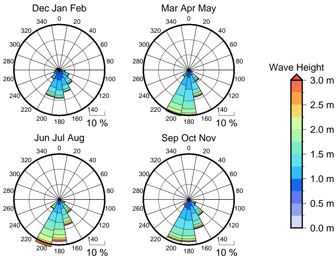
Figure 3 Seasonal wave roses for Papeete
