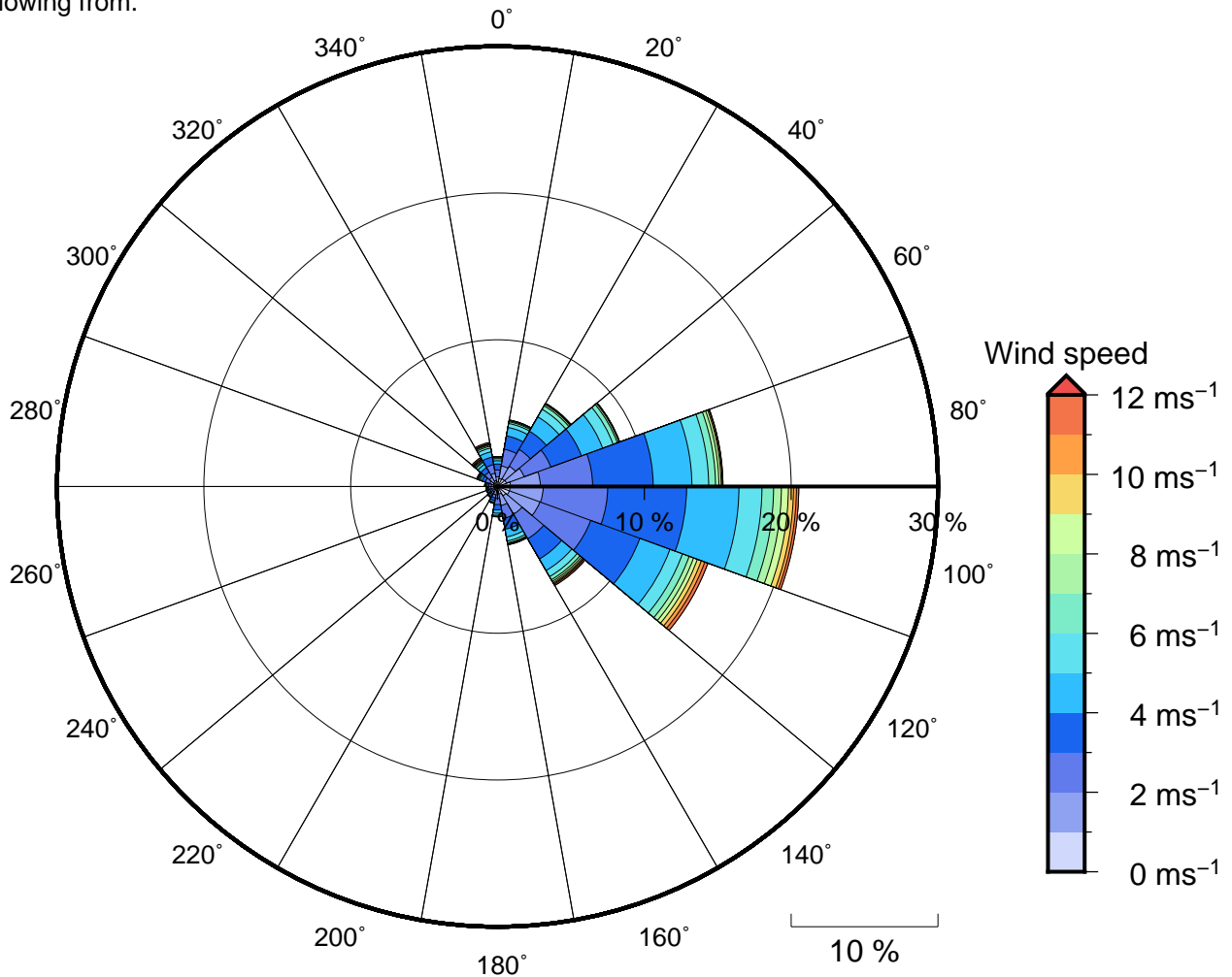
Figure 11 Annual wind rose for Papeete. Note that directions are where the wind is coming from .
