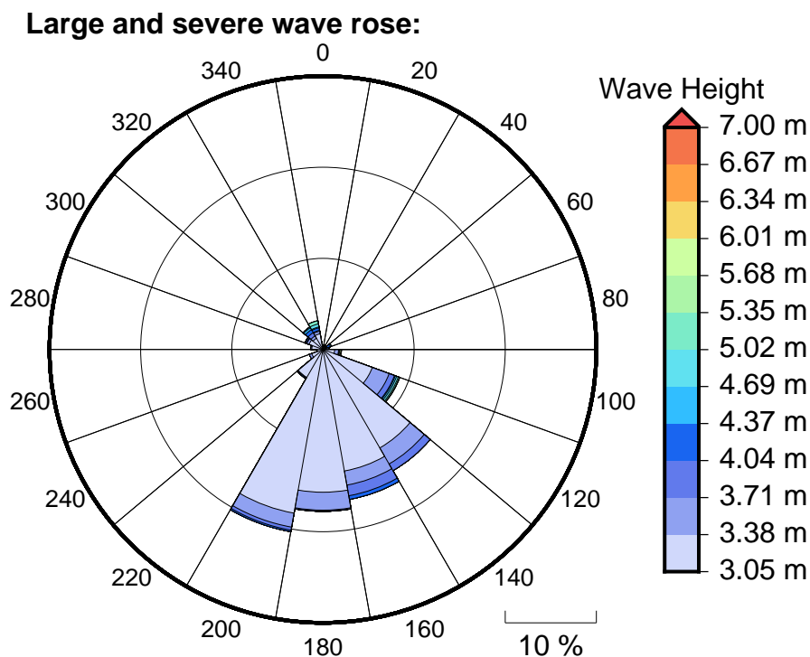
Figure 6 Large, severe and extreme wave roses for Papeete
