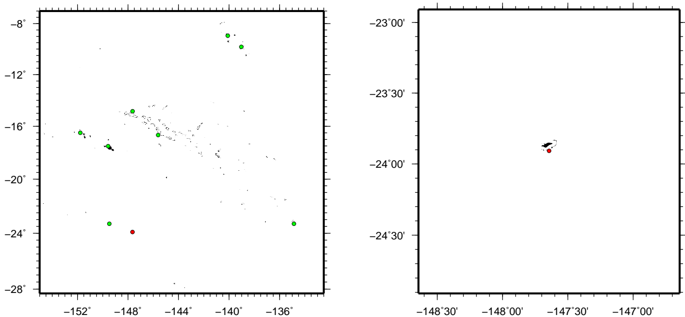
Figure 1. Location maps of the site. The map on the left shows the region. The map on the right shows the island and its surroundings. The red point shows to the actual site and green points (if present) indicate other available wave climate reports in the region.
