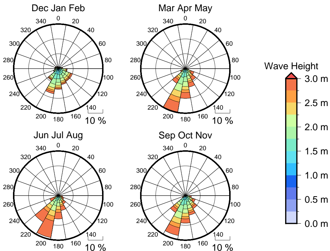
Figure 3 Seasonal wave roses for Raivavae
