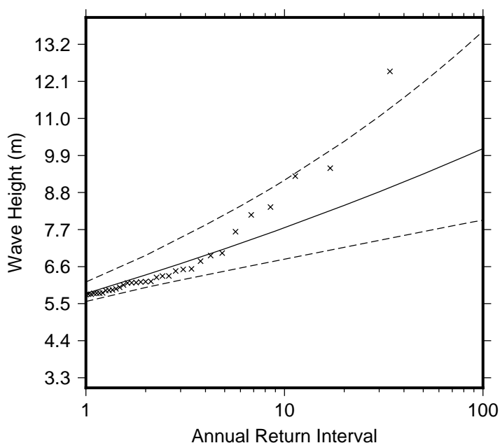
Figure 9 Extreme wave distribution for Raivavae. The crosses represents the wave events that occurred since 1979. The plain line is the statistical distribution that best fit the past wave events. The dotted line show the upper and lower high confidence of the fit, there is a 95% chance that the fitted distribution lie between the two dashed lines.
