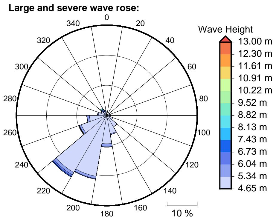
Figure 6 Large, severe and extreme wave roses for Raivavae
