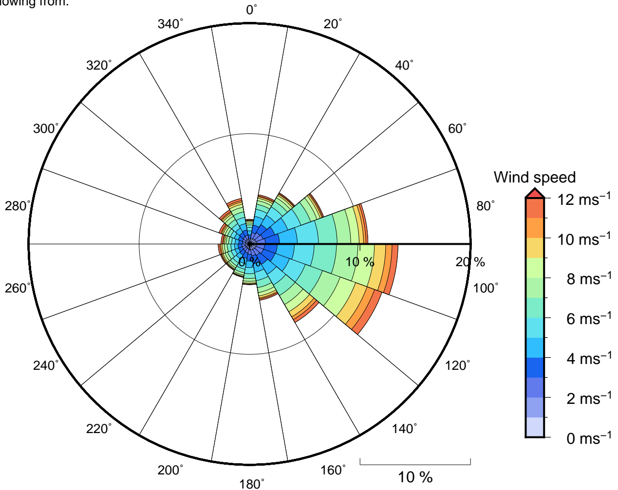
Figure 11 Annual wind rose for Raivavae. Note that directions are where the wind is coming from.
