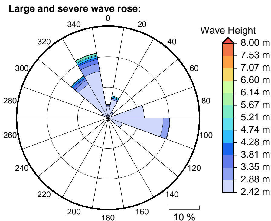
Figure 6 Large, severe and extreme wave roses for Rangiroa
