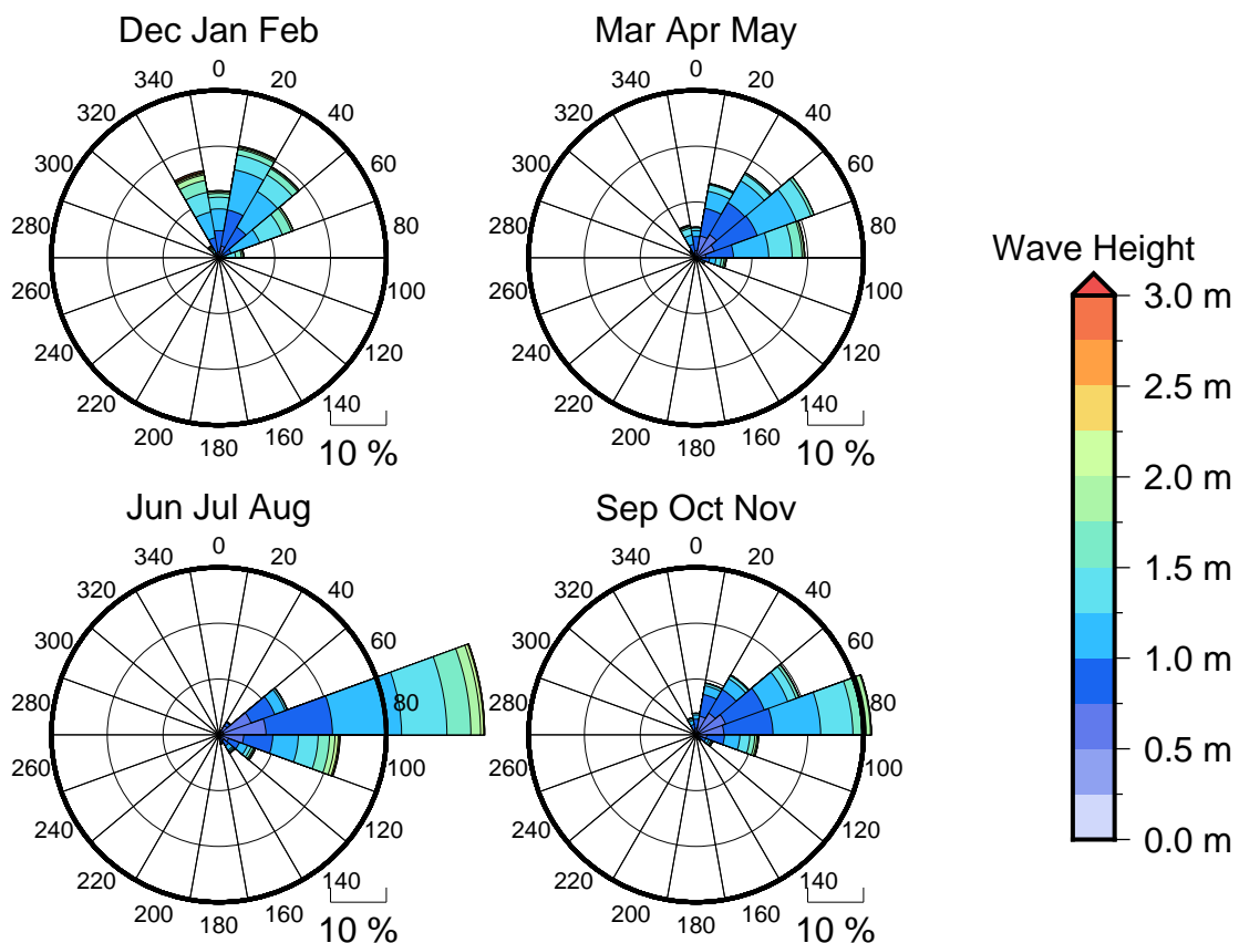
Figure 3 Seasonal wave roses for Rangiroa
