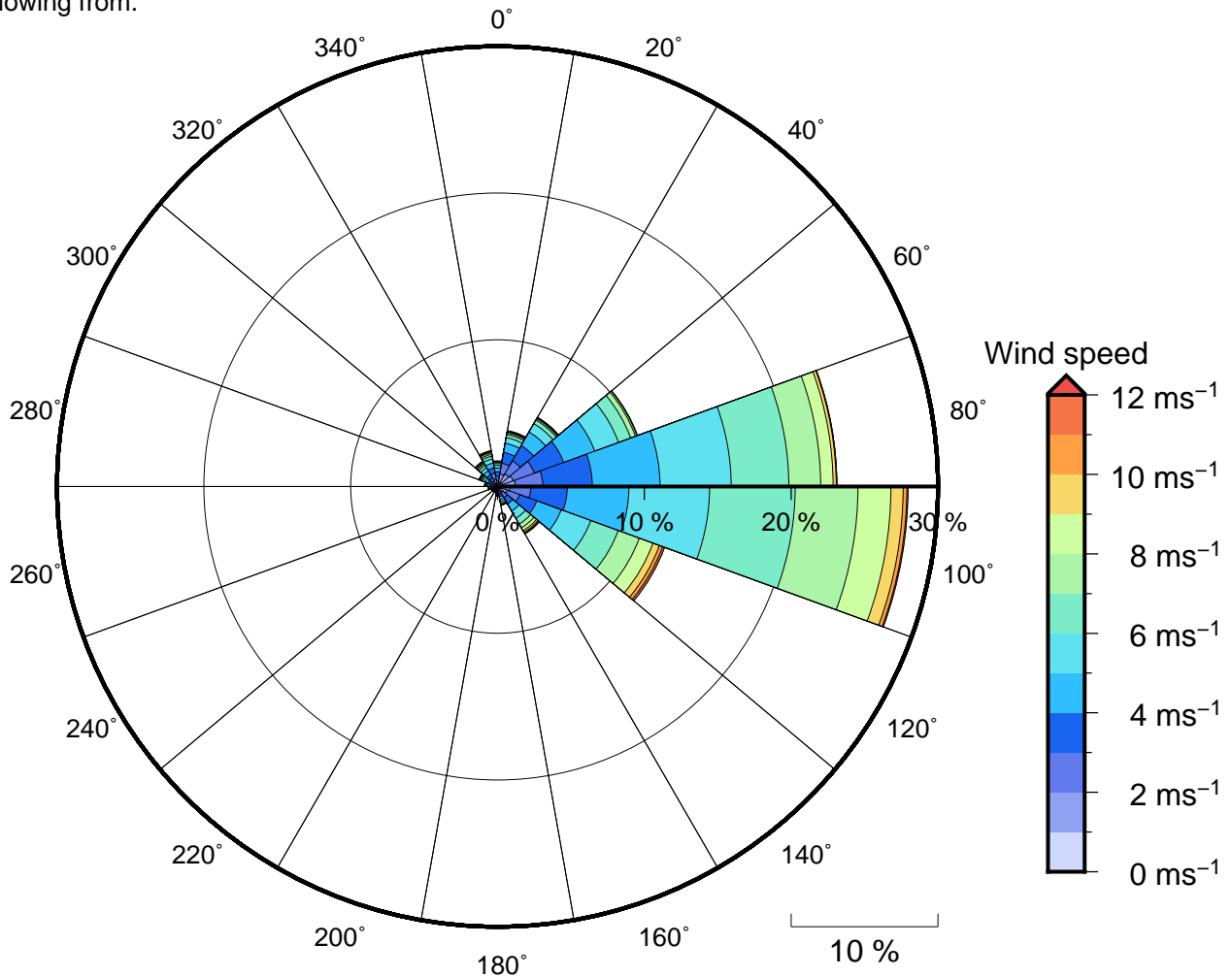
Figure 11 Annual wind rose for Rangiroa. Note that directions are where the wind is coming from.
