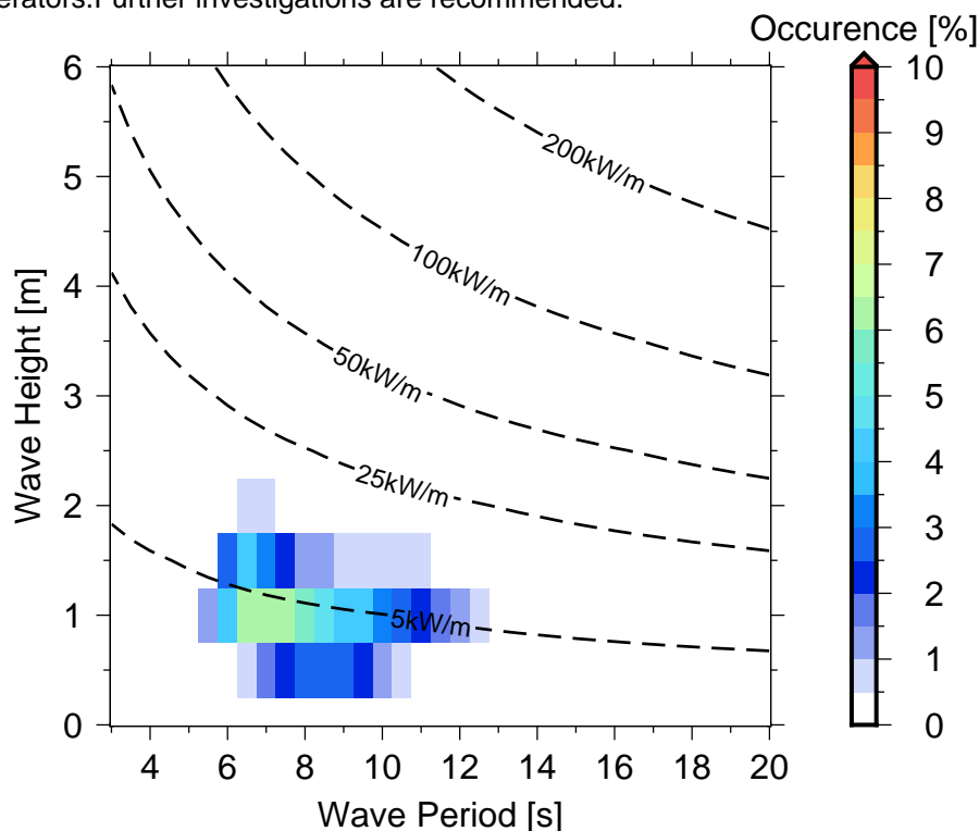
Figure 10 Occurrences of sea states in Rangiroa .
