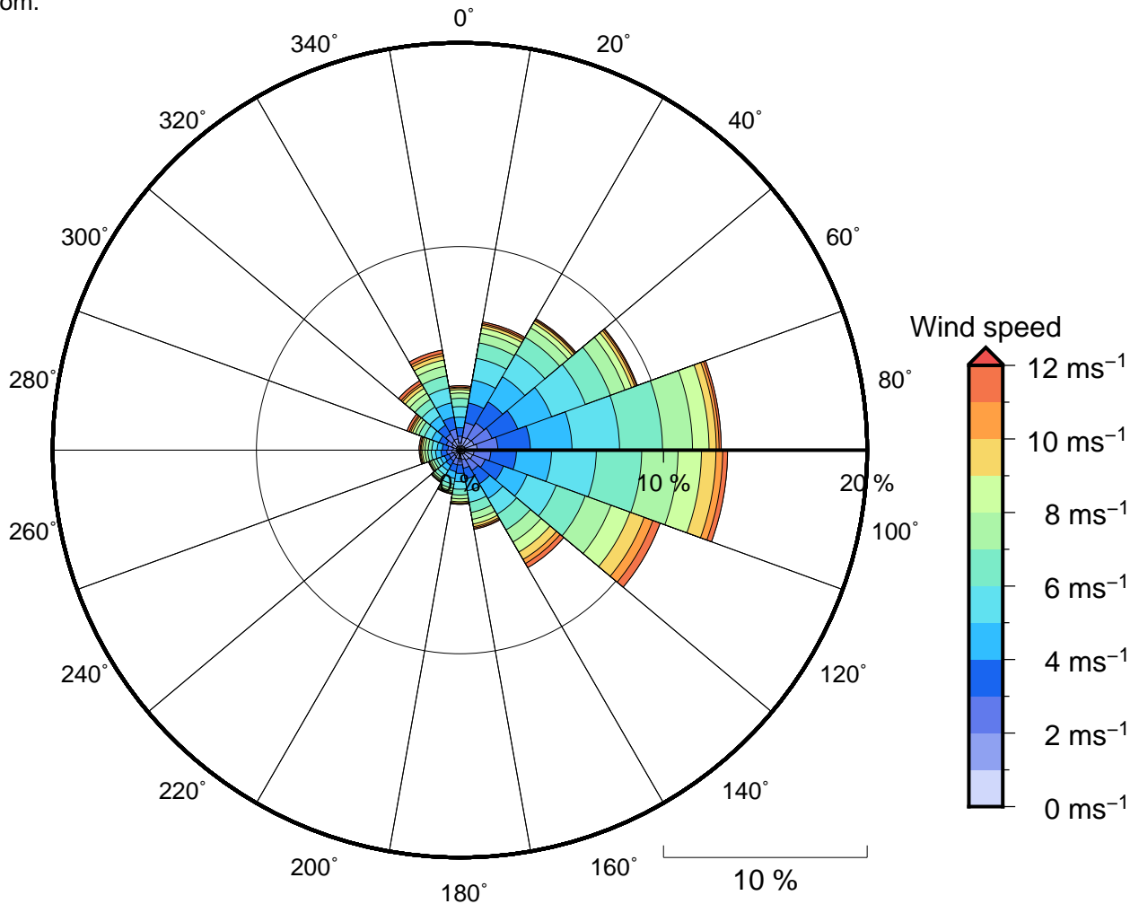
Figure 11 Annual wind rose for Rikitea. Note that directions are where the wind is coming from.
