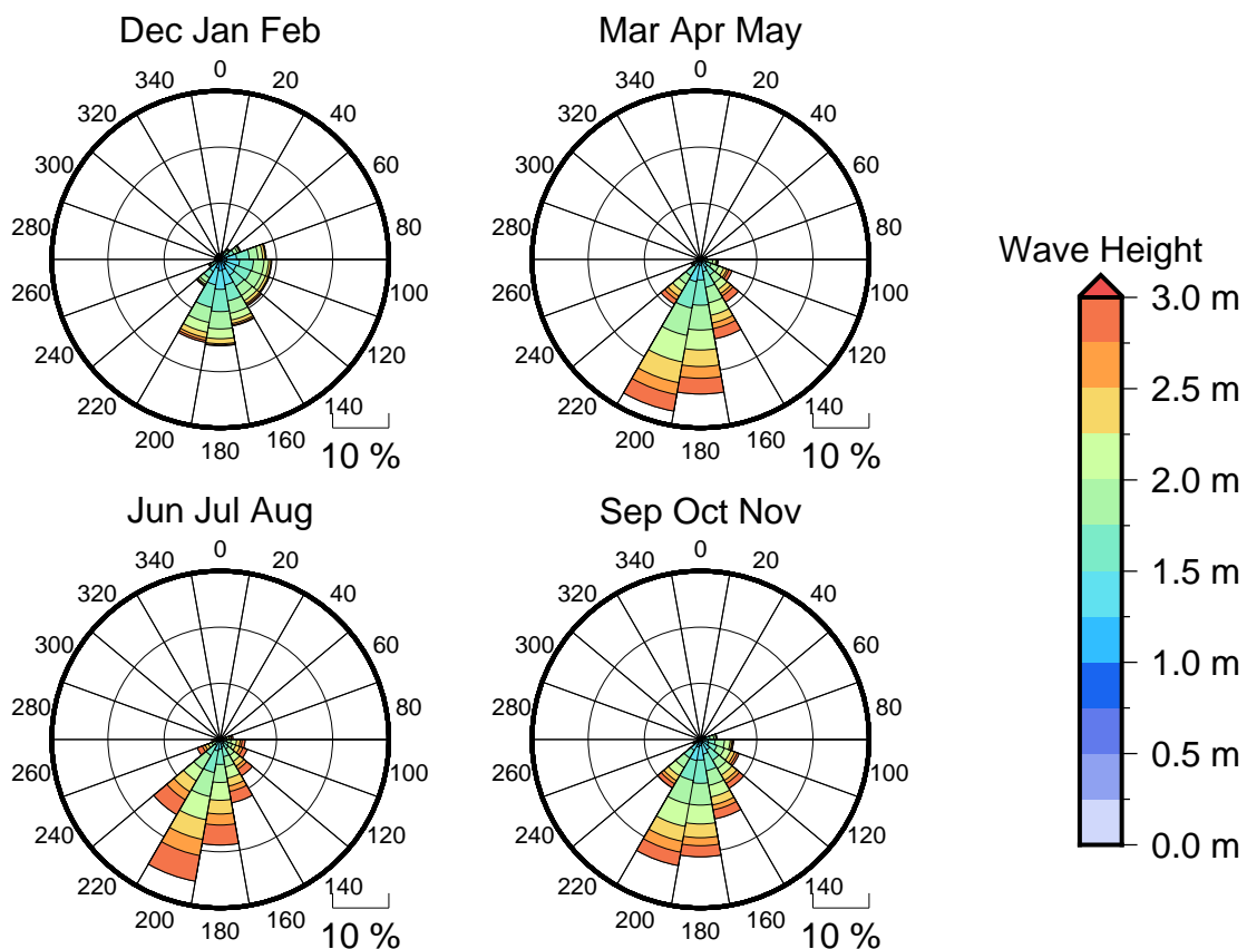
Figure 3 Seasonal wave roses for Rikitea
