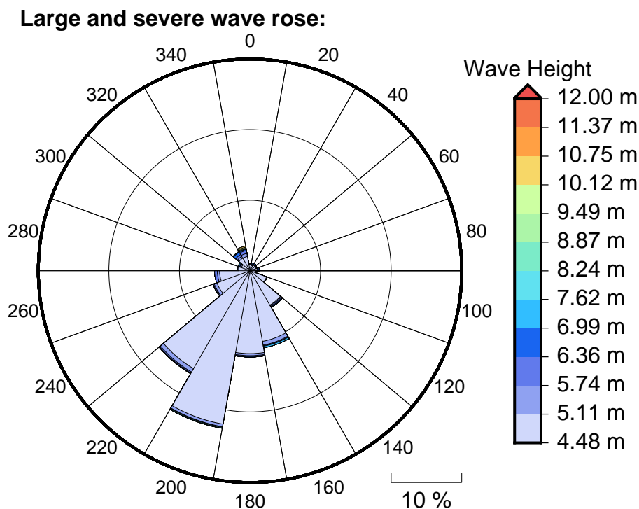
Figure 6 Large, severe and extreme wave roses for Rimatara
