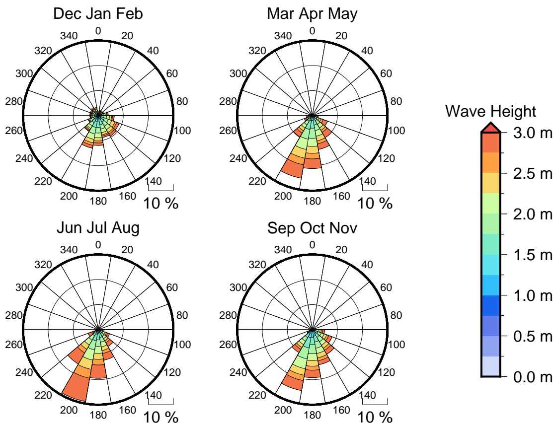
Figure 3 Seasonal wave roses for Rimatara
