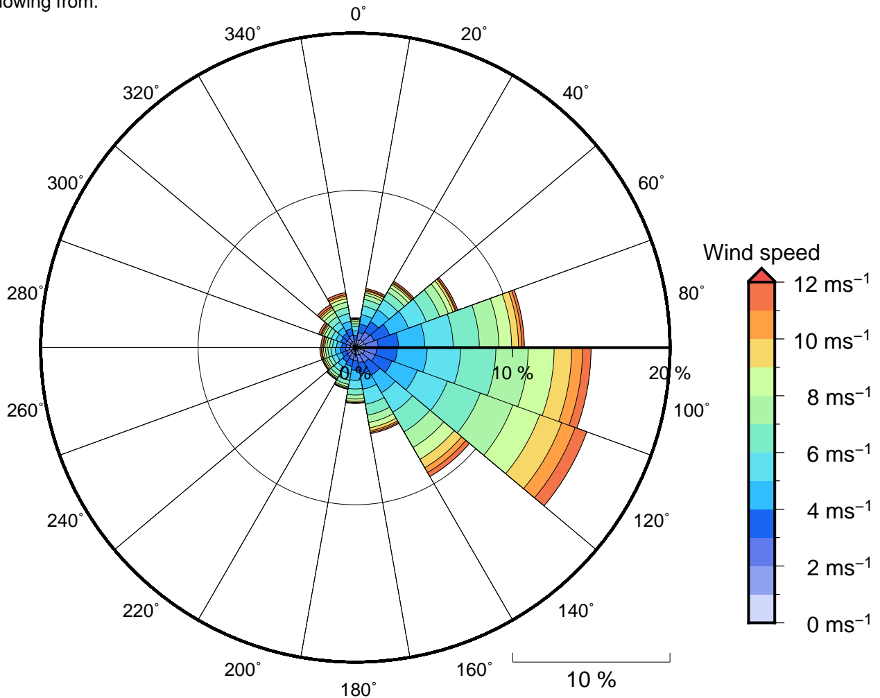
Figure 11 Annual wind rose for Rimatara. Note that directions are where the wind is coming from.
