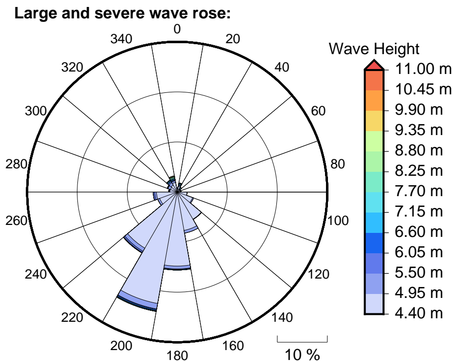
Figure 6 Large, severe and extreme wave roses for Rurutu
