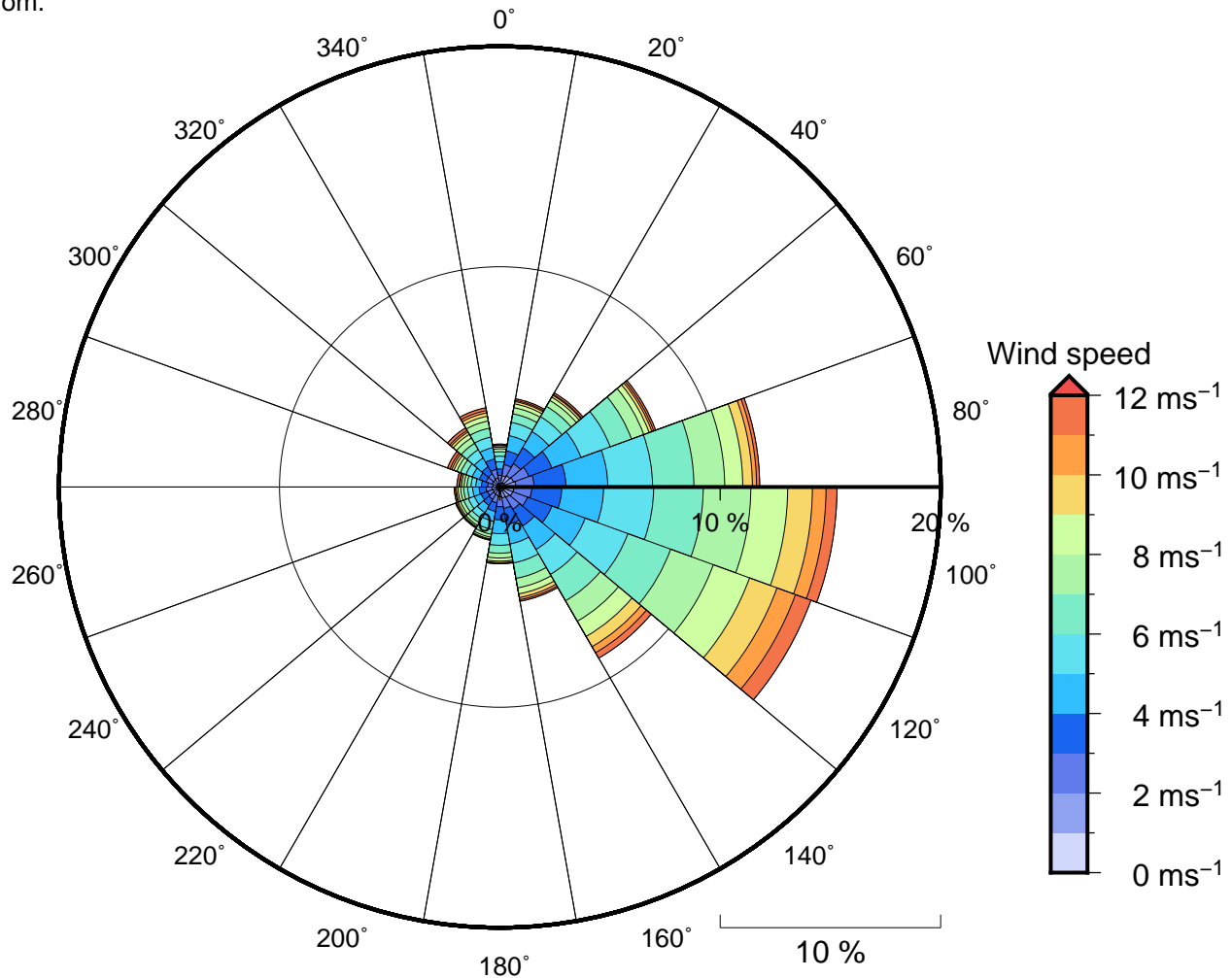
Figure 11 Annual wind rose for Rurutu. Note that directions are where the wind is coming from .
