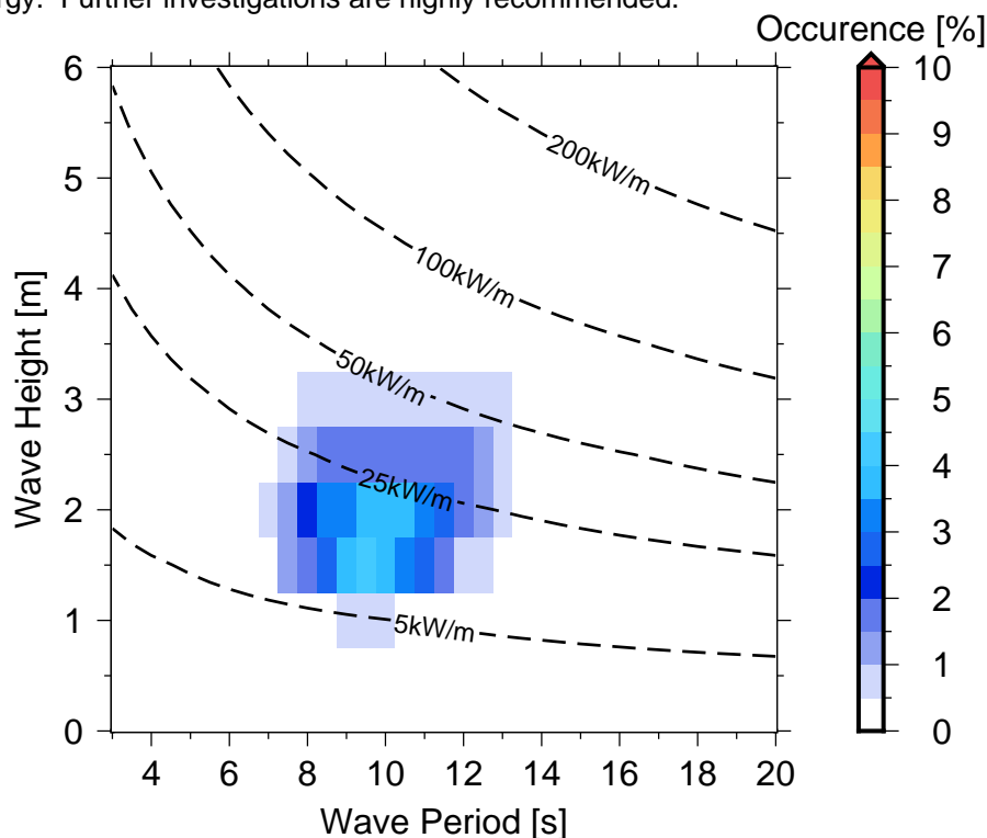
Figure 10 Occurrences of sea states in Rurutu .
