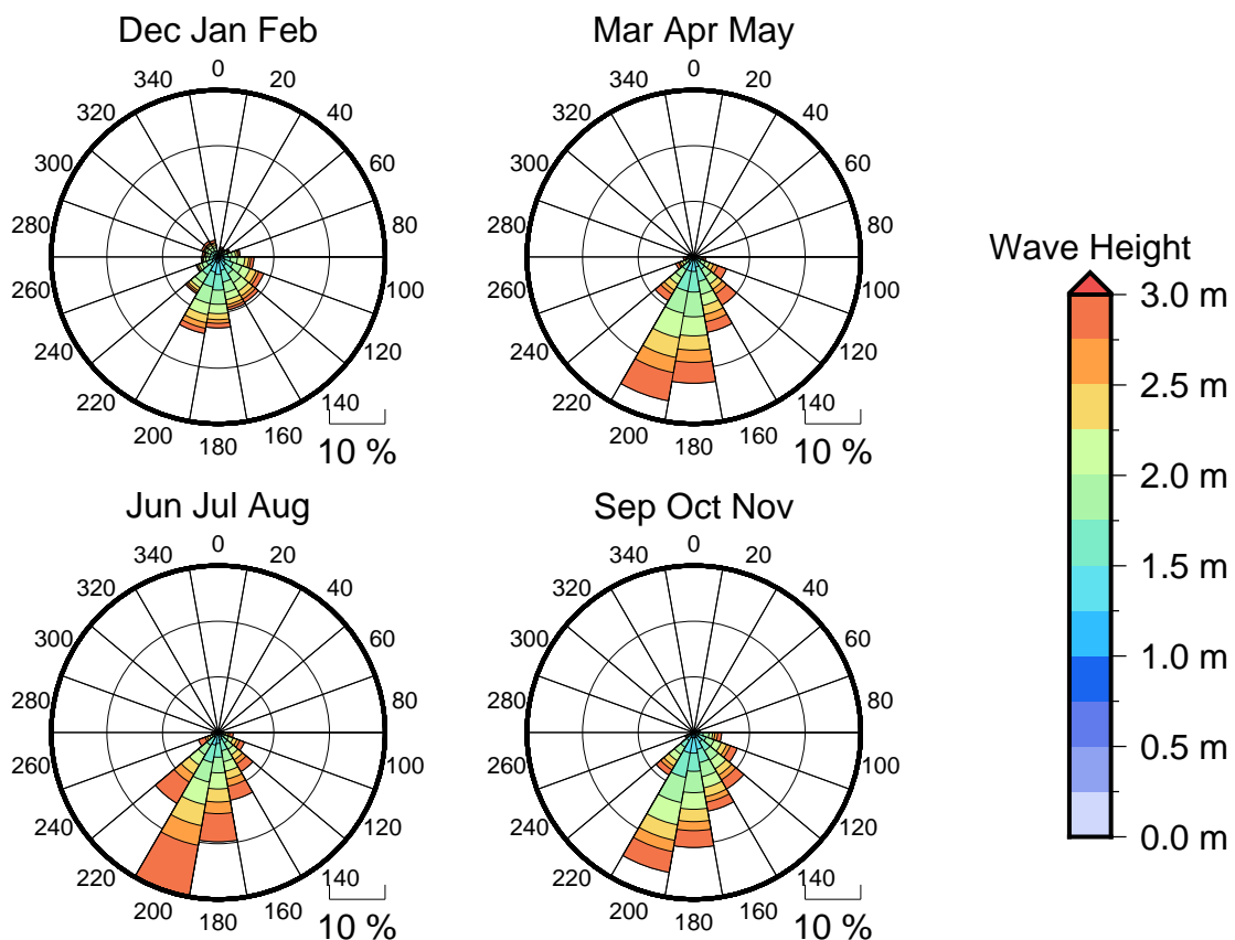
Figure 3 Seasonal wave roses for Rurutu
