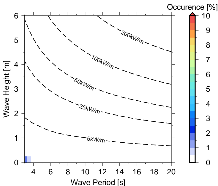
Figure 10 Occurrences of sea states in Alotau .
