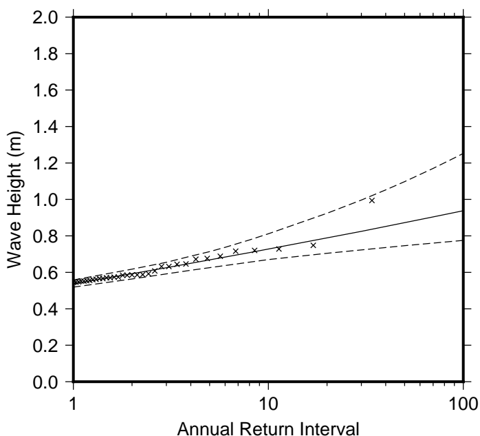
Figure 9 Extreme wave distribution for Alotau. The crosses represents the wave events that occurred since 1979. The plain line is the statistical distribution that best fit the past wave events. The dotted line show the upper and lower high confidence of the fit, there is a 95% chance that the fitted distribution lie between the two dashed lines.
