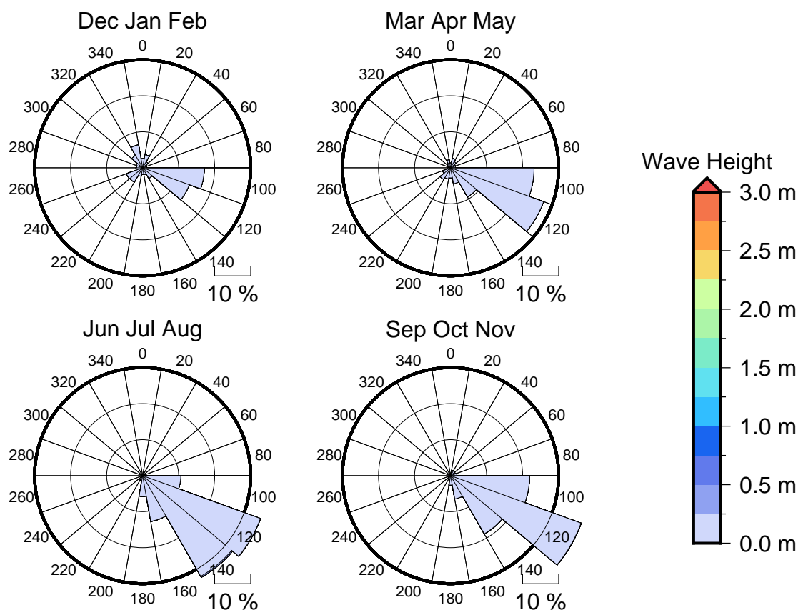
Figure 3 Seasonal wave roses for Alotau
