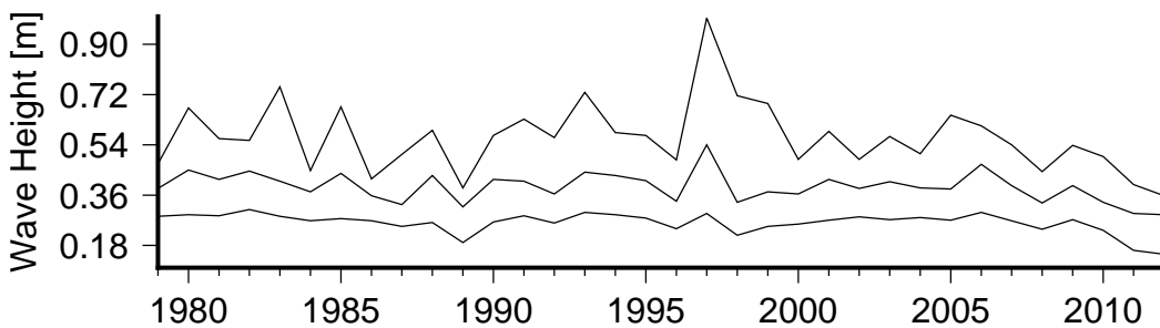
Figure 8 Annual variation in large waves (90th percentile)(lower curve), severe waves (99th percentile) (middle curve) and the largest wave(upper curve) in Alotau.
