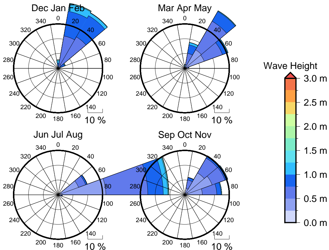
Figure 3 Seasonal wave roses for Arawa
