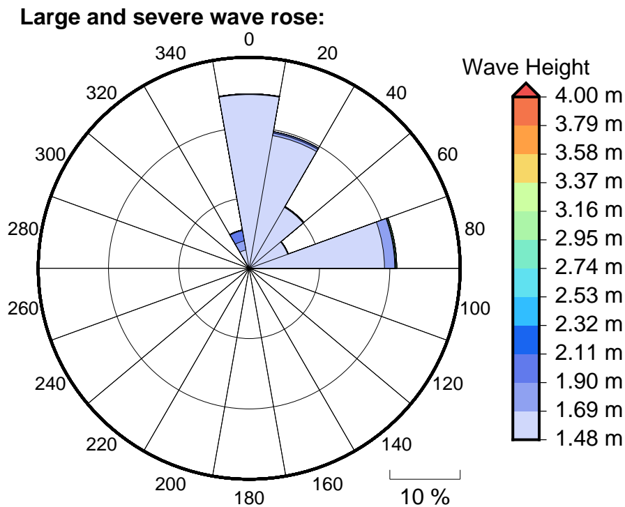
Figure 6 Large, severe and extreme wave roses for Arawa
