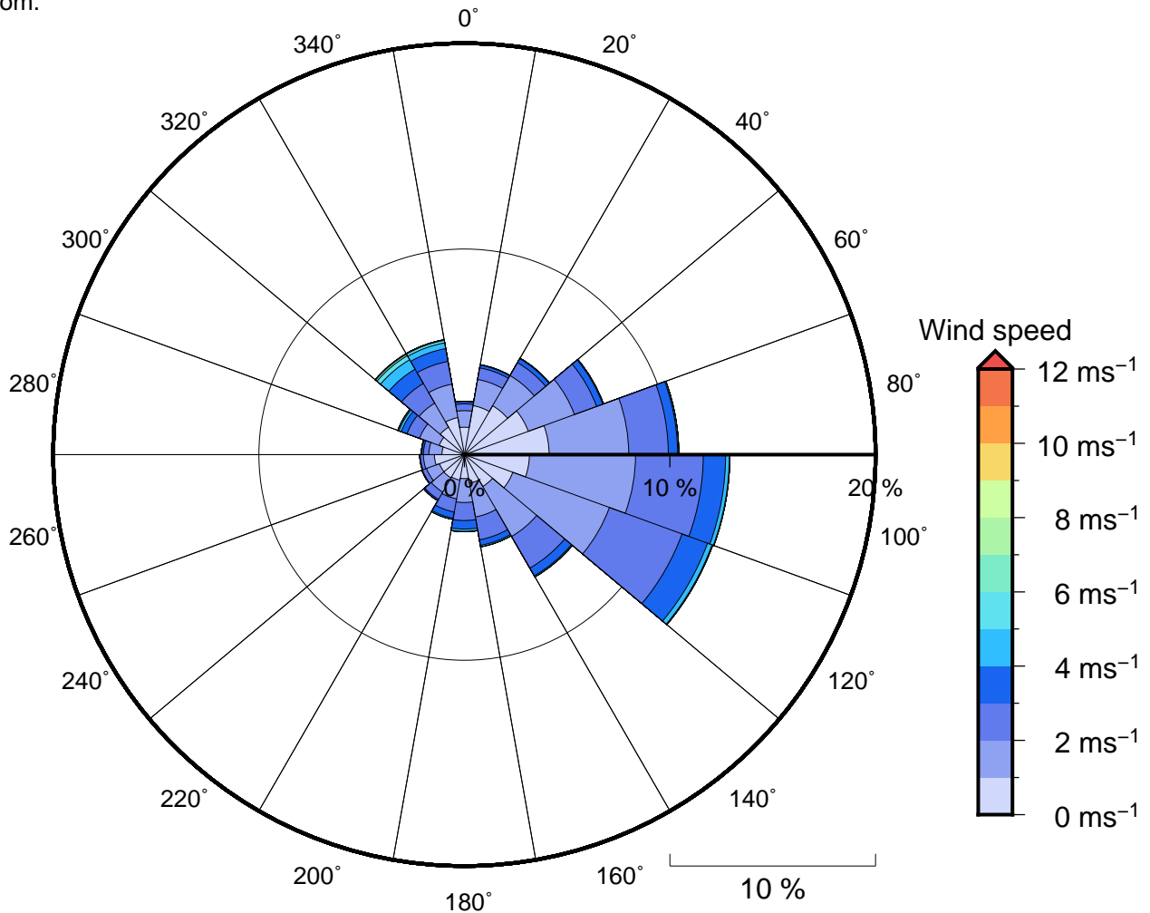
Figure 11 Annual wind rose for Arawa. Note that directions are where the wind is coming from.
