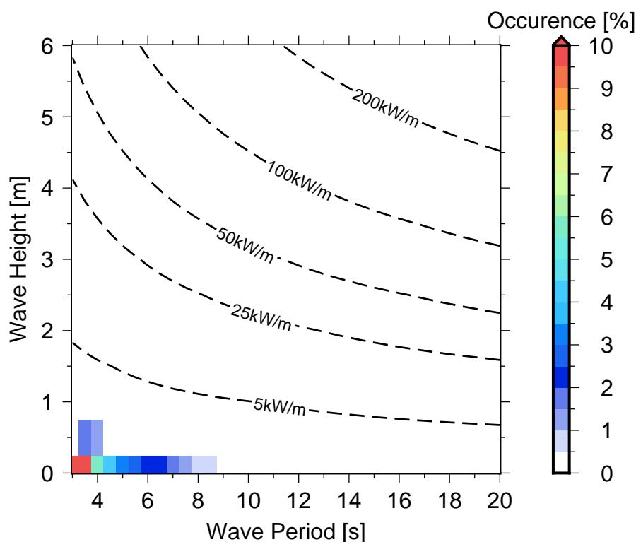
Figure 10 Occurrences of sea states in Daru .
