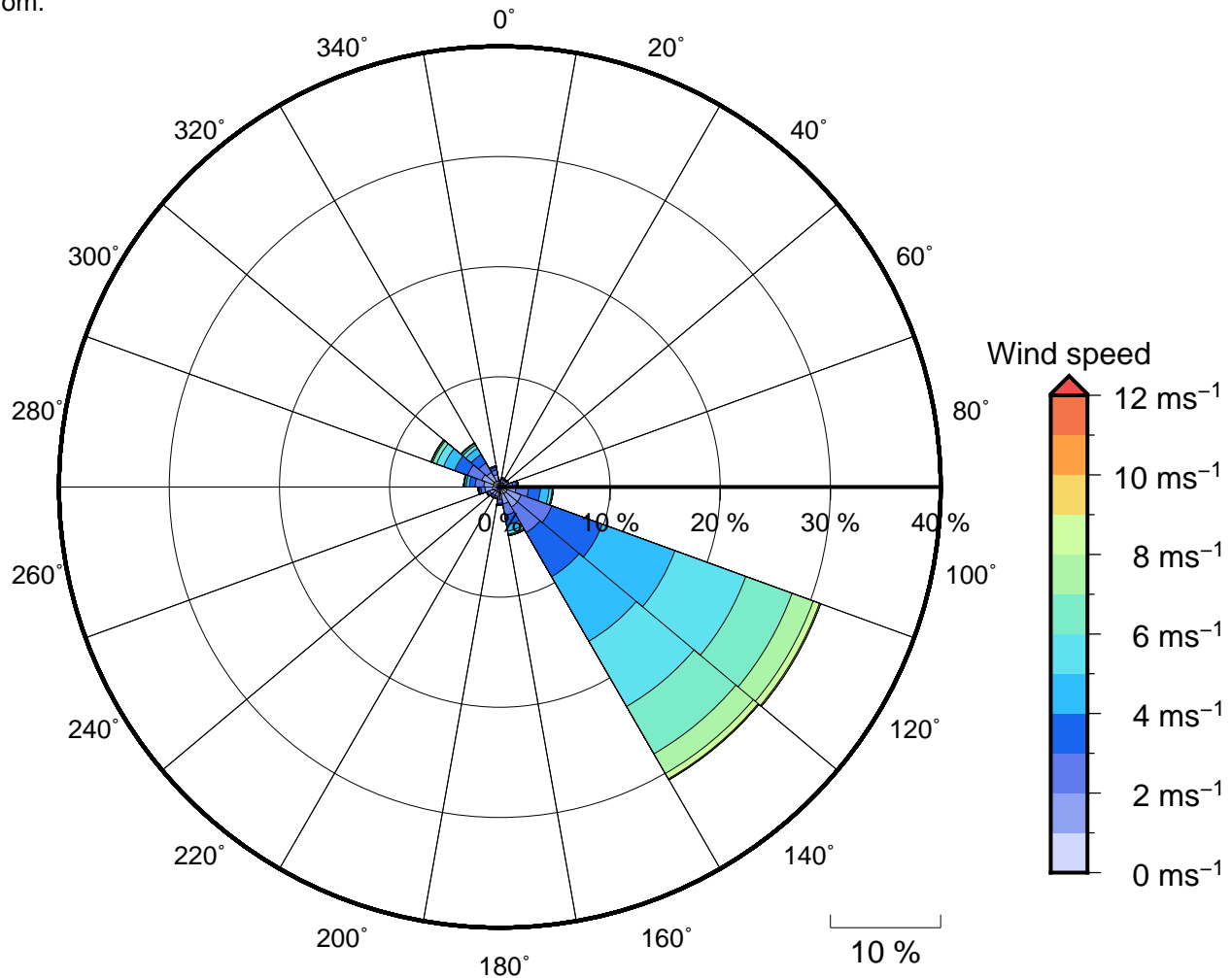
Figure 11 Annual wind rose for Daru. Note that directions are where the wind is coming from .
