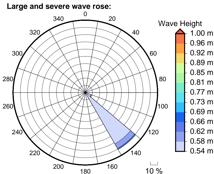
Figure 6 Large, severe and extreme wave roses for Daru
