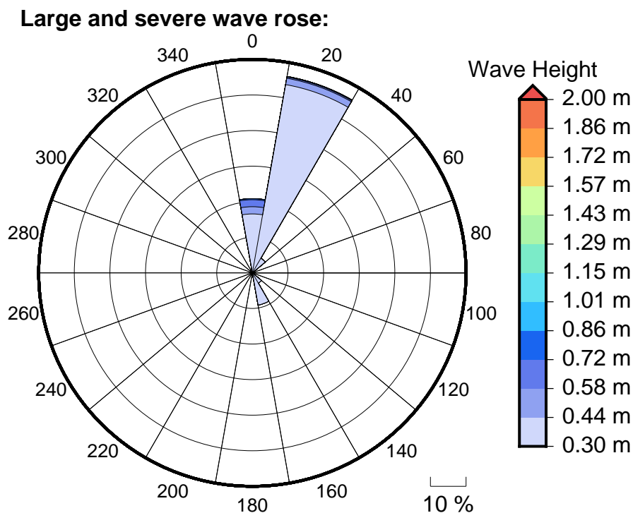
Figure 6 Large, severe and extreme wave roses for Kimbe
