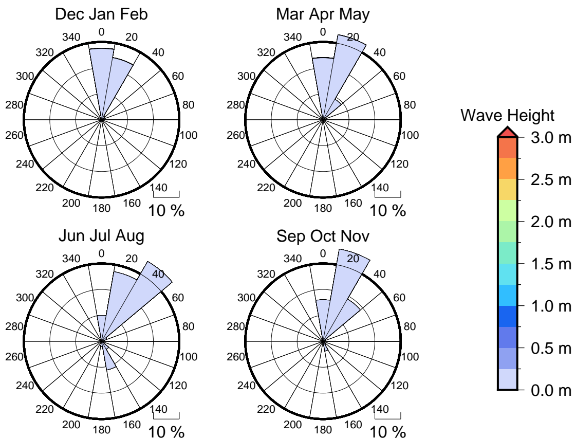
Figure 3 Seasonal wave roses for Kimbe
