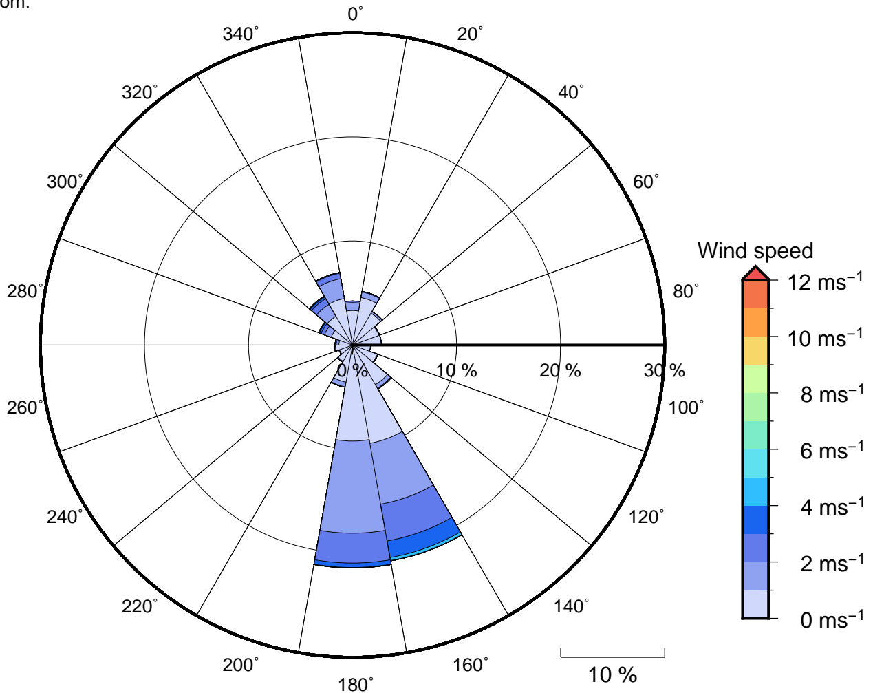
Figure 11 Annual wind rose for Kimbe. Note that directions are where the wind is coming from.
