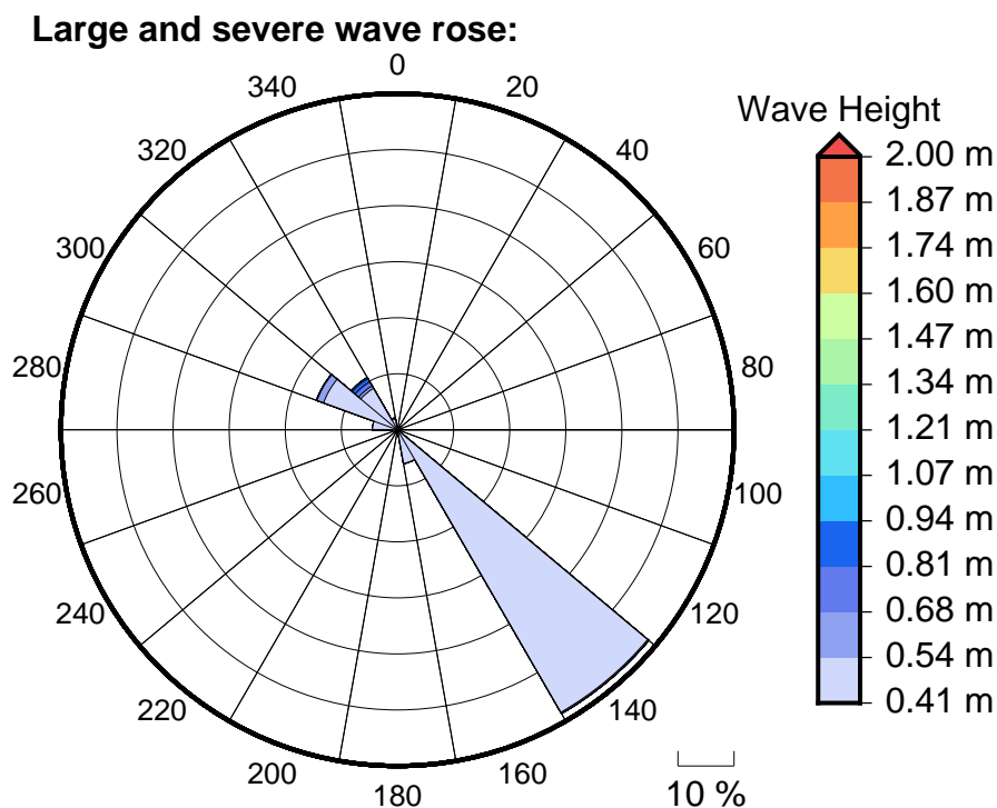
Figure 6 Large, severe and extreme wave roses for Rabaul
