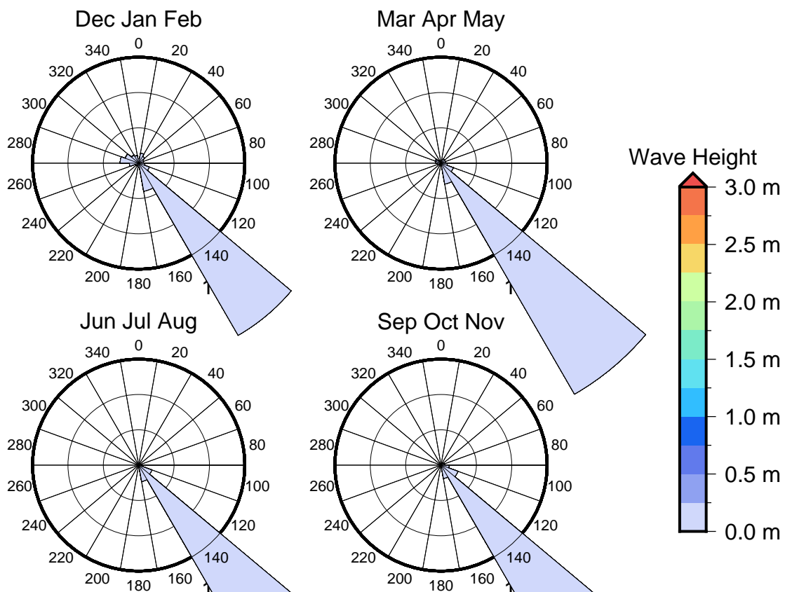
Figure 3 Seasonal wave roses for Rabaul
