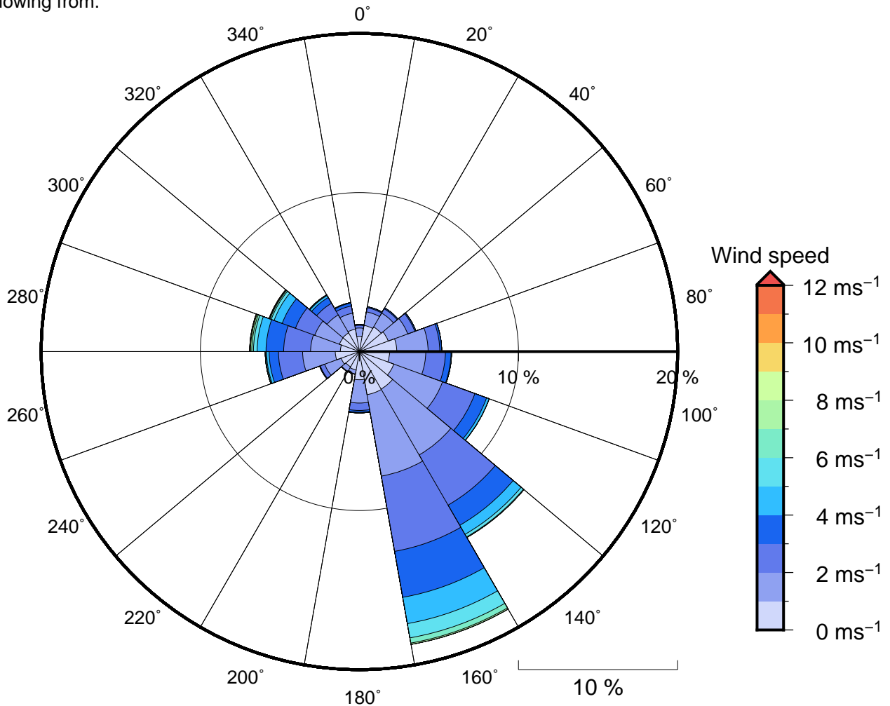
Figure 11 Annual wind rose for Rabaul. Note that directions are where the wind is coming from.
