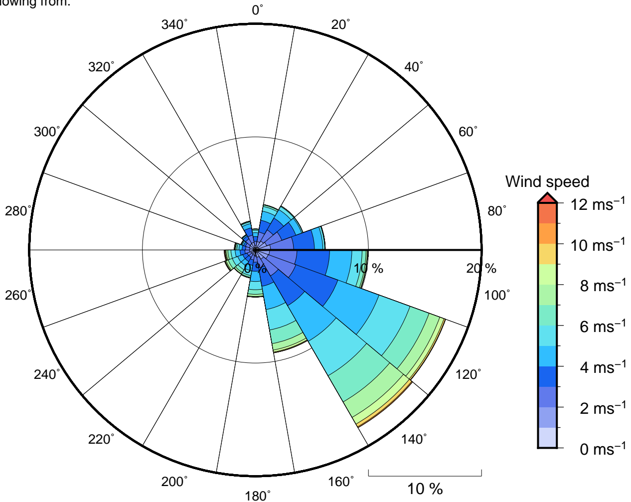
Figure 11 Annual wind rose for Samarai. Note that directions are where the wind is coming from .
