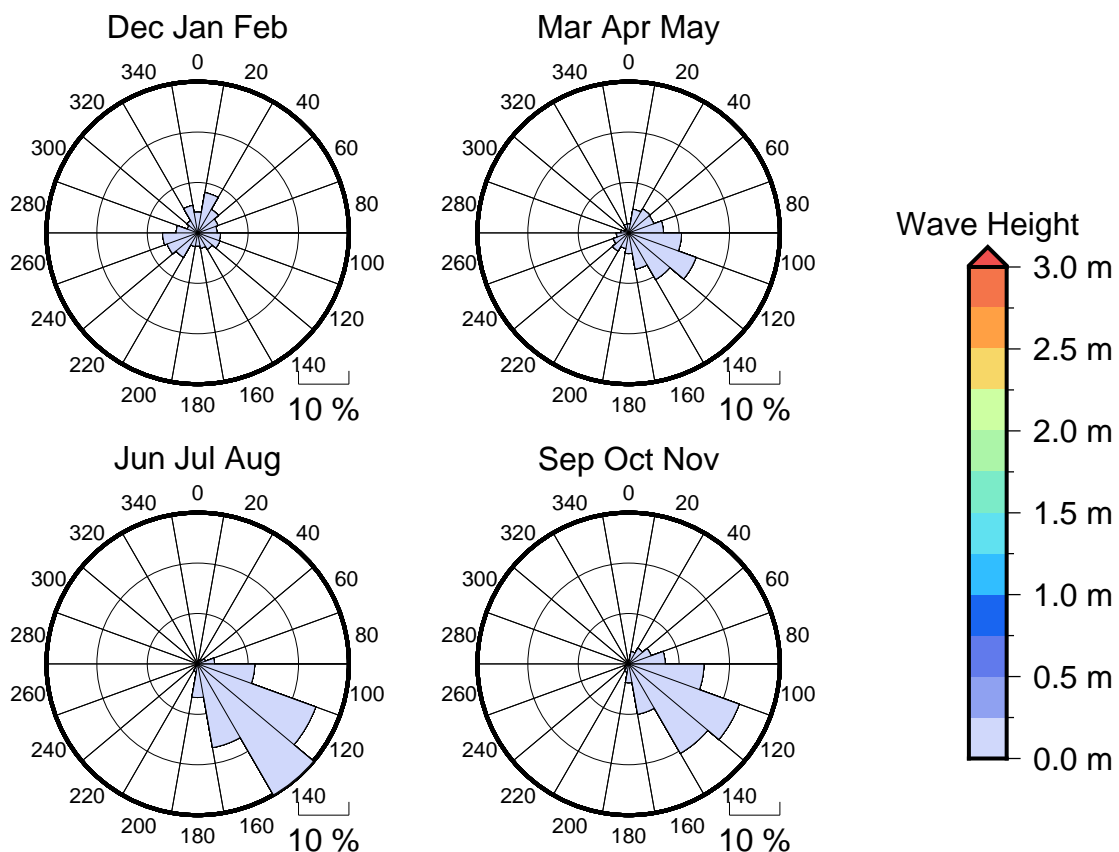
Figure 3 Seasonal wave roses for Samarai
