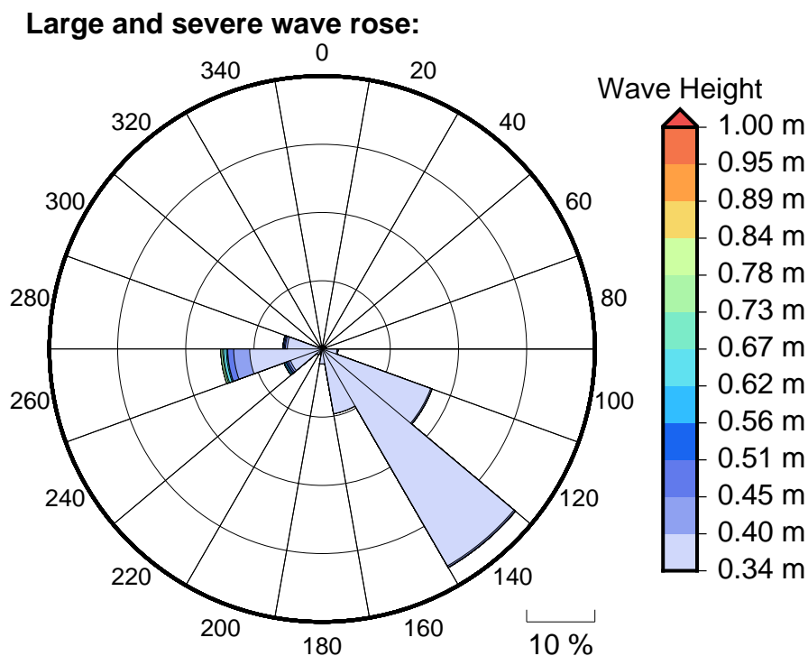
Figure 6 Large, severe and extreme wave roses for Samarai
