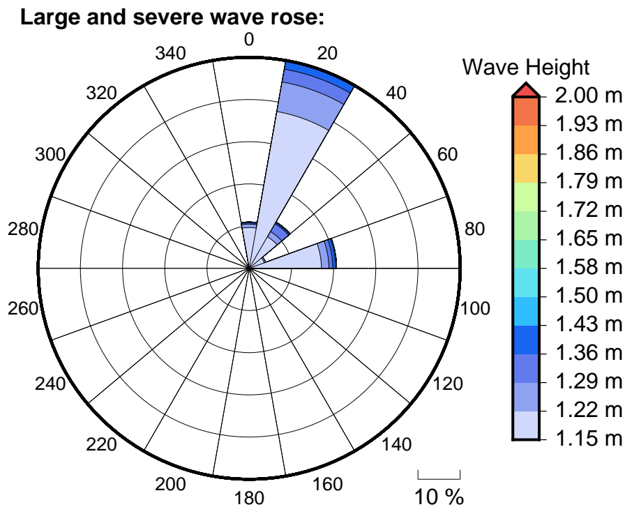
Figure 6 Large, severe and extreme wave roses for Wewak
