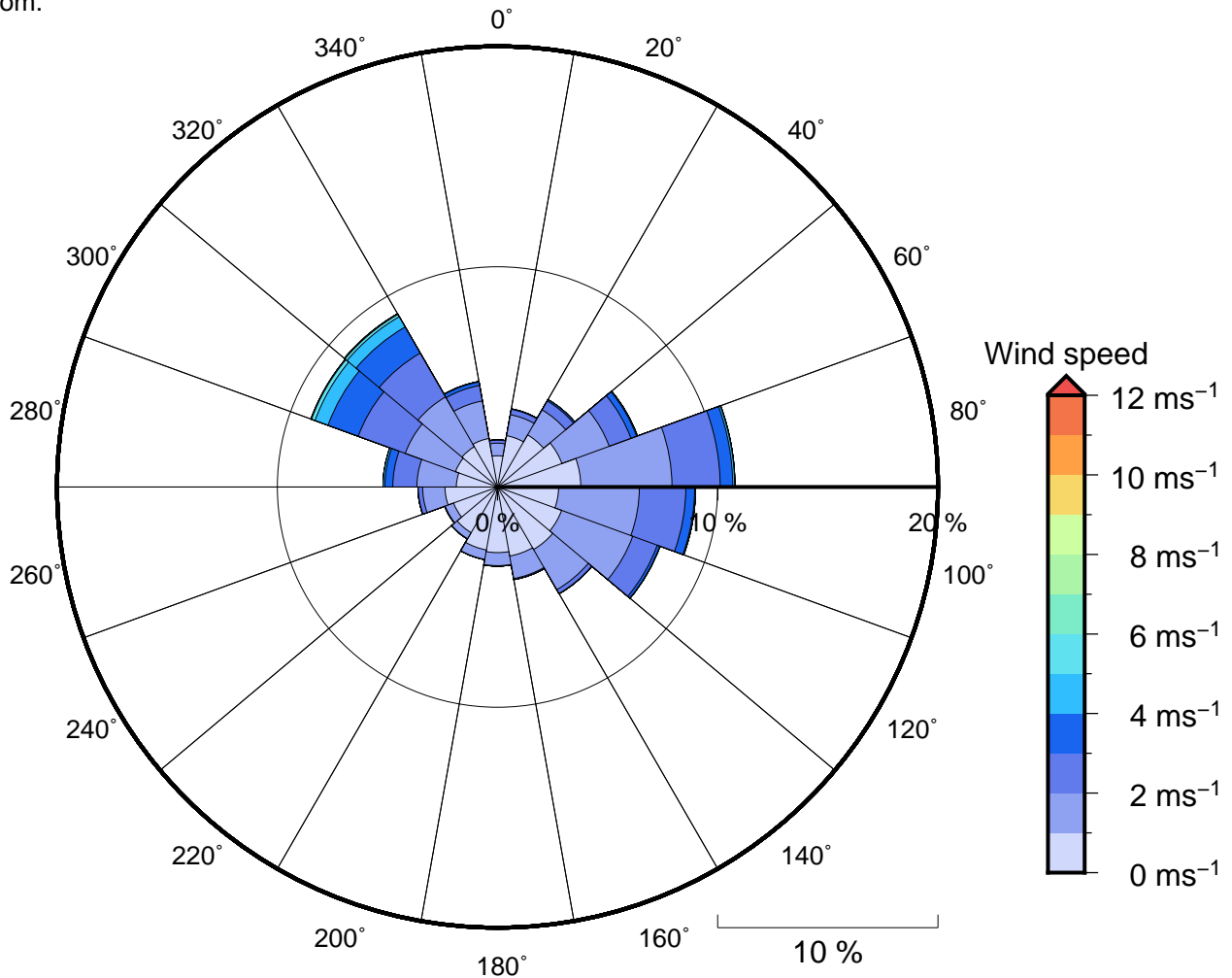
Figure 11 Annual wind rose for Wewak. Note that directions are where the wind is coming from .
