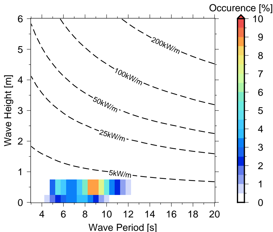
Figure 10 Occurrences of sea states in Wewak .
