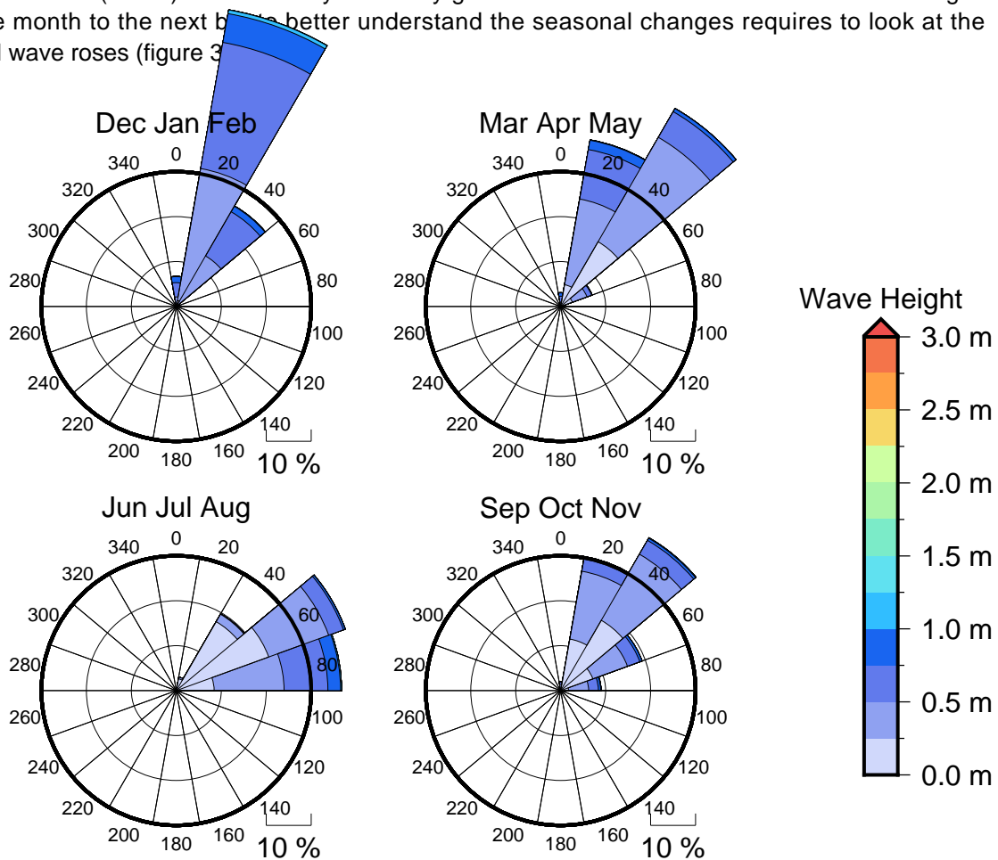
Figure 3 Seasonal wave roses for Wewak
