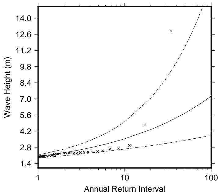
Figure 9 Extreme wave distribution for Koror. The crosses represents the wave events that occurred since 1979. The plain line is the statistical distribution that best fit the past wave events. The dotted line show the upper and lower high confidence of the fit, there is a 95% chance that the fitted distribution lie between the two dashed lines.
