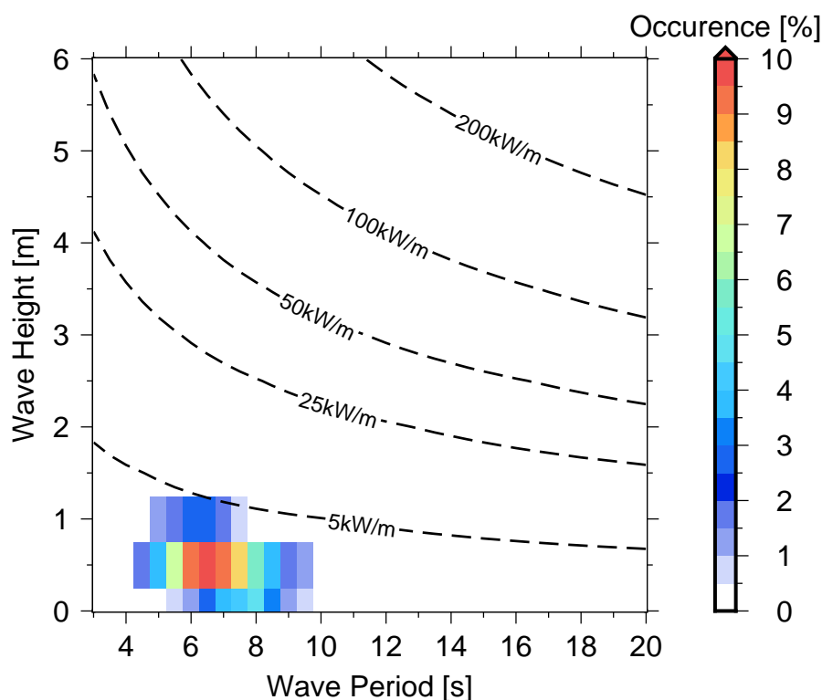
Figure 10 Occurrences of sea states in Koror .
