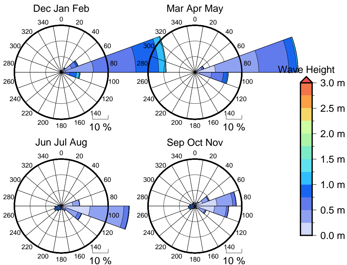
Figure 3 Seasonal wave roses for Koror
