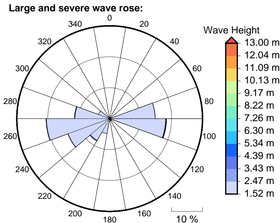
Figure 6 Large, severe and extreme wave roses for Koror
